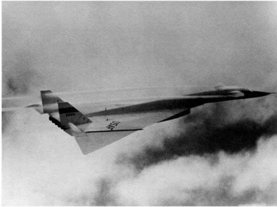
The North American XB-70 yielded valuable data on flight characteristics of large, supersonic aircraft. This photo of a test flight shows shock waves and vortices forming on the fuselage and wings.
