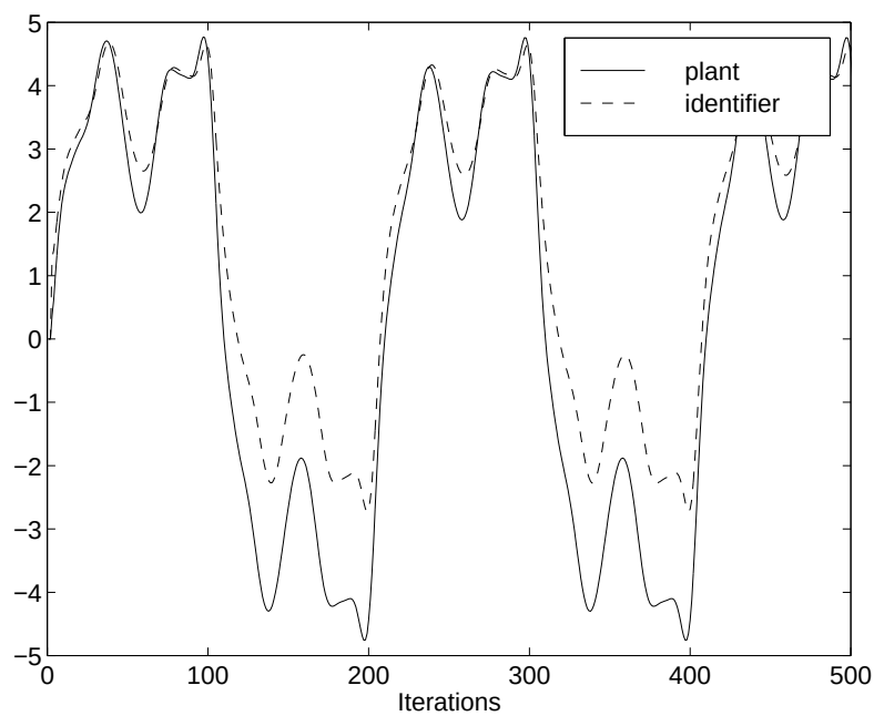
Figure 16.13: Plots of the outputs of the plant and its identifier during the testing phase in Example 16.4.
