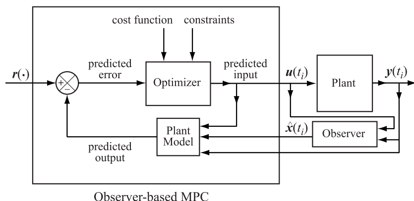
Figure 13.9: MPC implementation when the plant's state is not available.
