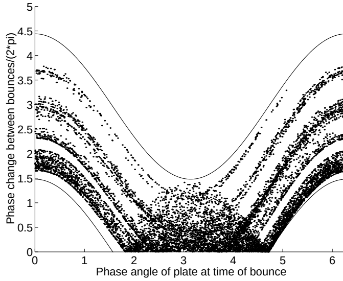
Figure 18.29: An orbit of the ball map.
