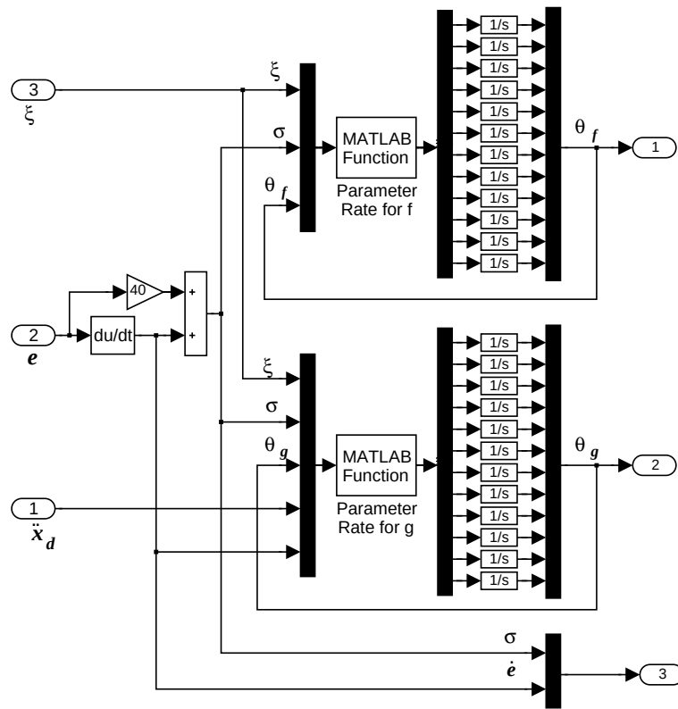
Figure 15.39: Parameter adaptation block of Example 15.12.
