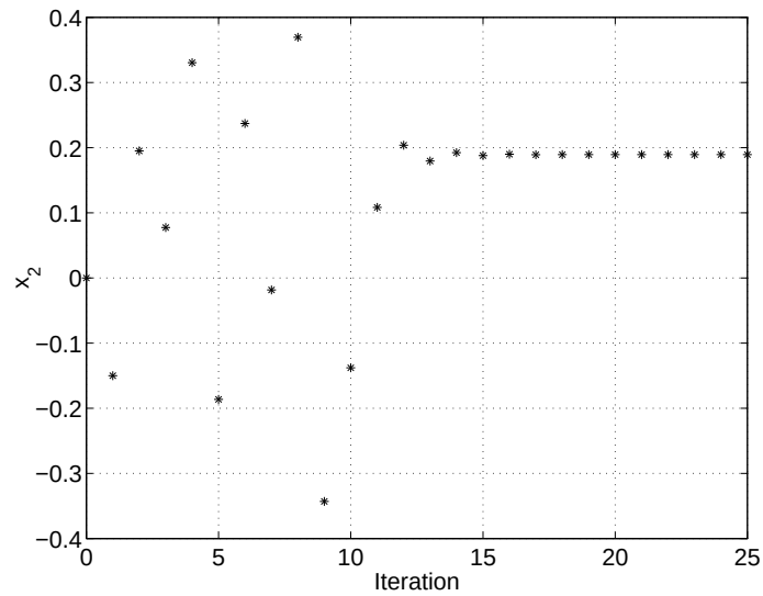
Figure 18.25: A plot of x_2 versus time for the controlled Hénon map of Example 18.5.
