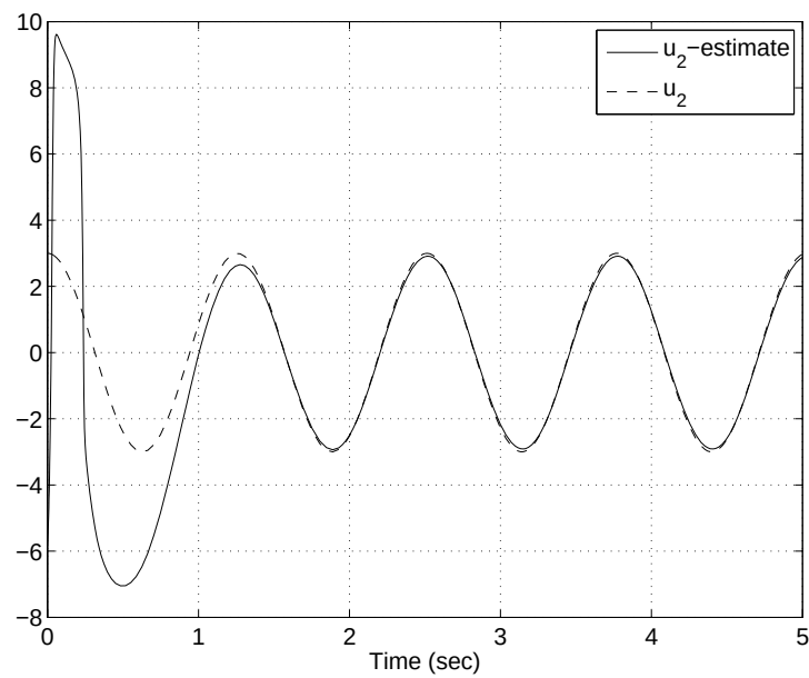
Figure 12.11: Plots of the unknown input and its estimate using the Edwards-Spurgeon UIO.
