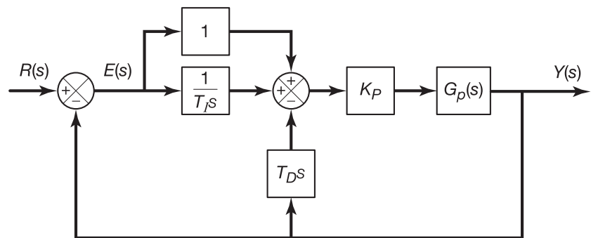
Figure 14.19: Type B PID controller.
