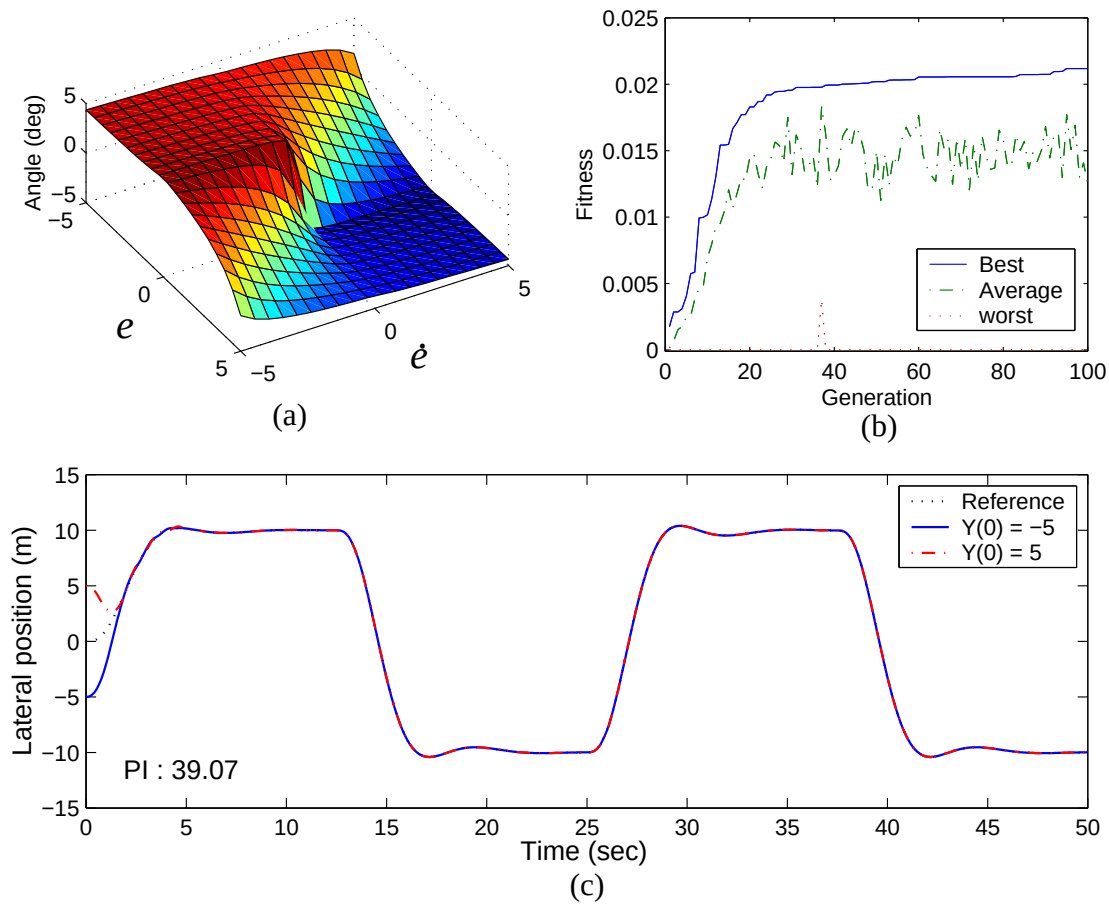
Figure 17.17: Summary of the simulation run of the closed-loop system driven by the fuzzy logic controller obtained from the fuzzy rule base shown in Figure 17.16: (a) control surface (b) fitness values of the best, average, and worst chromosomes (c) tracking performance.
