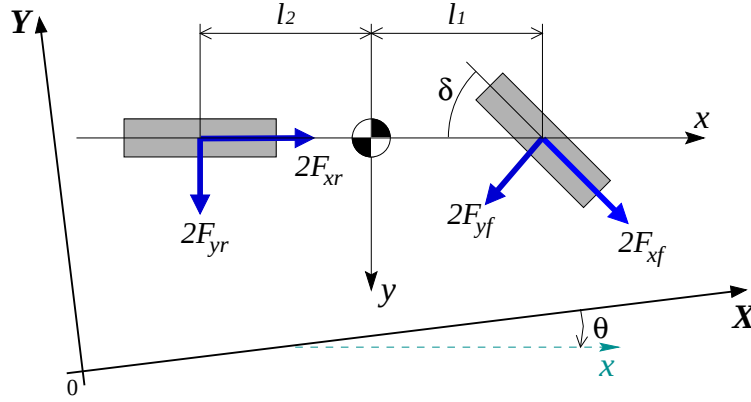
Figure 17.6: Schematic of a bicycle model of a front-wheel-steering vehicle.
