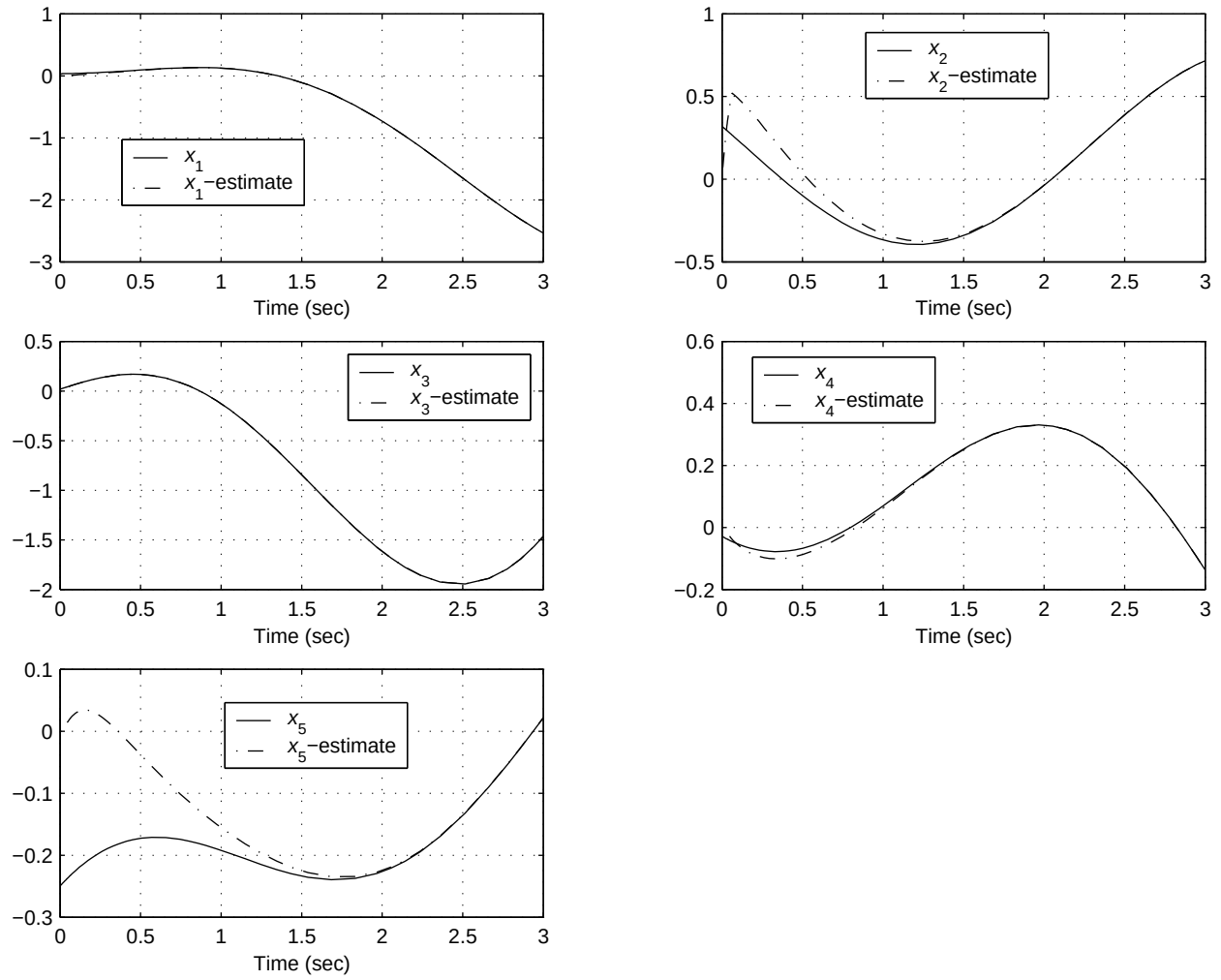
Figure 12.5: Plots of x_i s and their estimates versus time for Example 12.3.
