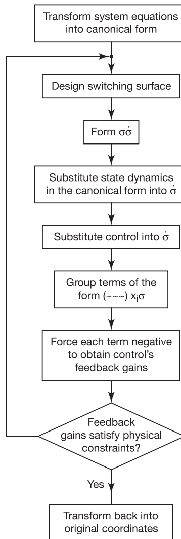
Figure 10.11: Summary of a single-input sliding mode controller design. Adapted from DeCarlo et al. [77].
