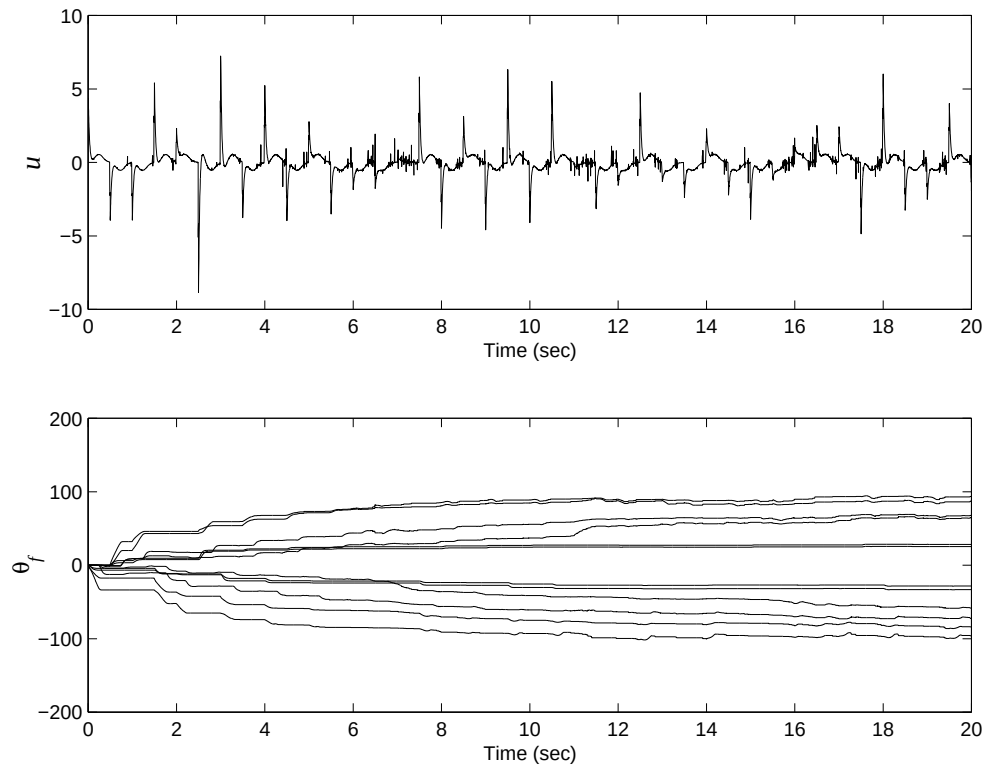
Figure 15.37: Plots of control effort u(t) and the components of the parameter vector \theta_f versus time in Example 15.11.
