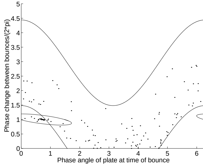
Figure 18.30: An orbit of the controlled modified ball map.
