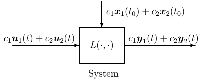
Figure 1.9: Illustration of the superposition property.
