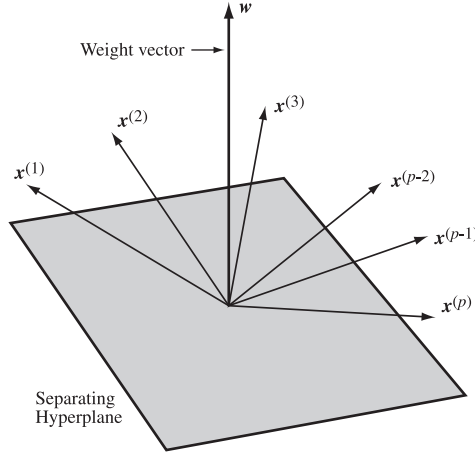
Figure 16.5: Linearly separable vectors after their preprocessing.
