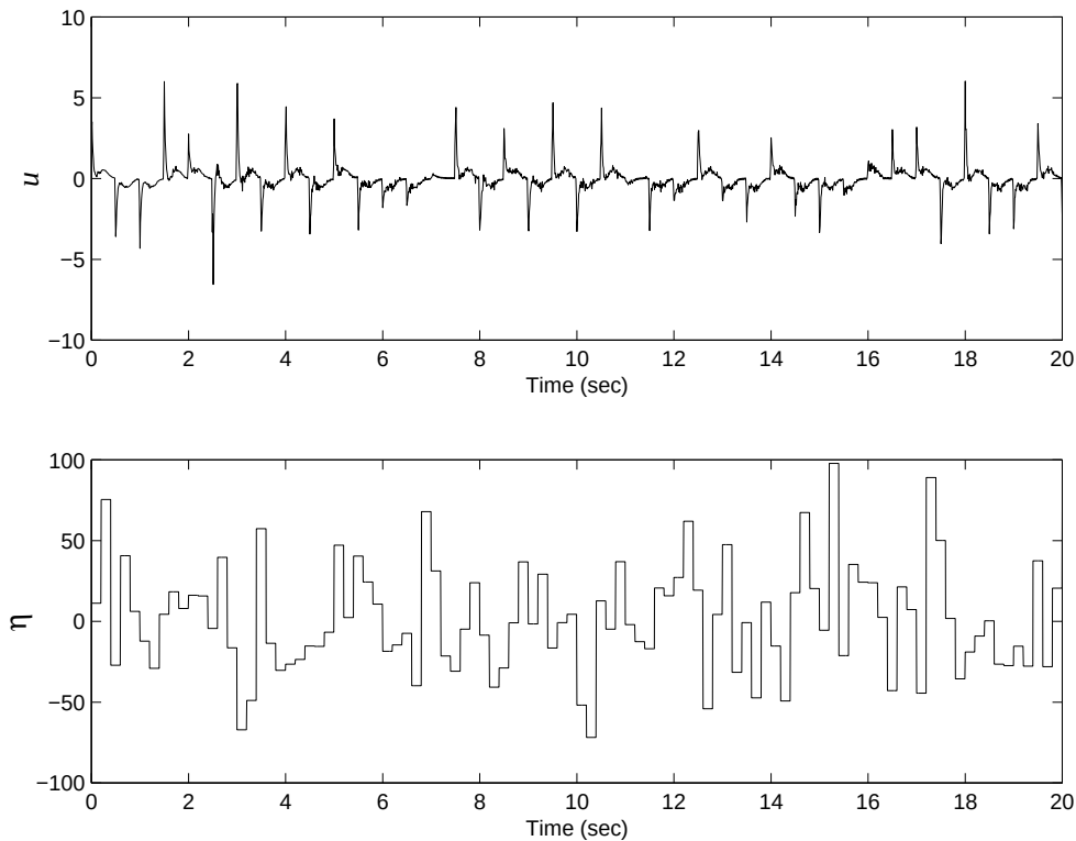
Figure 15.40: Plots of the control effort u(t) and disturbance \eta(t) versus time in Example 15.12.
