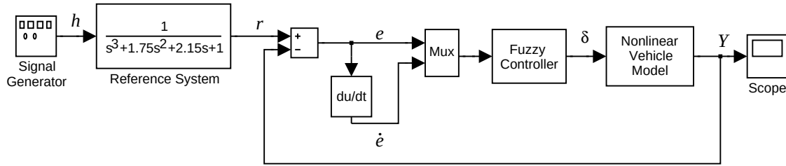
Figure 17.7: SIMULINK block diagram of the closed-loop vehicle system driven by a fuzzy logic controller.
