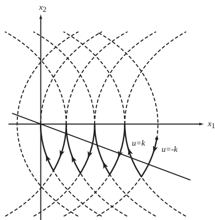
Figure 10.5: Chattering in a variable structure sliding mode system—a magnified view.
