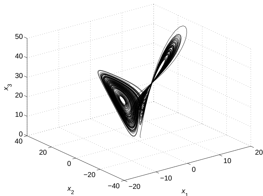
Figure 18.36: State-space trajectory of the transmitter (18.121).
