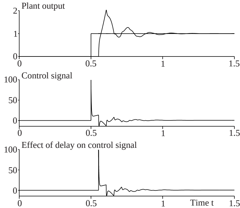
Figure 14.11: Step response of the PIDF-controlled first-order system with transportation delay in Example 14.4.
