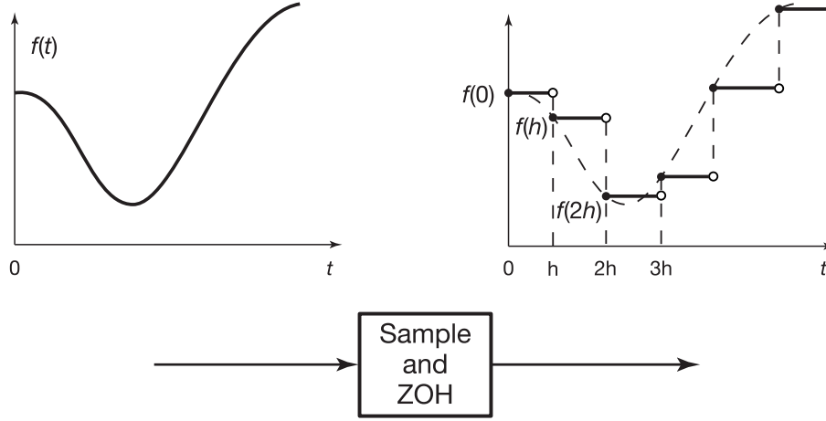
Figure 3.1: Sample and zero-order hold (ZOH) element operating on a continuous function.
