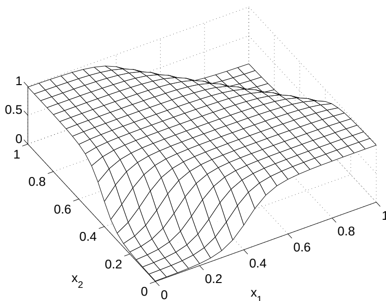
Figure 16.9: The function implemented by the trained neural network to solve the two-input XOR problem in Example 16.3.
