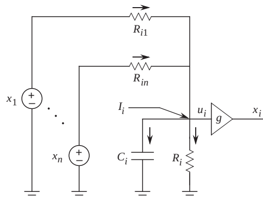
Figure 16.25: Equivalent representation of a single node in the circuit realization of the Hopfield neural network.
