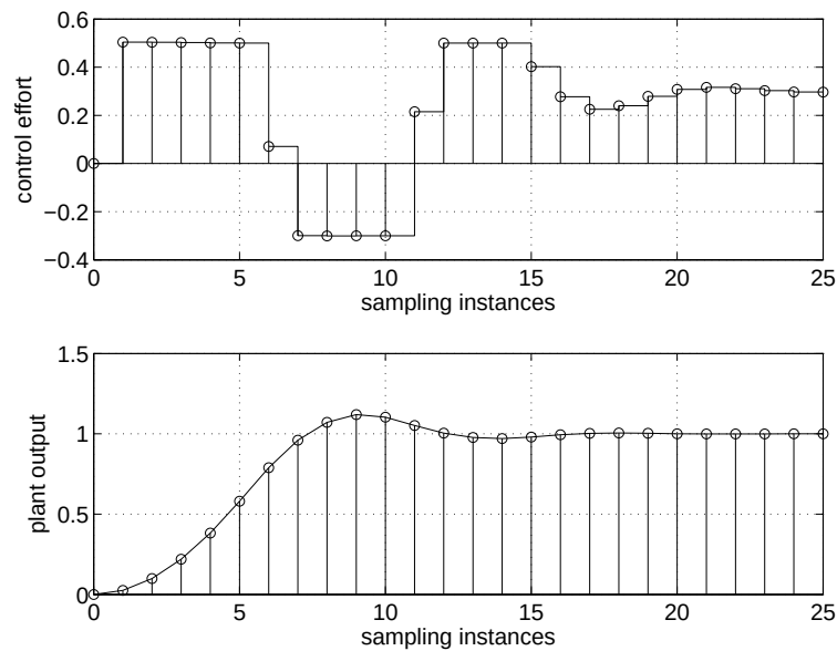
Figure 13.7: Plots of control effort and the plant's output versus time of the closed-loop system of Example 13.2 for the case when the constraints were imposed on all the components of \mathbf{U}[k] .
