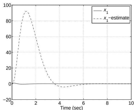
Figure 5.16: A plot of x_1 and its estimate versus time for the closed-loop system with the reduced-order observer, designed using method 2, in the loop.
