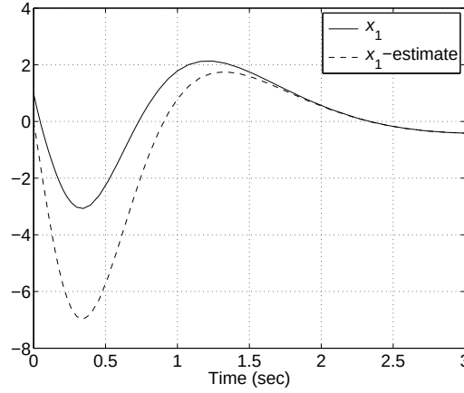
Figure 5.14: A plot of x_1 and its estimate versus time for the closed-loop system with the full-order observer in the loop.
