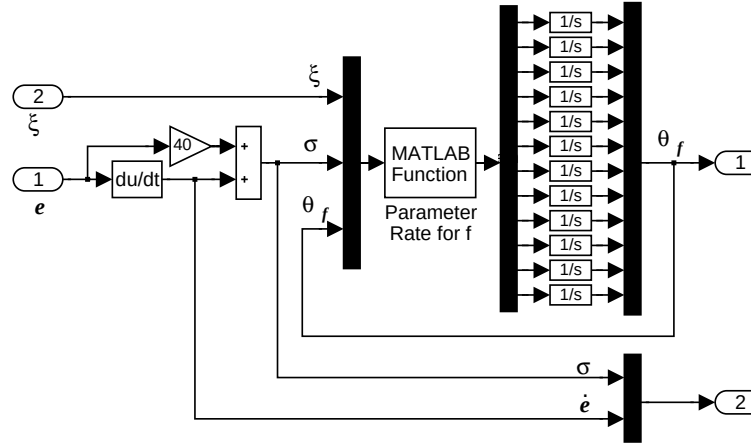
Figure 15.34: Parameter adaptation block of Example 15.11.
