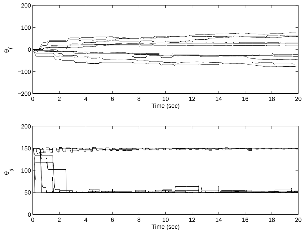
Figure 15.42: Plots of the components of the parameter vectors \theta_f and \theta_g versus time in Example 15.12
