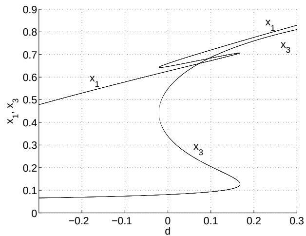
Figure 7.14: Plots of the equilibrium values of x_1 and x_3 versus d for u = 0 .
