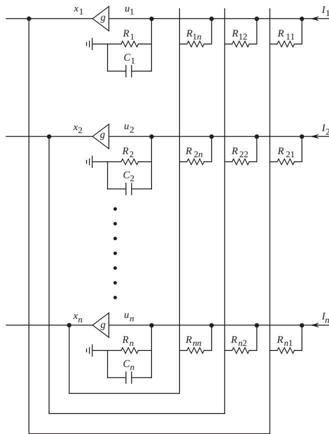
Figure 16.24: A circuit realization of the Hopfield neural network.
