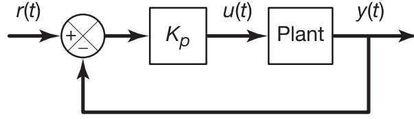
Figure 14.8: Experimental setup to determine the critical gain, K_{cr} and critical period of oscillation, P_{cr} .
