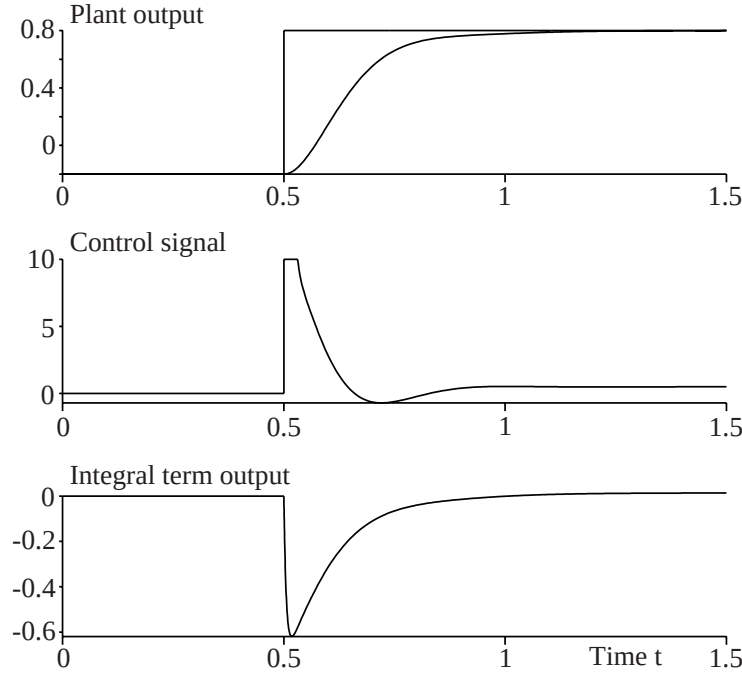
Figure 14.16: Plant output of the PIDF-controlled second-order plant with the integrator anti-windup circuit.
