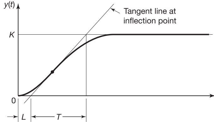
Figure 14.6: An S -shaped step response and its characterization using three parameters.
