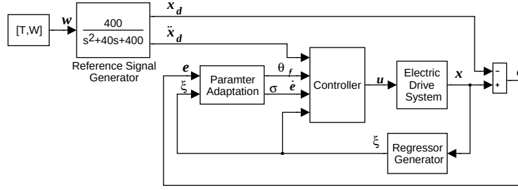
Figure 15.33: SIMULINK block diagram of fuzzy adaptive robust control system of Example 15.11.
