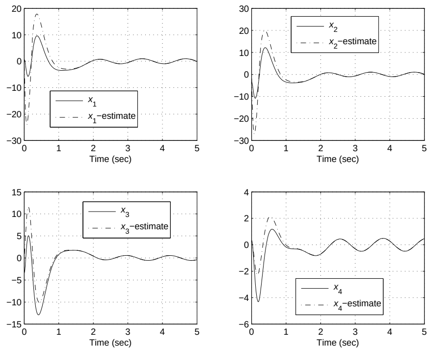
Figure 12.10: Plots of states and their estimates using the Edwards-Spurgeon UIO.
