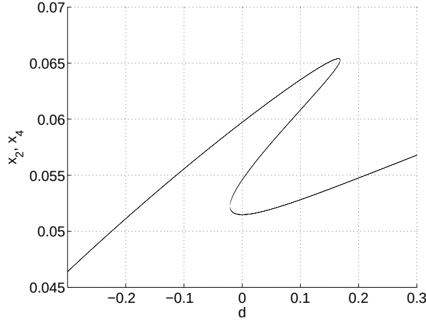
Figure 7.15: Plots of the equilibrium values of x_2 and x_4 versus d for u = 0 .
