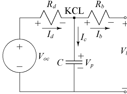
Figure 6.4: A battery model in the discharging mode of operation.
