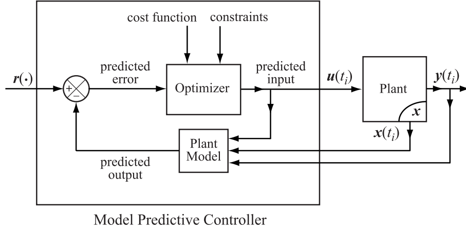
Figure 13.3: State feedback model predictive controller.
