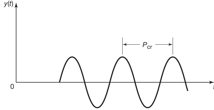
Figure 14.9: Measuring the period of the sustained oscillation, P_{cr} .
