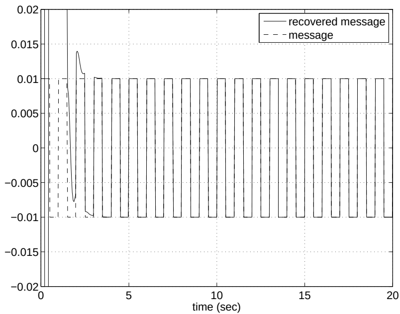
Figure 18.35: Plots of the message signal, m , and its recovered version at the receiver's end obtained from the difference, y - \tilde{y} ; see (18.124).
