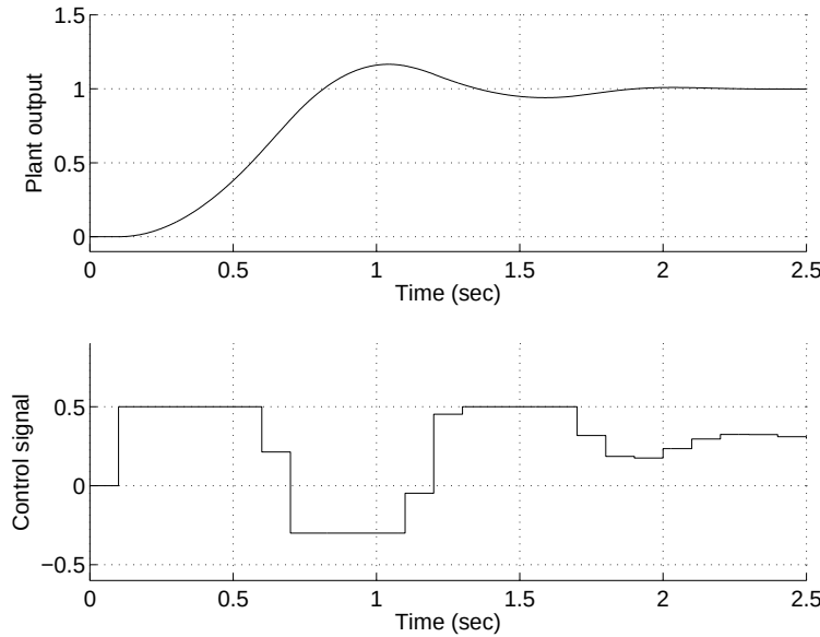
Figure 13.8: Plots of control effort and the plant’s output versus time of the closed-loop system of Example 13.3 for the case when the constraints were imposed only on the first component of \mathbf{U}(k) .
