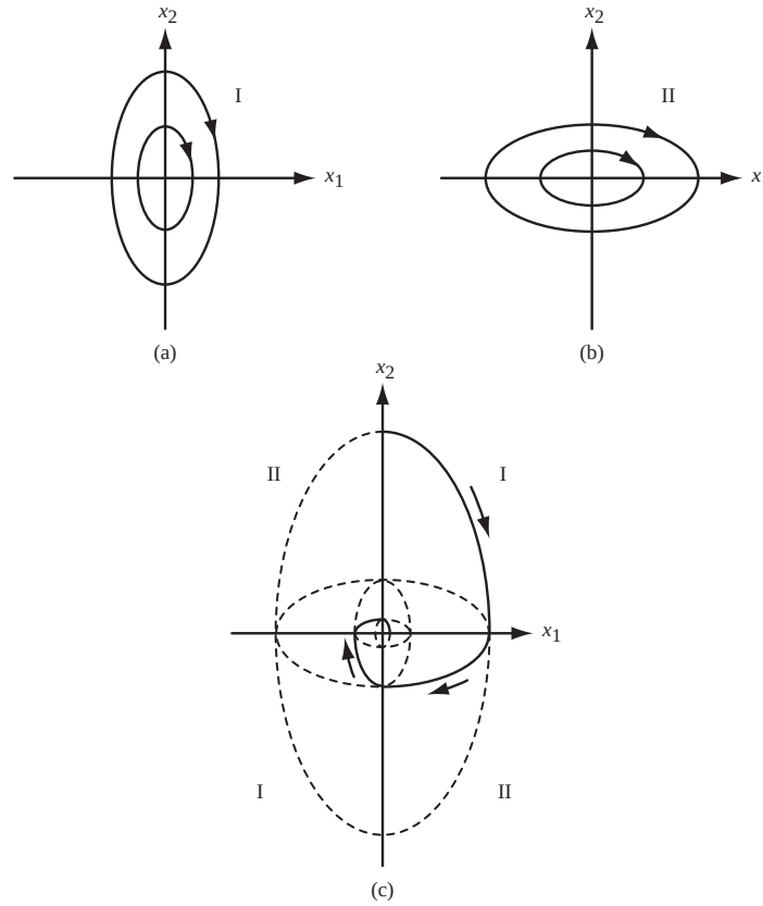
Figure 10.1: Figures (a) and (b) are phase-plane portraits of structures making up a variable structure system and Figure (c) is a phase-plane portrait of the variable structure system itself, where the structure of the system is changed any time the system's trajectory crosses either of the coordinate axis. This figure was adapted from the survey paper by Utkin [331].
