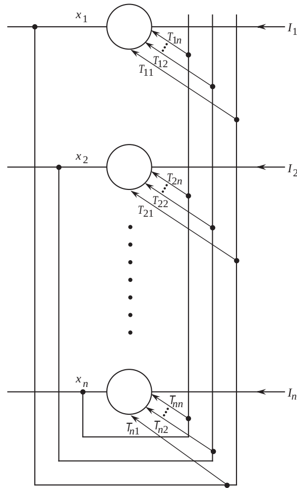
Figure 16.22: Hopfield neural network model.
