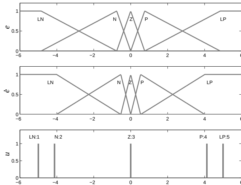
Figure 17.12: Input and output fuzzy membership functions of the best FLC of the 50-th generation obtained by tuning fuzzy membership functions.
