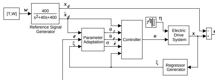
Figure 15.38: SIMULINK block diagram of the fuzzy adaptive robust control system of Example 15.12.
