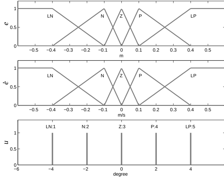
Figure 17.8: Fuzzy membership functions for e , \dot{e} , and u .
