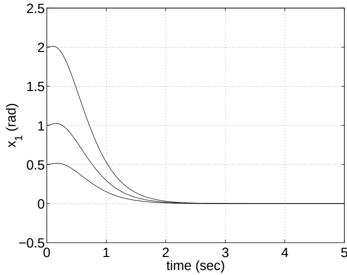
Figure 11.1: Plots of the one-link manipulator's link angle, x_1 = \theta , versus time for three different initial angles \theta(0) . The manipulator is driven by the state-feedback control law (11.50).
