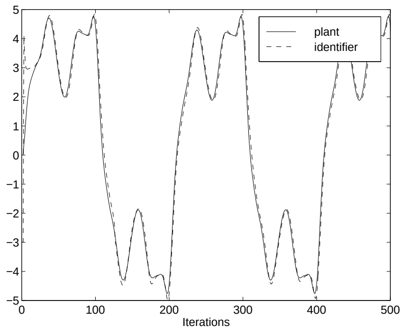
Figure 16.12: Plots of the outputs of the plant and its identifier during the learning phase in Example 16.4.
