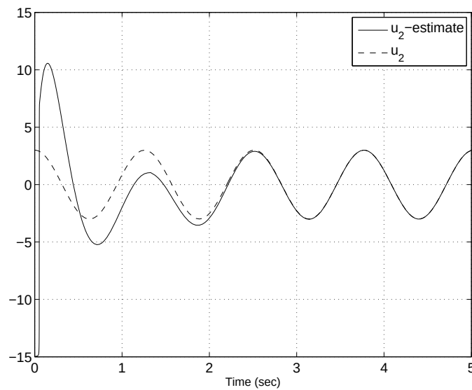
Figure 12.8: Plots of the unknown input and its estimate.
