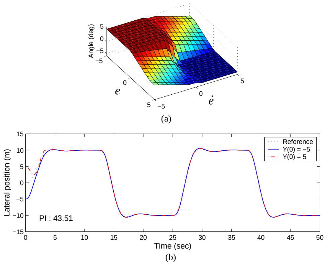
Figure 17.13: The best FLC of the 50-th generation obtained by tuning fuzzy membership functions: (a) control surface (b) tracking performance.
