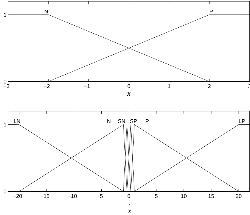
Figure 15.32: Fuzzy sets for x and \dot{x} .
