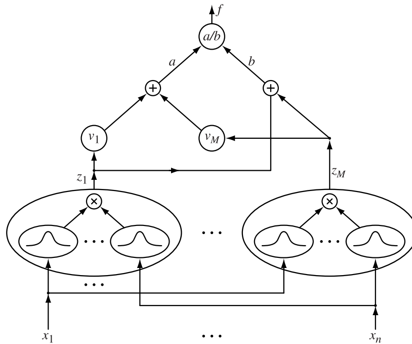
Figure 16.10: Fuzzy logic system (16.27) represented as a feedforward network.
