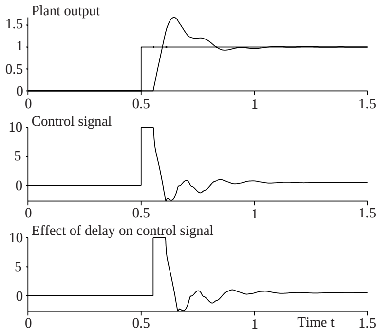
Figure 14.14: Plant output of the PIDF-controlled first-order plant with with transportation delay and constraints on input.
