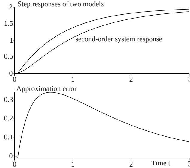
Figure 14.7: Comparison of step responses of the second-order system and its approximation using a first-order system with transportation delay in Example 14.3.
