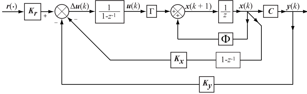
Figure 13.4: Discrete-time MPC for linear time-invariant systems.
