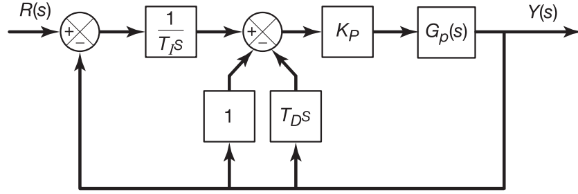
Figure 14.20: Type C PID controller.
