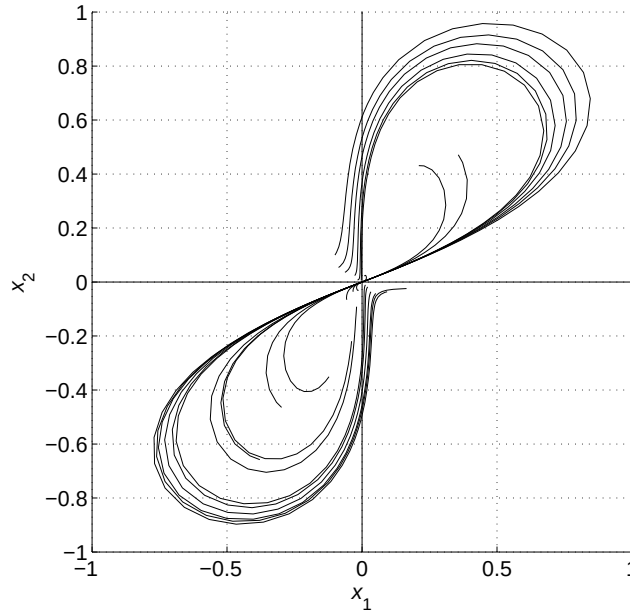
Figure 7.2: A phase portrait of system (7.2) where the origin is attractive but not asymptotically stable.
