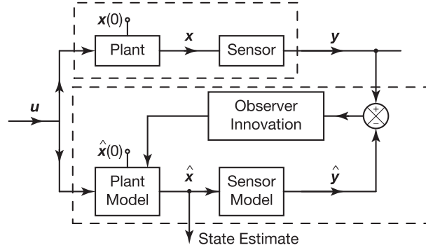
Figure 5.5: General observer architecture.
