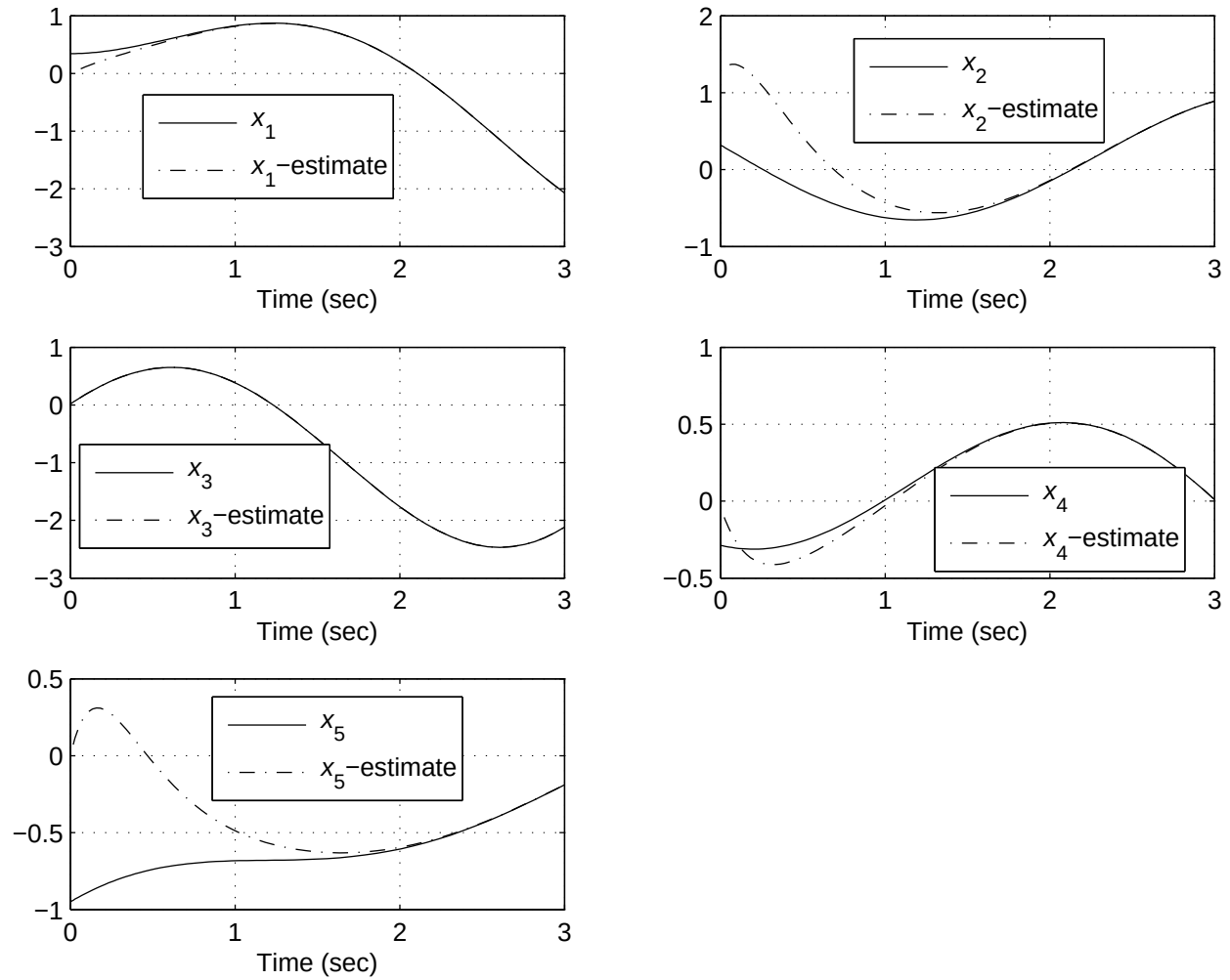
Figure 12.3: Plots of x_i s and their estimates versus time for Example 12.2.
