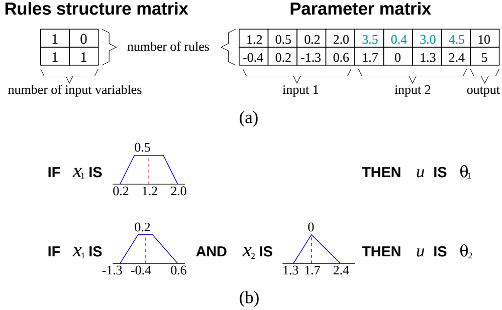
Figure 17.15: An example of a chromosome structure and its corresponding fuzzy rule base where the controller has two inputs, x_1 and x_2 , and one output u .
