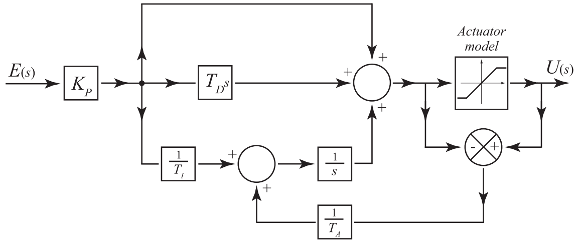
Figure 14.15: A type A PID controller with the integrator anti-windup.
