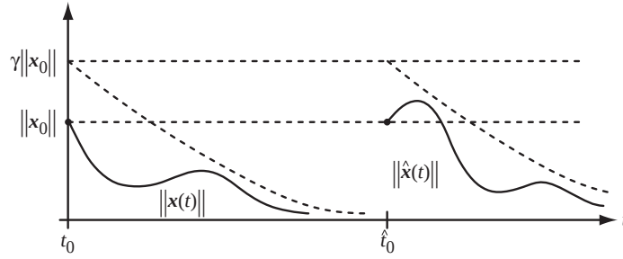
Figure 7.3: Illustration of uniform exponential stability: a decaying-exponential bound is independent of the initial time t_0 .
