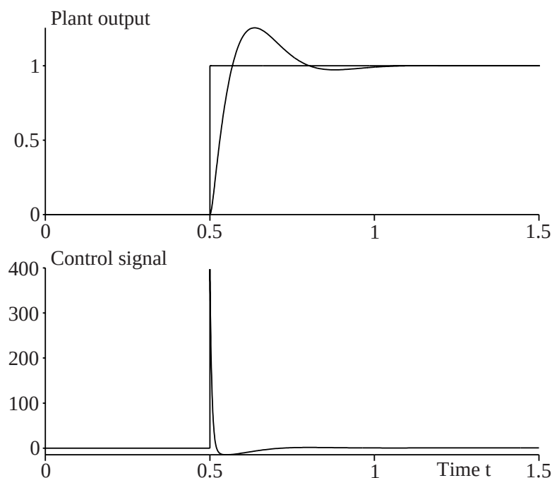
Figure 14.12: Step response of the closed-loop system with re-tuned PIDF controller and second-order plant in Example 14.4.
