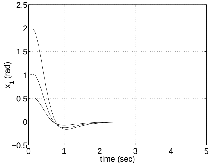
Figure 11.2: Plots of the one-link manipulator's link angle, x_1 = \theta , versus time for three different initial angles \theta(0) . The manipulator is driven by the combined controller-estimator compensator.
