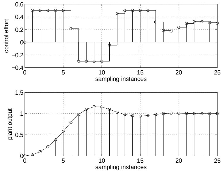
Figure 13.6: Plots of control effort and the plant's output versus time of the closed-loop system of Example 13.2 for the case when the constraint was imposed only on the first component of \mathbf{U}[k] .
