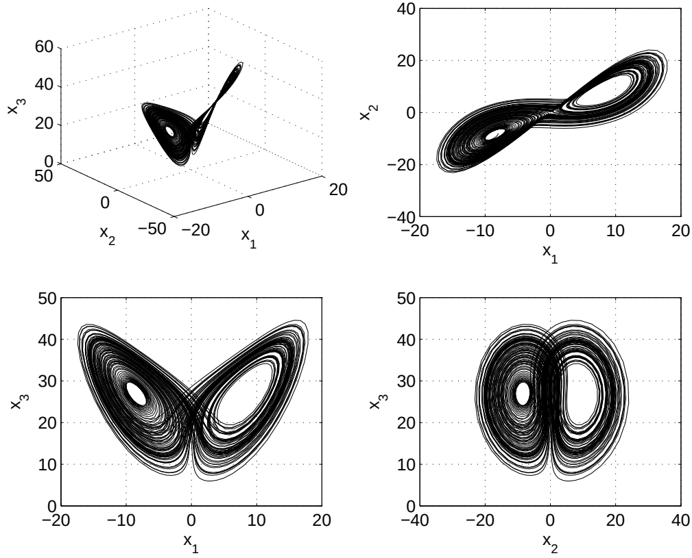
Figure 18.33: Plots of trajectories of the fuzzy Lorentz system (18.121).
