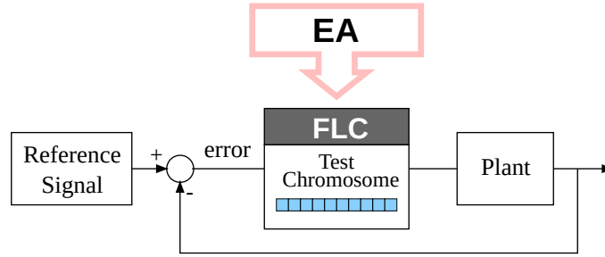
Figure 17.5: A configuration used to design a fuzzy logic controller using an evolutionary algorithm.
