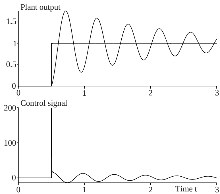
Figure 14.10: PIDF-controlled second-order system's step response of Example 14.4, where the reference input is a step function delayed by 0.5 s in order to better observe the set-point kick phenomenon.
