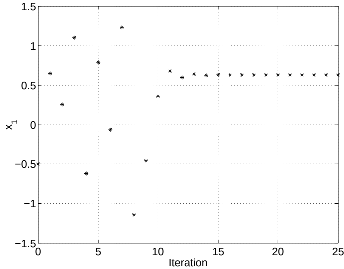
Figure 18.24: A plot of x_1 versus time for the controlled Hénon map of Example 18.5.
