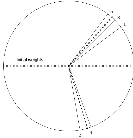
Figure 16.21: Training patterns, initial weights and the final weights of the WTA network of Example 16.8.
