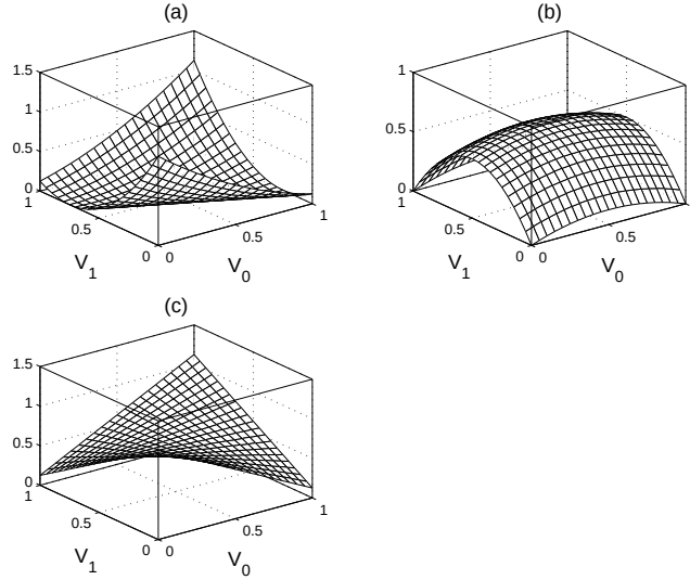
Figure 16.27: Constructing the cost function for a 2-bit A/D converter—plots of the cost function and its components; (a) plot of (16.96) for an analog input of x = 1.5 ; (b) plot of the term used to cancel the quadratic terms in (16.96); (c) plot of the cost function (16.98).
