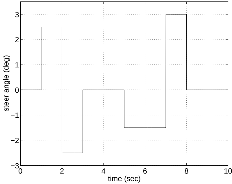
Figure 9.30: Plot of the steer angle \delta_f versus time for Exercise 9.22.
