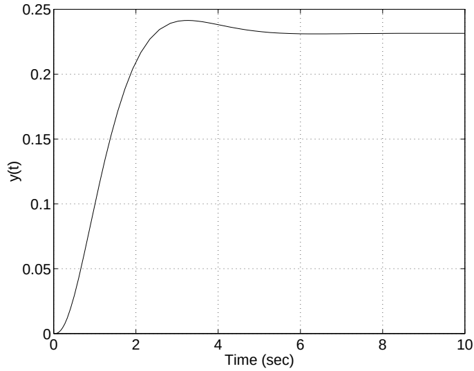
Figure 5.13: Step response of the closed-loop DC motor system with state feedback.
