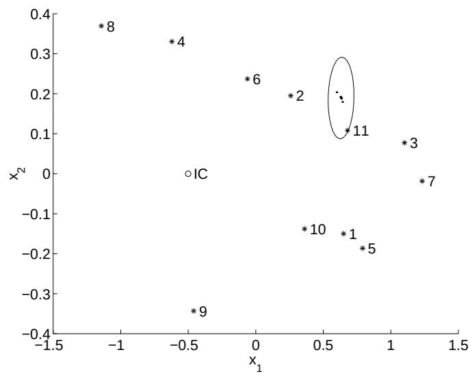
Figure 18.26: An orbit of the controlled Hénon map of Example 18.5, where the initial condition is denoted by “ \circ ” and labelled “IC”. The subsequent iterations prior to hitting the controllable target are denoted by “ \star ”. The iterations in the controllable target are denoted by “ \cdot ”.
