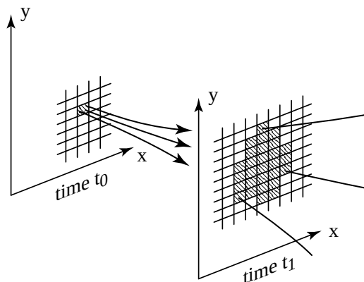
Figure 18.1: An illustration of the growth of uncertainty in a chaotic dynamical system.
