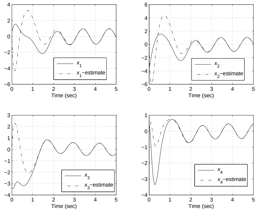
Figure 12.7: Plots of the states and their estimates.
