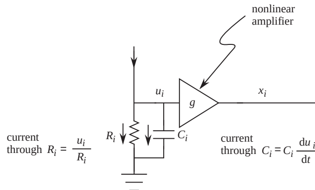
Figure 16.23: Model of a neuron in the Hopfield neural network.
