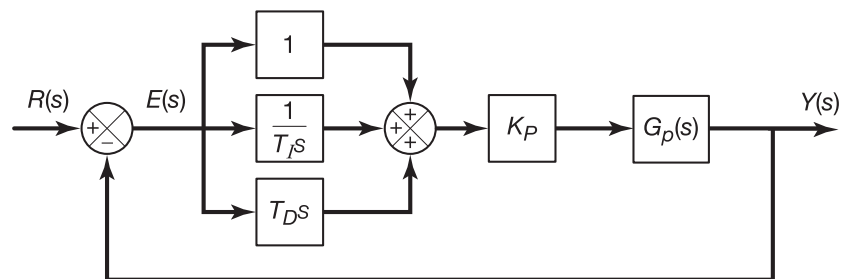
Figure 14.18: More detailed view of the type A PID controller.
