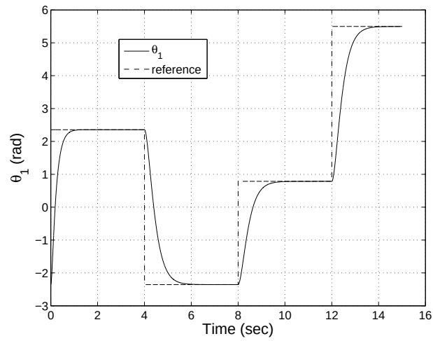
Figure 10.12: A plot of \theta_1 and its reference versus time.
