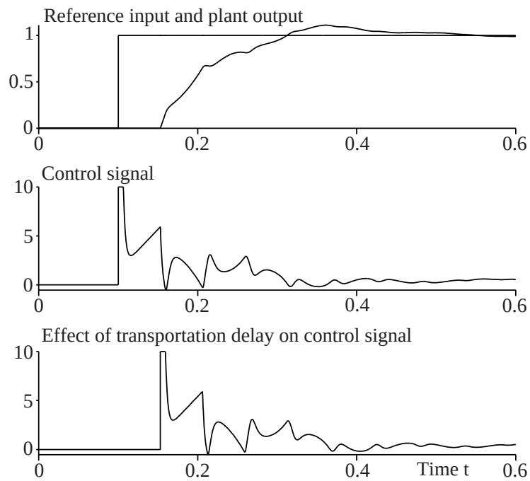
Figure 14.17: Plant output of the PIDF-controlled first-order plant with transportation delay and the integrator anti-windup.
