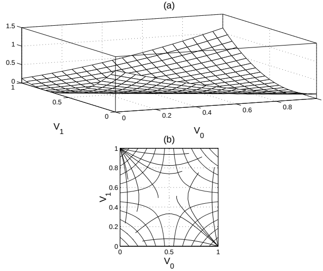
Figure 16.28: A plot of the cost function and a phase portrait of the 2-bit A/D converter for the analog value x = 1.5 .
