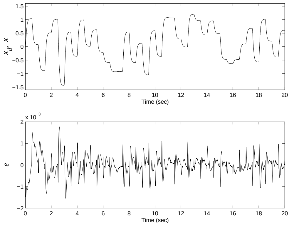
Figure 15.41: Plots of x(t) and error e(t) versus time in Example 15.12.
