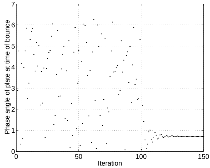
Figure 18.31: A plot of \phi(k) versus time of the controlled modified ball map.
