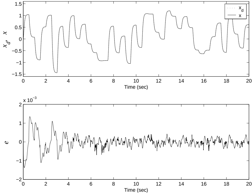
Figure 15.36: Plots of x(t) and error e(t) in Example 15.11.
