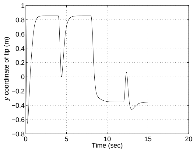
Figure 10.15: A plot of the y -coordinate of the end effector versus time.
