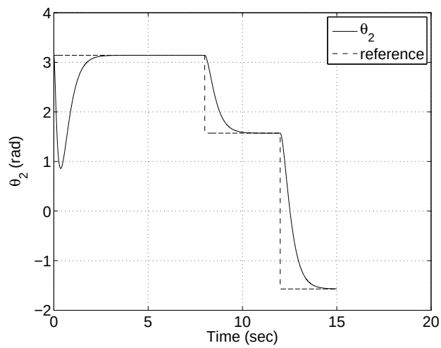
Figure 10.13: A plot of \theta_2 and its reference versus time.
