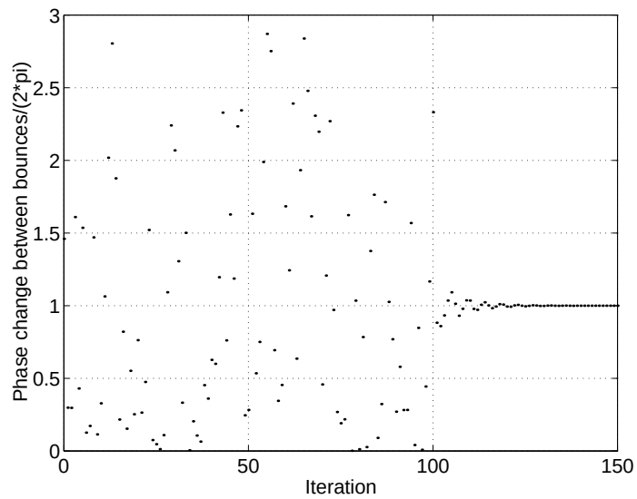
Figure 18.32: A plot of \psi(k) versus time of the controlled modified ball map.
