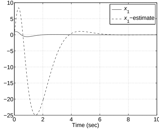
Figure 5.15: A plot of x_1 and its estimate versus time for the closed-loop system with the reduced-order observer, designed using method 1, in the loop.
