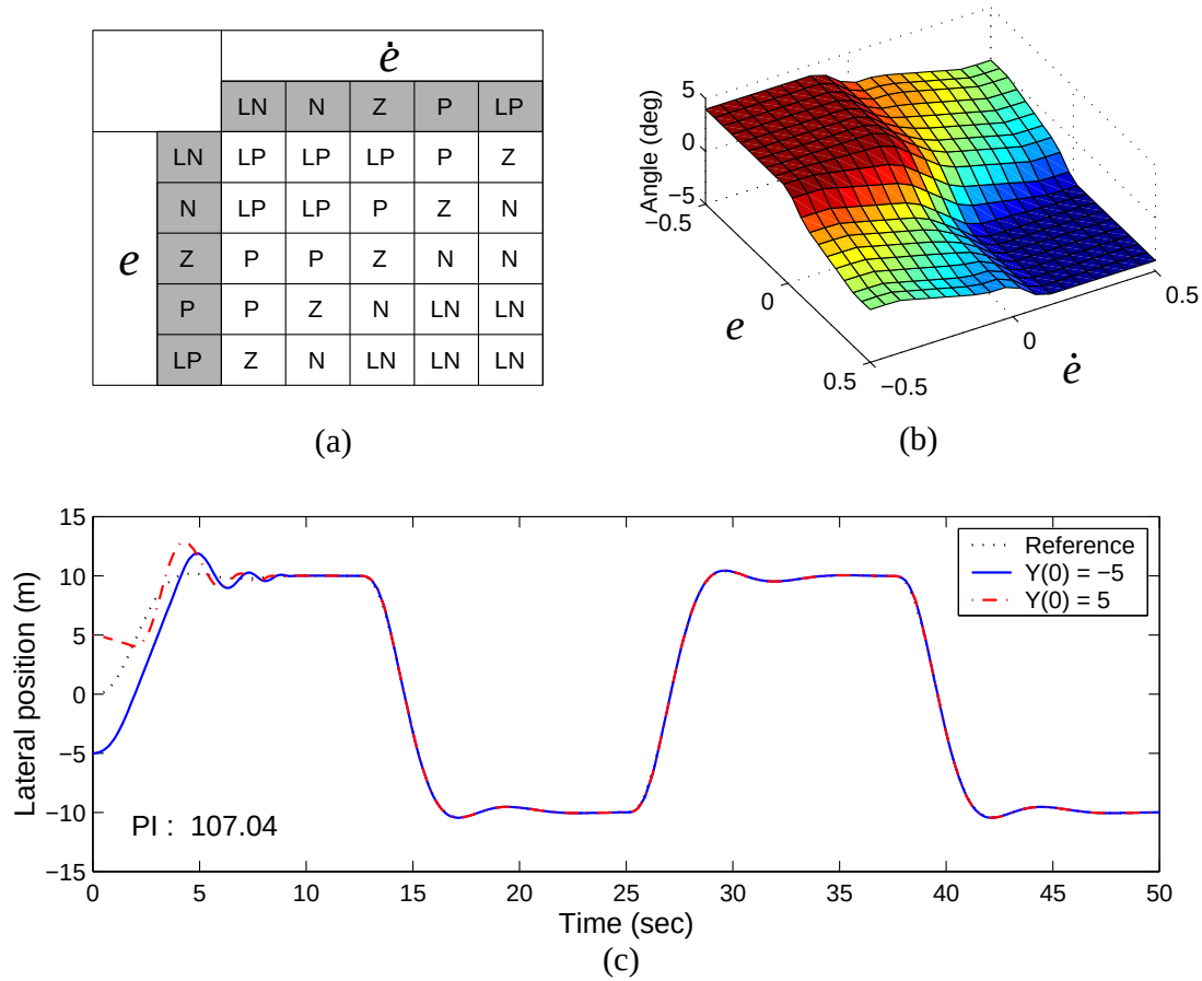
Figure 17.9: FLC constructed using a fuzzy rule base obtained heuristically: (a) fuzzy rules table (b) control surface (c) tracking performance.
