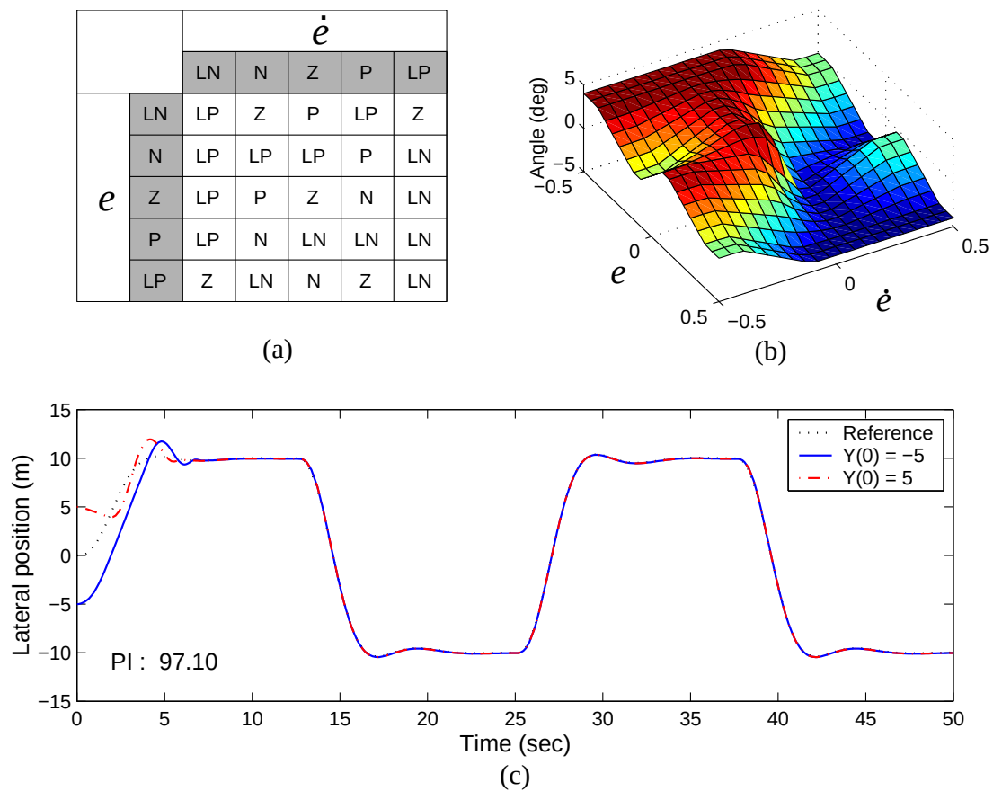
Figure 17.11: The best FLC of the 50-th generation using a fuzzy rule base automatically generated by the EA: (a) fuzzy rules table (b) control surface (c) tracking performance.
