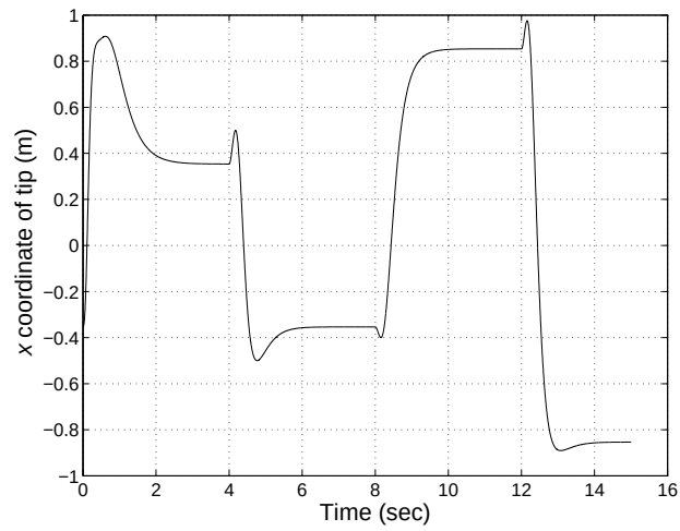
Figure 10.14: A plot of the x -coordinate of the end effector versus time.
