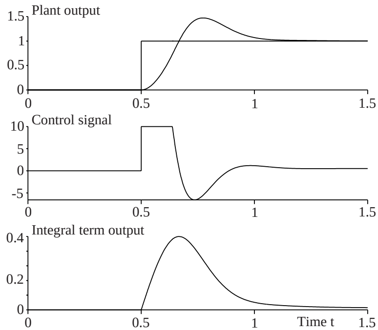
Figure 14.13: A PIDF-controlled second-order plant with with constrained actuator.
