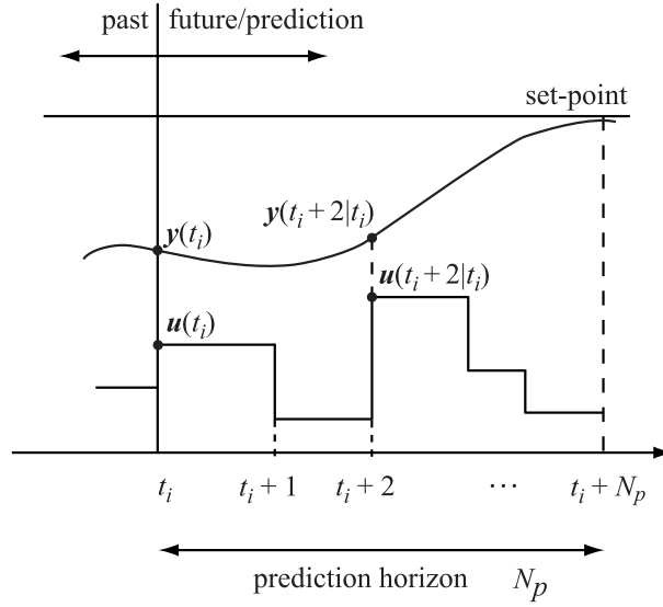
Figure 13.2: Controller action construction using model-based predictive control (MPC) approach.
