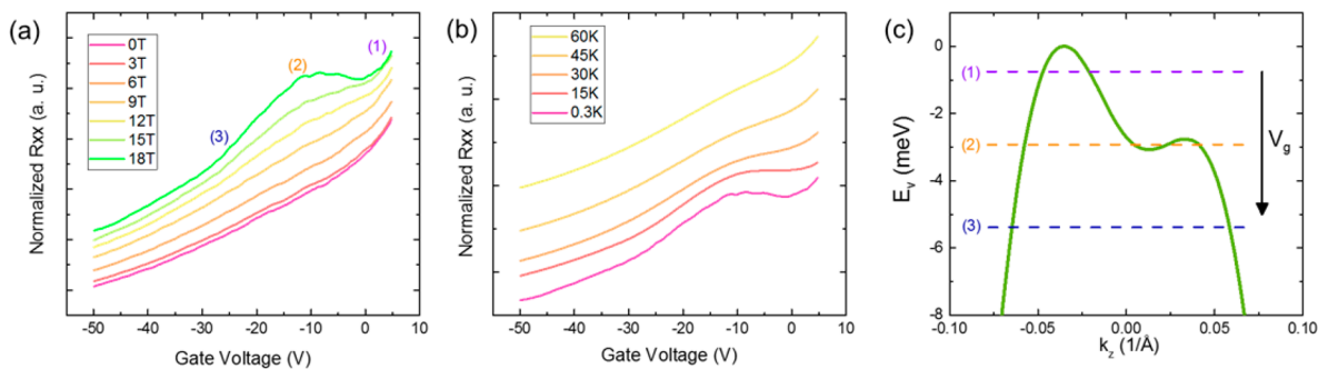
Figure 5. Anomalous increase in R_{xx} when sweeping gate voltage toward negative bias. The abnormal increase measured under different (a) magnetic field and (b) different temperature. (c) Explanation of the abnormal increase of resistance. As we sweep gate in the reverse direction, the Fermi energy will be pulled downward and slightly enter the valence band. (1), (2), and (3) represent three typical scenarios corresponding to the points with the same notations in panel a.
