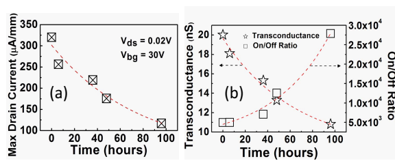
Fig. 3. (a) Maximum drain current. (b) Peak transconductance and ON/OFF ratio as a function of time exposed in ambient air at V_{ds} = 0.02 V.
