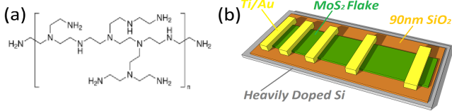
Fig. 1. (a) Molecular structure of PEI. (b) Geometry of MoS 2 FETs TLM structure with channel length of 500 nm, 1, 2, and 3 \mu\text{m} .
