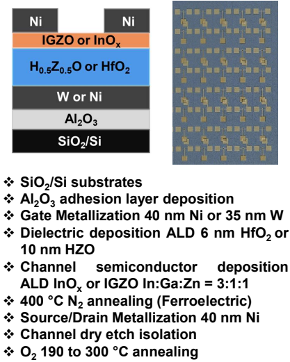
FIGURE 2. Device schematic, image, and fabrication flow of ALD InOx-based FETs and FeFETs.
