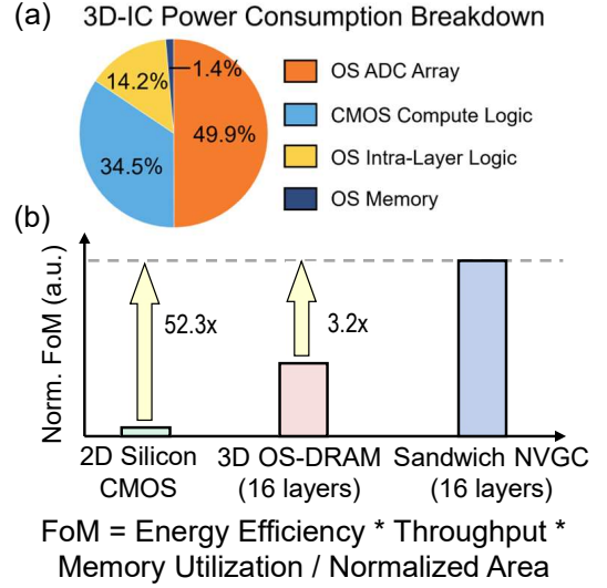
FIGURE 10. (a) 3D-IC cross-tier power breakdown. (b) FoM comparison among 2D silicon CMOS, 3D OS-DRAM, and this work.
