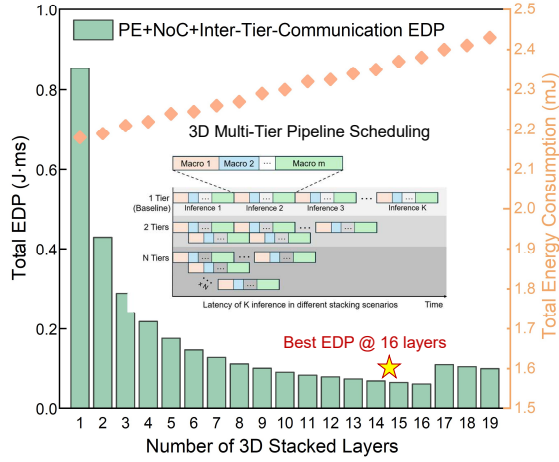
FIGURE 9. 3D stacking design exploration considering CMOS resources, NoC, and inter-tier communication with cross-tier pipelining, showing best performance with 16 layers.
