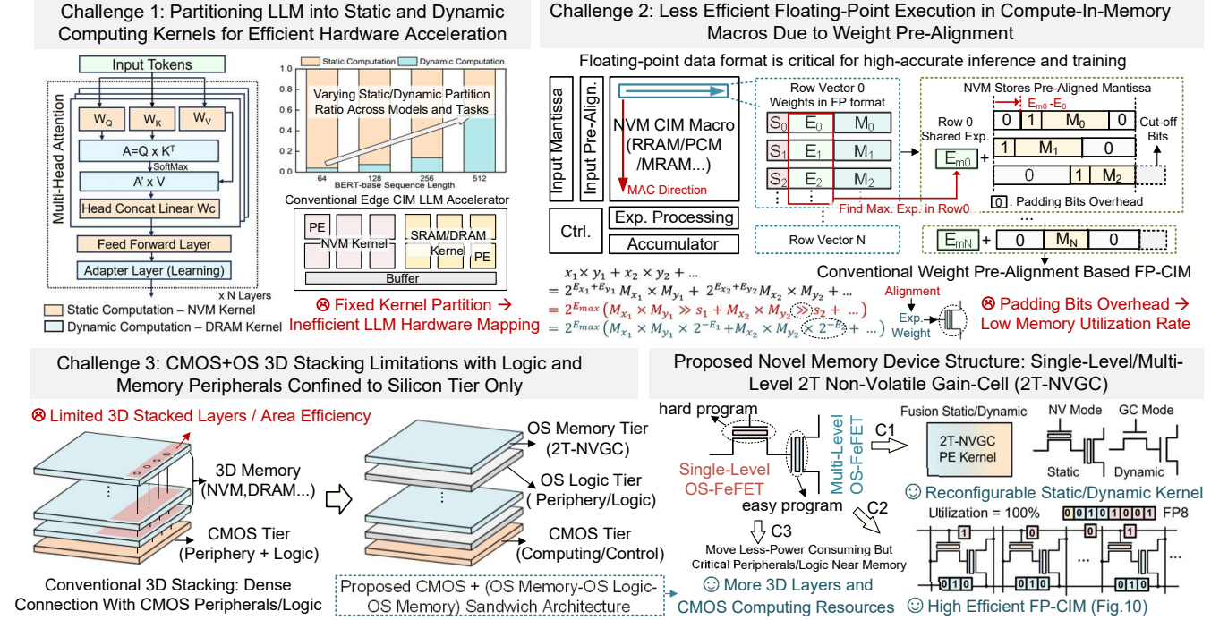
FIGURE 1. Key challenges in LLM accelerators, and our full-stack co-design solution harnessing OS technologies.
