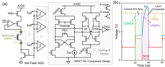
FIGURE 5. Analog circuit design with InOx transistors. (a) NMOS-only 3-bit flash ADC incorporating E-mode and D-mode OSFETs, with eight comparators that also function as sense amplifiers. (b) Simulated waveform of a two-stage current sense amplifier using a custom Verilog-A model with measured characteristics of fabricated OSFETs.
