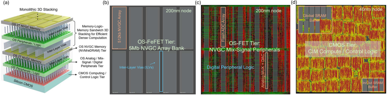
FIGURE 7. (a) Illustration of 3D NVGC accelerator featuring OS memory/OS logic/OS memory sandwich tiers on silicon CMOS. (b) OS-FeFET tier: 5 Mb NVGC array bank, composed of 512 Kb sub-arrays, connected to the OS logic tier through inter-layer vias. (c) OS-FET tier: analog components (such as DACs, flash ADCs) with digital peripherals and essential functional logic. (d) CMOS tier: CIM auxiliary and control logic for upper tiers, system scheduler, global buffer and input/output SRAM buffer.
