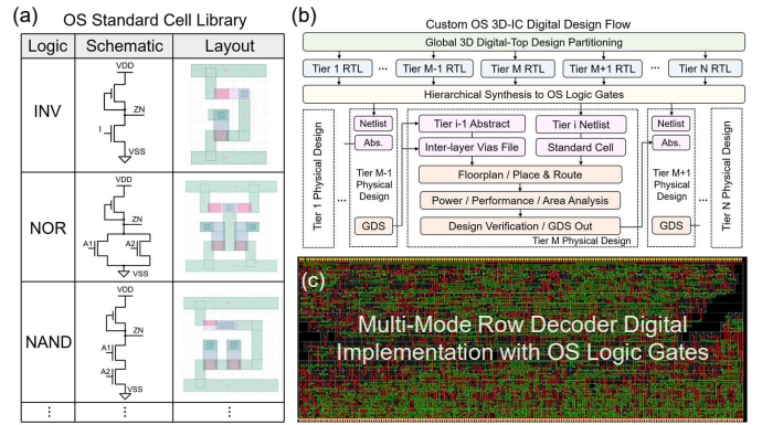
FIGURE 6. Digital circuit design with custom OS PDK. (a) Standard cell library based on InOx transistors. (b) Customized 3D-IC digital design flow. (c) Example result: multi-mode row decoder with OS gates.
