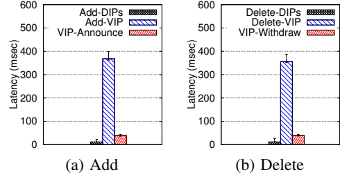
Figure 14: Latency breakdown.
