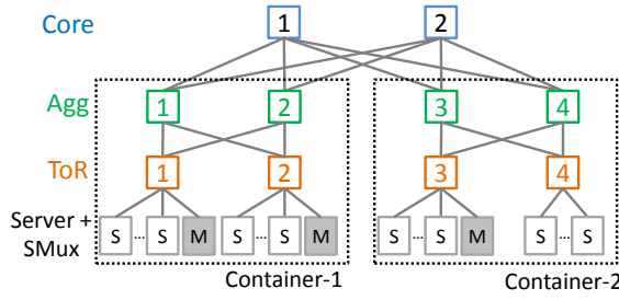
Figure 10: Our testbed. FatTree with two containers of two Agg and two ToR Switches each, connected by two Core switches.
