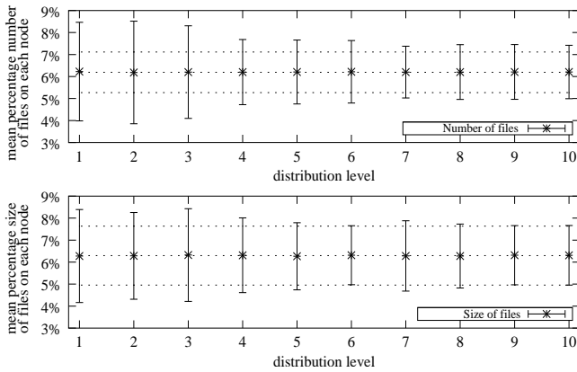
Figure 5: The mean and standard deviation of the percentage of the number of files and their sizes per node across 16 nodes as the distribution level is increased. The dotted horizontal lines show the mean and the standard deviation when each individual file was distributed to a different node, i.e., with the finest grained distribution.
