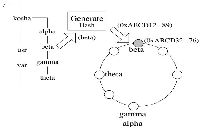
Figure 2: Example of file distribution to multiple nodes. The virtual mount point is /kosha . The directory name is first hashed using the Generate Hash function to generate a unique key, which is then routed using Pastry to a node whose nodeId is numerically closest to the key. The selected Pastry node will provide the physical storage for the directory. The actual file operations, however, are performed via the NFS protocol (not shown).
