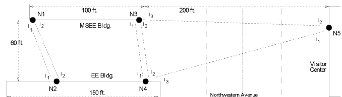
Fig. 5. Purdue MAP testbed schematic (top view). Only outdoor mesh routers are depicted.
