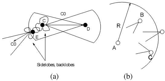
Fig. 3. Channel assignment issues in A-DCA and M-DCA. (a) A-DCA side-lobe interference. (b) M-DCA estimation problem.
