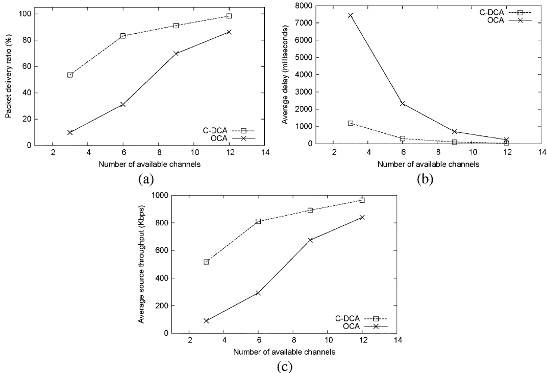
Fig. 4. Impact of a finite number of available channels. Maximum traffic per node is 3 Mb/s. Beamwidth used is 45^\circ . (a) Packet delivery ratio (%). (b) Average delay (ms). (c) Throughput (kb/s).
