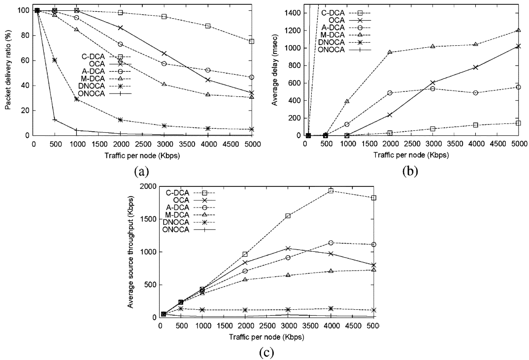
Fig. 2. Comparison of different mesh network architectures. (a) Packet delivery ratio (%). (b) Average delay (ms). (c) Average throughput (kb/s).
