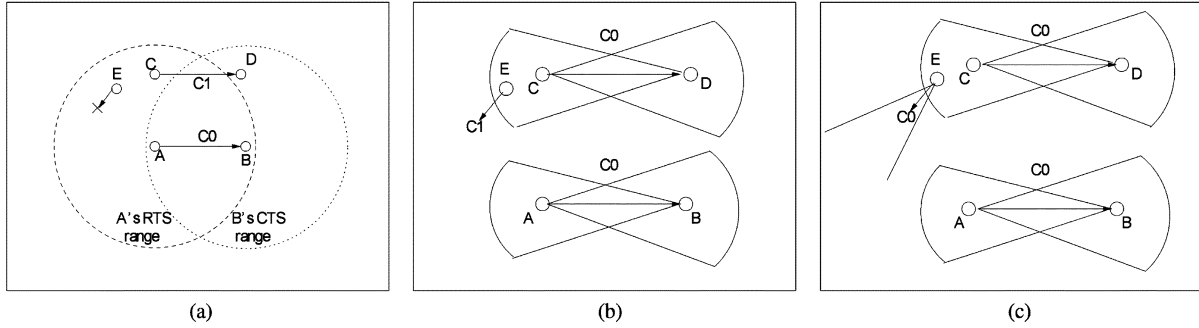
Fig. 1. Channel assignment schemes. (a) Omnidirectional with OCA. (b) Directional with C-DCA. (c) Directional with A-DCA.
