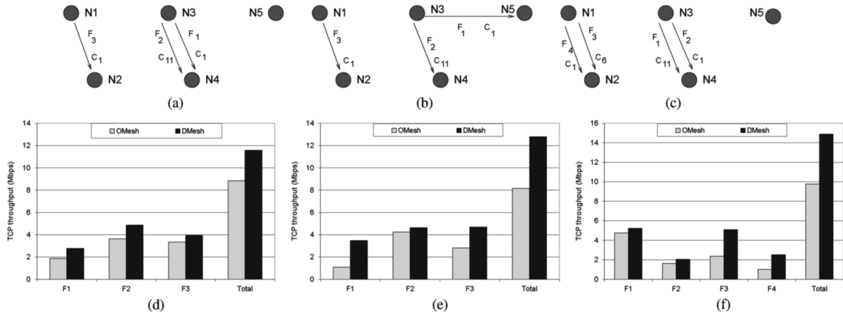
Fig. 6. Testbed results. OMesh is a WMN with omni antennas running OCA, while DMesh is a WMN with practical directional antennas running C-DCA. (a) S1: scenario setup. (b) S2: scenario setup. (c) S3: scenario setup. (d) S1: two channels, three flows. (e) S2: two channels, three flows. (f) S3: three channels, four flows.
