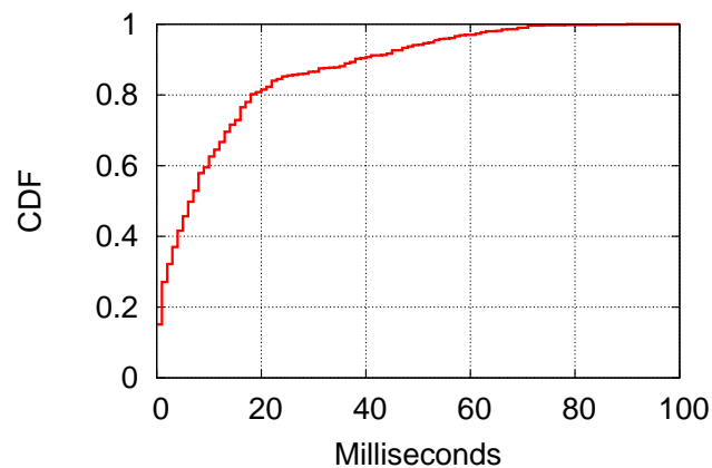
Figure 3: LSP latency difference (max-min) CDF
