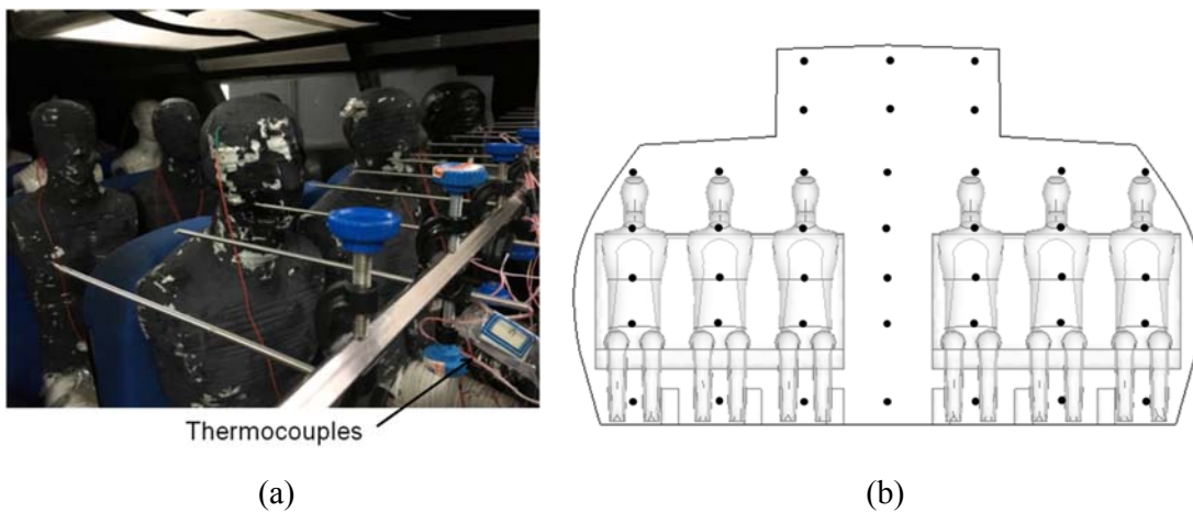
Figure 4. (a) Thermocouples mounted on a stand for measuring air temperature in CS4; and
