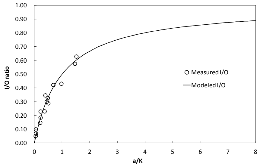
Fig. 4. I/O ratio vs. a/K ratio for measurement and prediction.
