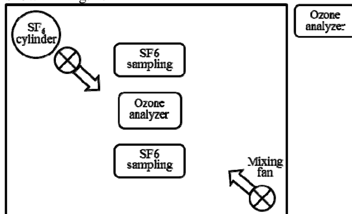
Fig. 2. Setup of the instruments.
