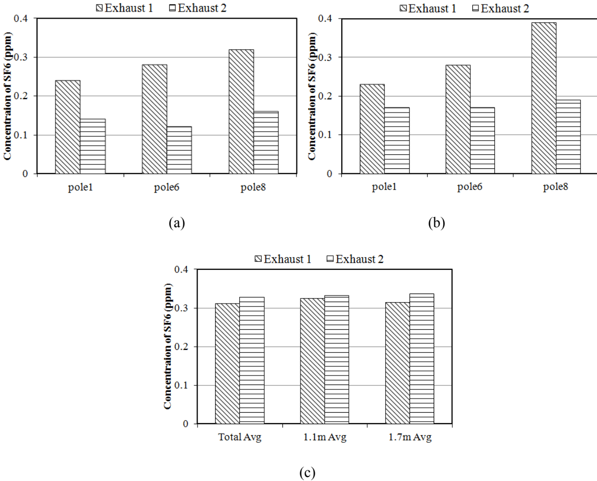
Figure 8 The local contaminant concentration with different exhaust locations at 12 ACH: (a) Average concentration with spill location 1; (b) Average concentration with spill location 2; (c) Average concentration with spill location 3
