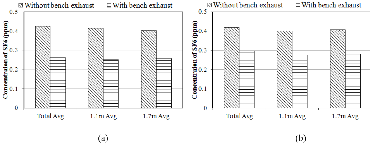
Figure 11 The average contaminant concentration at 6 ACH with wall exhaust or with bench exhaust, (a) at spill location 1 and (b) at spill location 2.
