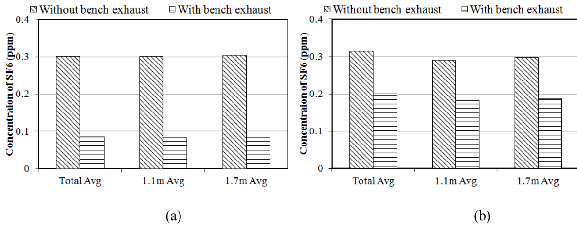
Figure 9 The average contaminant concentration with and without bench exhaust at 12 ACH, (a) at spill location 1 and (b) at spill location 2
