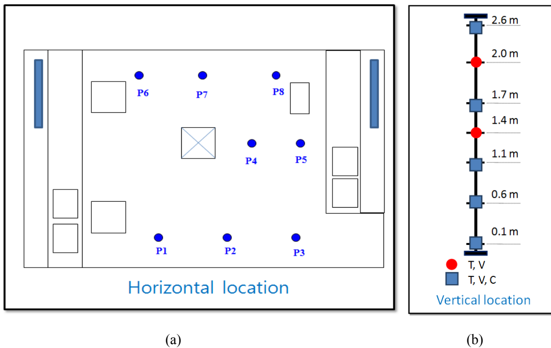
Figure 3 Measurement locations: (a) Horizontal locations; (b) Vertical locations
