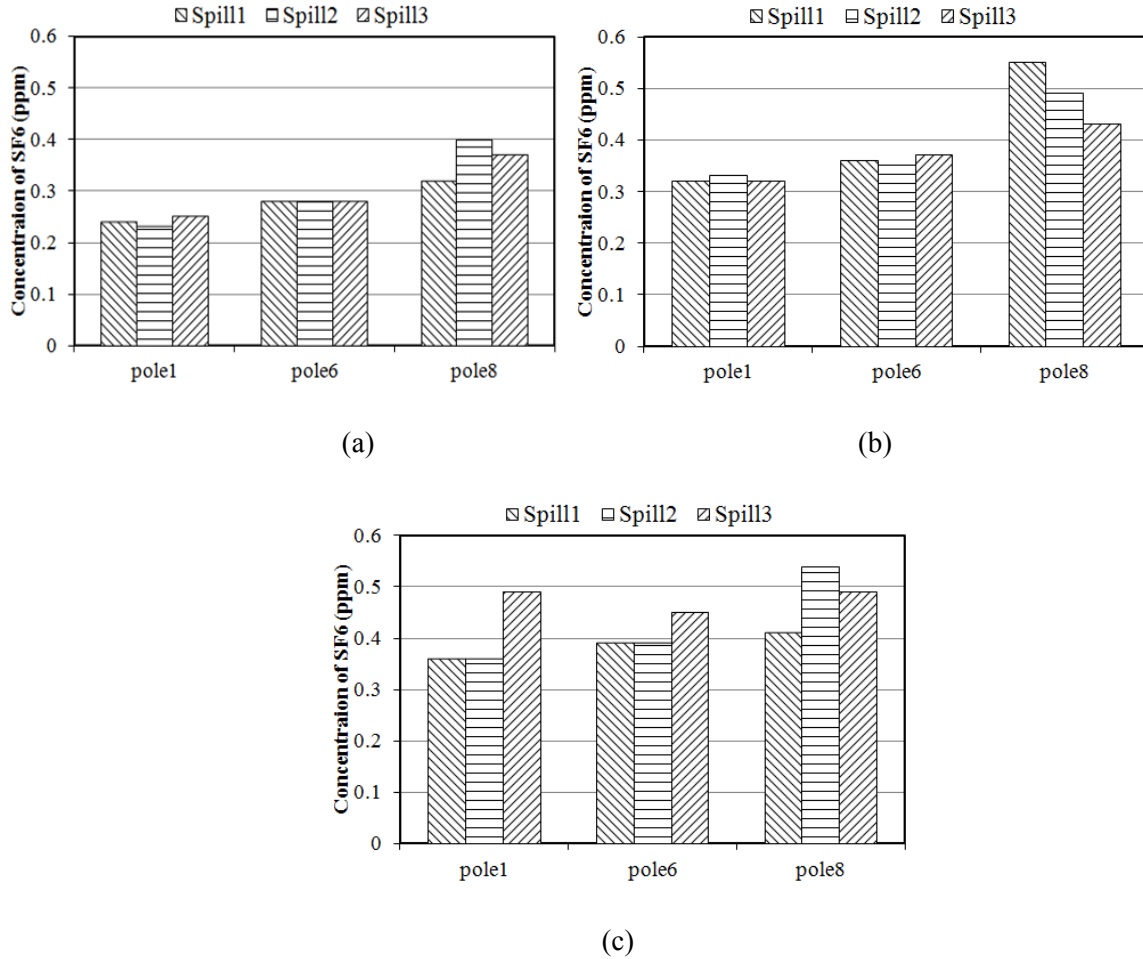
Figure 6 The local contaminant concentration with different spill locations at different ventilation rates: (a) 12 ACH, (b) 9 ACH, and (c) 6 ACH
