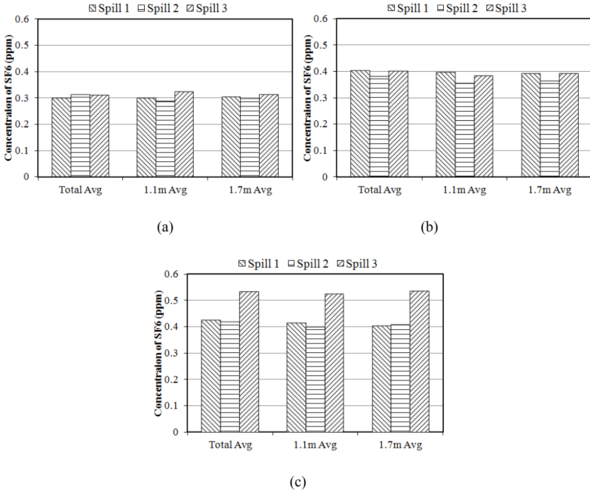
Figure 5 The average contaminant concentration with different spill locations at different ventilation rates: (a) 12 ACH, (b) 9 ACH, and (c) 6 ACH
