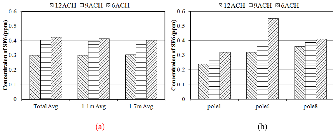
Figure 4 The contaminant concentration at different ventilation rates with spill location 1: (a) Average concentration; (b) Concentration near the occupants
