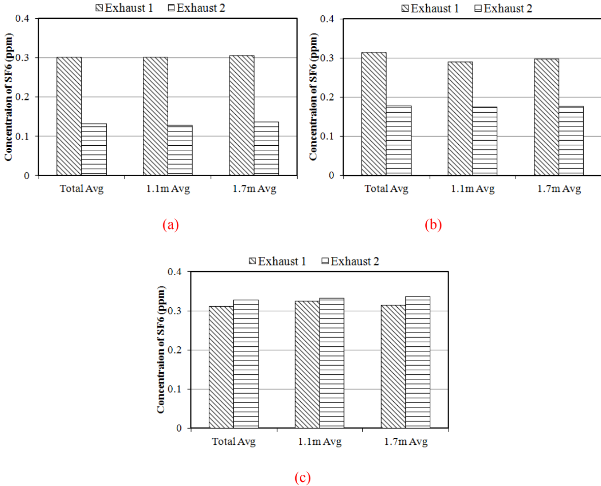
Figure 7 The impact of exhaust location on the average contaminant concentration at 12 ACH: (a) with spill location 1, (b) with spill location 2, and (c) with spill location 3
