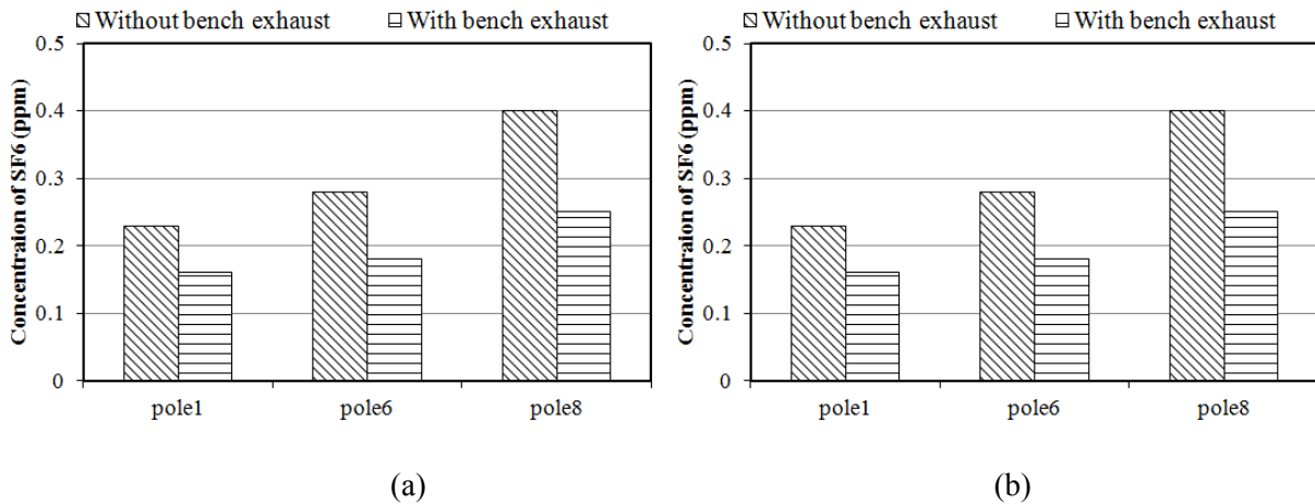
Figure 10 The local contaminant concentration with and without bench exhaust at 12 ACH, (a) at spill location 1 and (b) at spill location 2
