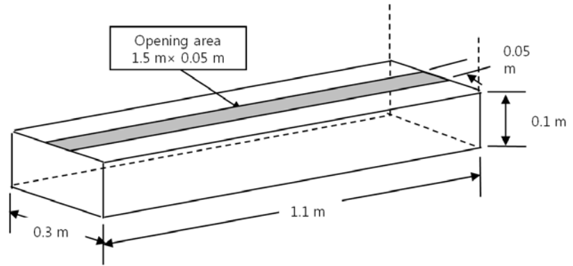
Figure 2 Photo and sketch of the bench hood exhaust
