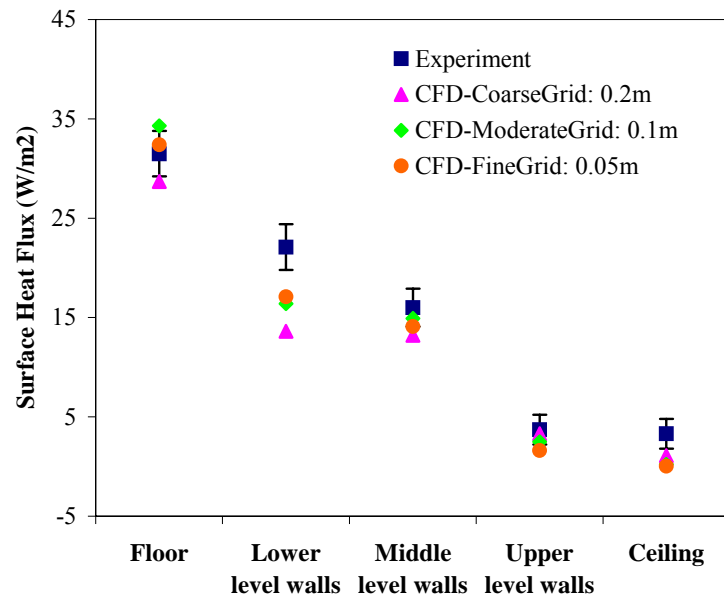
Figure 8 Comparison of simulated heat flux at enclosures with the measurement
