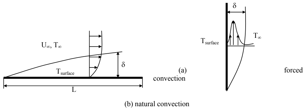
Figure 2 Laminar plate flows of forced and natural convection
