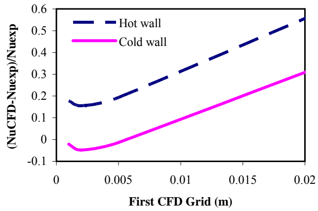
Figure 6 Influence of first CFD grid size on the calculation of Nu at Ra=2.6 \times 10^{10}
