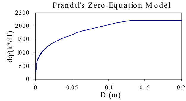
Figure 3 Impact of and first grid size on convective heat by CFD
