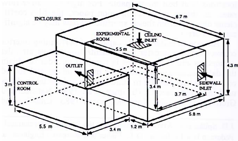
Figure 7 Schematic of experimental facility (Fisher 1995)
