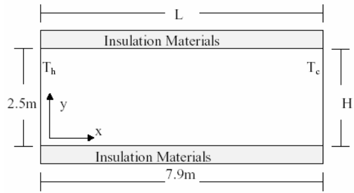
Figure 4 Configuration of the experiment (Olson et al. 1990)
