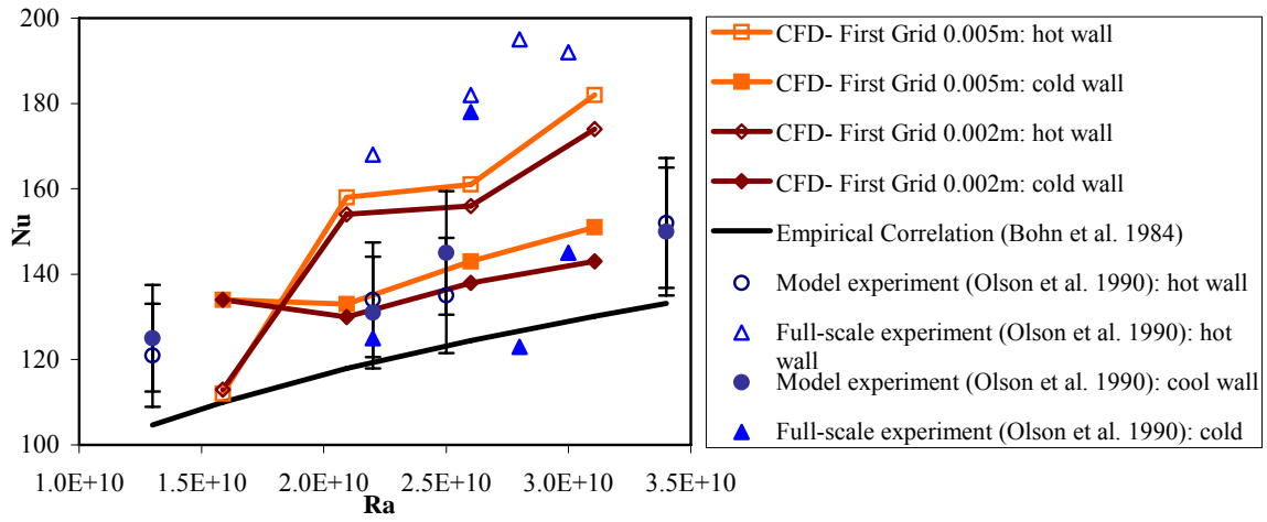
Figure 5 Comparison of simulated heat transfer at enclosures with the data from Olsen et al. (1990).
