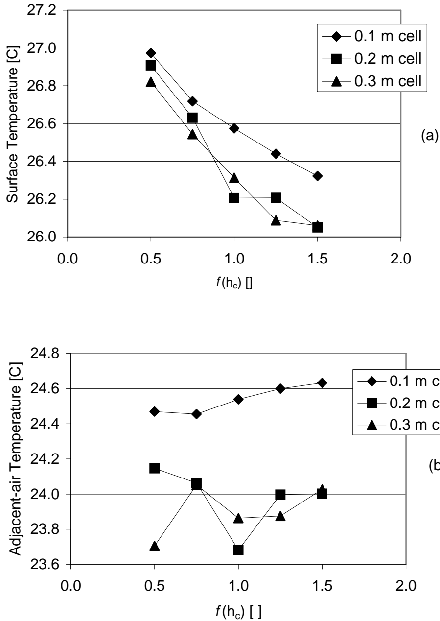
Figure 11 Variation in (a) surface and (b) adjacent-air temperatures for an upper glazing panel (adding heat to air) with different input levels for h_{c,i} 's and t_{cv} , case VTTC_cooling 10x10x8 momentum zonal air model
