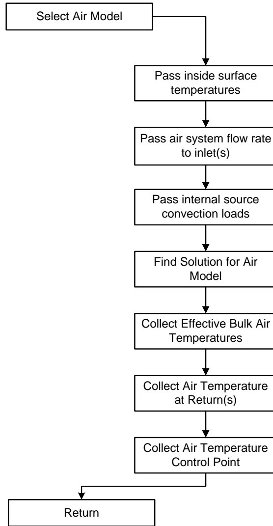
Figure 4 General steps in calling an air model
