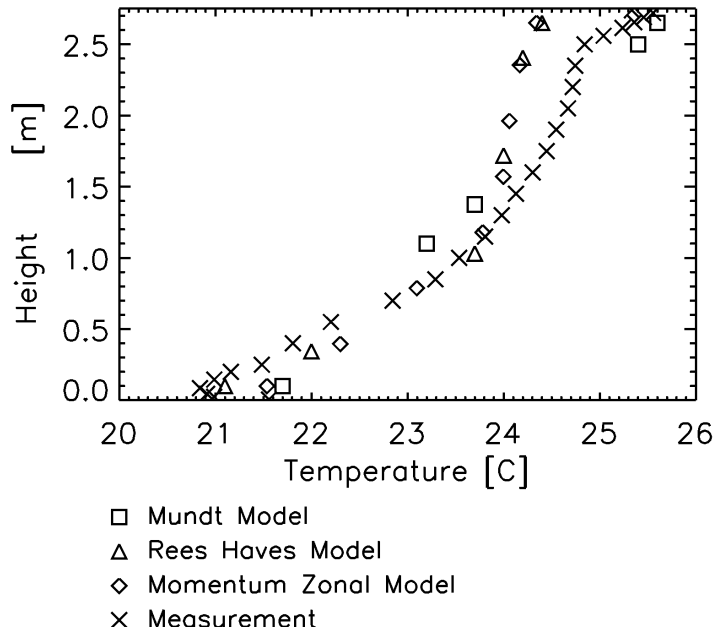
Figure 5 Indirect coupled air and load routines results for air temperatures: case B3 (Li et al. 1993)
