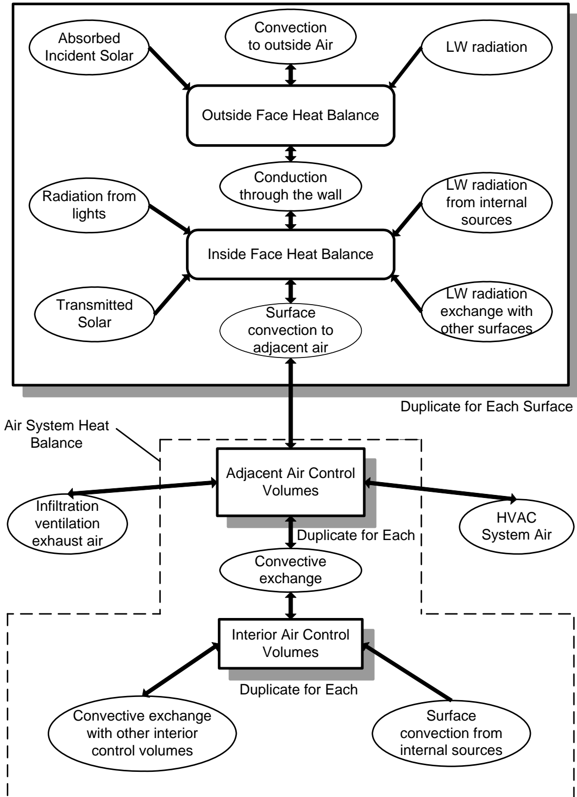
Figure 2 Schematic of heat balance processes in a zone with air models
