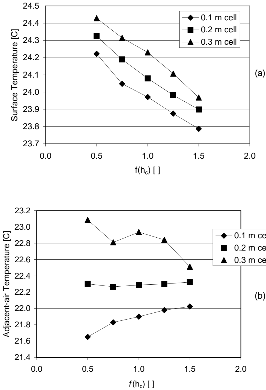
Figure 10 Variation in (a) surface and (b) adjacent-air temperatures for a lower insulated wall (adding heat to air) with different input levels for h_{c,i} 's and t_{CV} , case VTTC_cooling 10x10x8 momentum zonal air model
