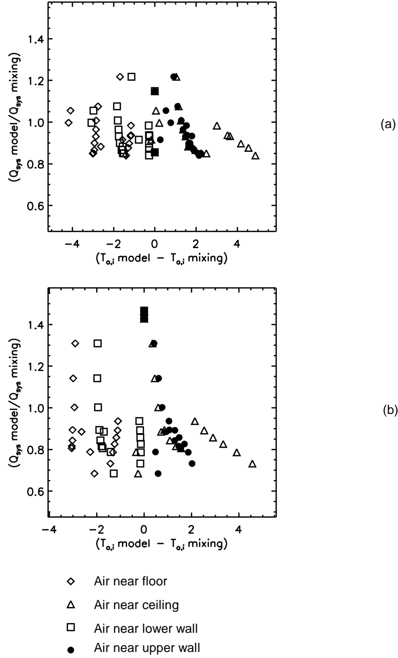
Figure 9 Ratio of change in \dot{Q}_{sys} with momentum-zonal air model to \dot{Q}_{sys} with well-mixed model as a function of deviations in T_{o,i} (a) with carpet and (b) without carpet
