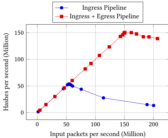
Figure 2: By using both ingress and egress pipelines, we increased our implementation’s maximum hash rate by 3x.
