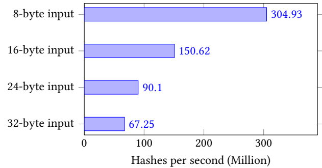
Figure 3: Hash rate of HalfSipHash on programmable switch under different input length.
