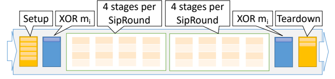
Figure 1: We run two SipRounds per switch pipeline pass, with each SipRound costing four stages.
