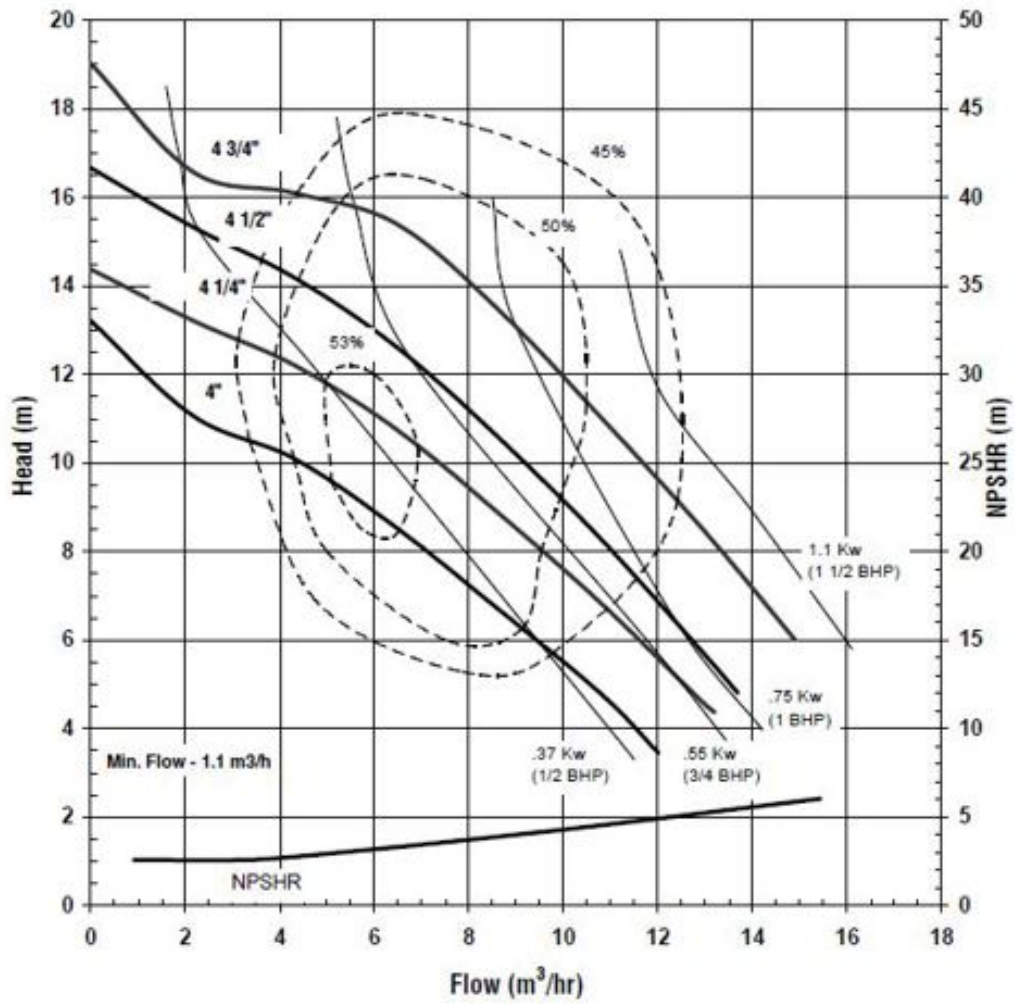
Figure 4. Pump curves for Finish Thompson AC5 series incorporating NPSH-R chart.
