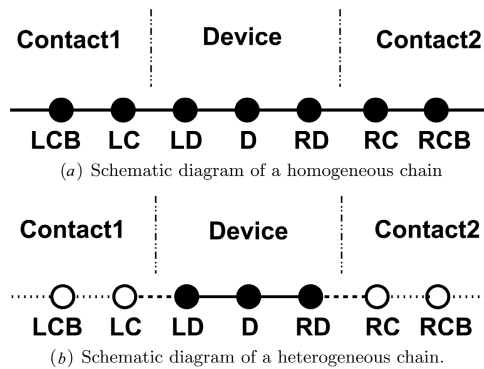
Figure 3. Homogeneous and heterogeneous atomic chain examples. Filled and open circles represent different types of atoms. The dotted, dashed, and solid lines between atoms represent different bonds.
