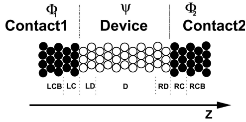
Figure 1. Schematic diagram for a general contact-device-contact setup.
