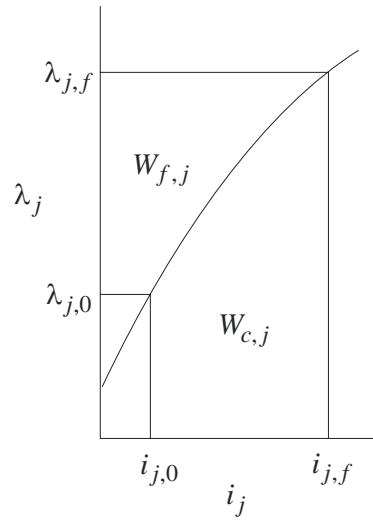
Figure5.1-1. Field Energy and Co-Energy.
