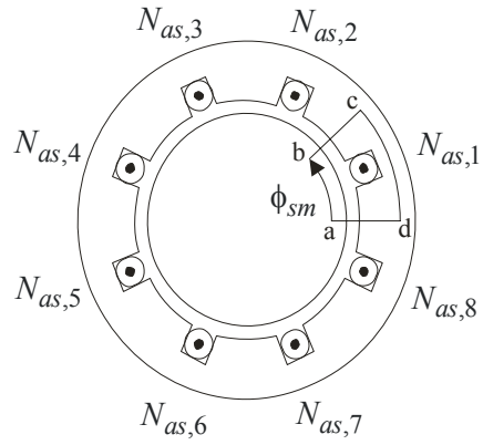
Figure 4.2-1. Slot Structure.
