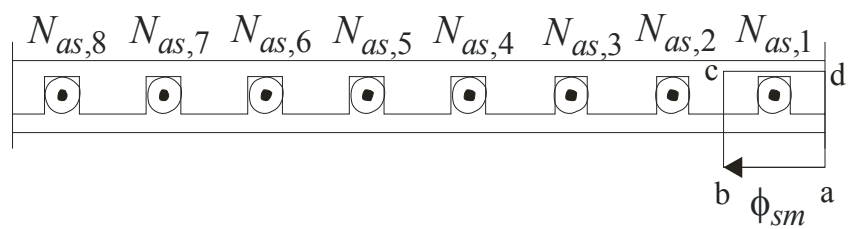
Figure 4.2-2. Developed Diagram.
