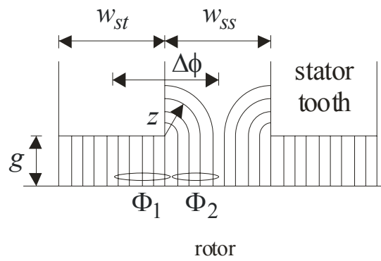
Figure 4.6-2. Carter's Coefficient
