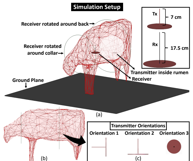
Fig. 5: (a) Model used for FEM simulations showing the dimensions of the transmitter and receiver. (b) Side view of the simulation model. (c) Simulations are performed with 3 different orientations of the transmitter.
