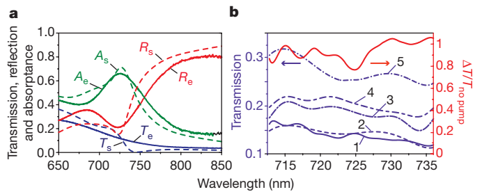
Figure 3 | Experimental results and simulation. a , Experimental far-field transmission ( T_e ), reflection ( R_e ) and absorption ( A_e ) spectra of the sample, along with simulated results ( T_s , R_s , and A_s ) at the primary linear polarization shown in Fig. 2a. b , The transmission spectra without pumping (line 1), with the optimized delay between pump and probe (probe pulse is 54 ps later than the pump) and 1-mW pumping power (line 5), with the optimized delay and 0.12-mW pumping power (line 3), with the optimized delay and 0.16-mW pumping power (line 4), and with the pump preceding the probe by 6 ps and 1-mW pumping power (line 2). The wavelength-dependent relative transmission change from the pump-probe experiment is shown by the red solid line.
