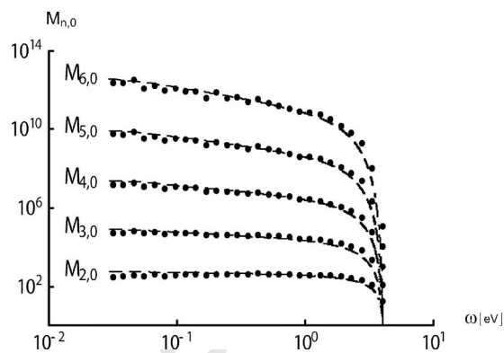
FIG. 3. The local-field moments M_{n,0} (dots) are calculated with the exact numerical method and compared to the analytical results with exponent \gamma=0.14 (dashed lines). The numerical data are averaged over 20 realizations of percolation systems with size L=250 . In the analytical estimates we use t \approx s \approx \nu \approx 4/3 (Ref. 9).
