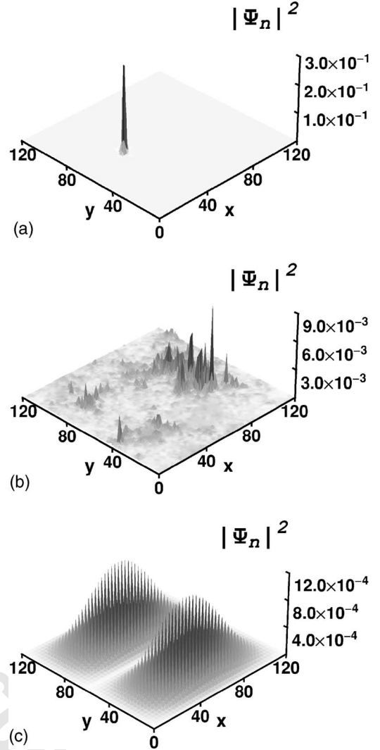
FIG. 1. Surface plasmon eigenmodes in random (a), (b) and periodic (c) metal-dielectric films. The corresponding eigenvalues are: (a) \Lambda = -5.6945 (localized), (b) \Lambda = 0.0044 (delocalized), (c) \Lambda = -5.9974 (periodic).
