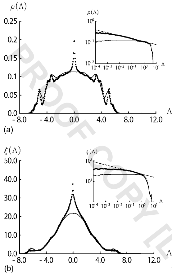
FIG. 2. The density of states \rho(\Lambda) (a), and the SP localization lengths \xi(\Lambda) (b) for the KH (dots) and for the corresponding Anderson problem (solid line), calculated at the resonant condition \varepsilon_d^* = -\varepsilon_m^* = 1 . The band-center singularity is shown in the log-log insets where a power-law fit (dashed line) with exponent \gamma = \alpha = 0.14 is applied. The data is averaged over 100 different realizations of percolation samples each with size L = 120 .
