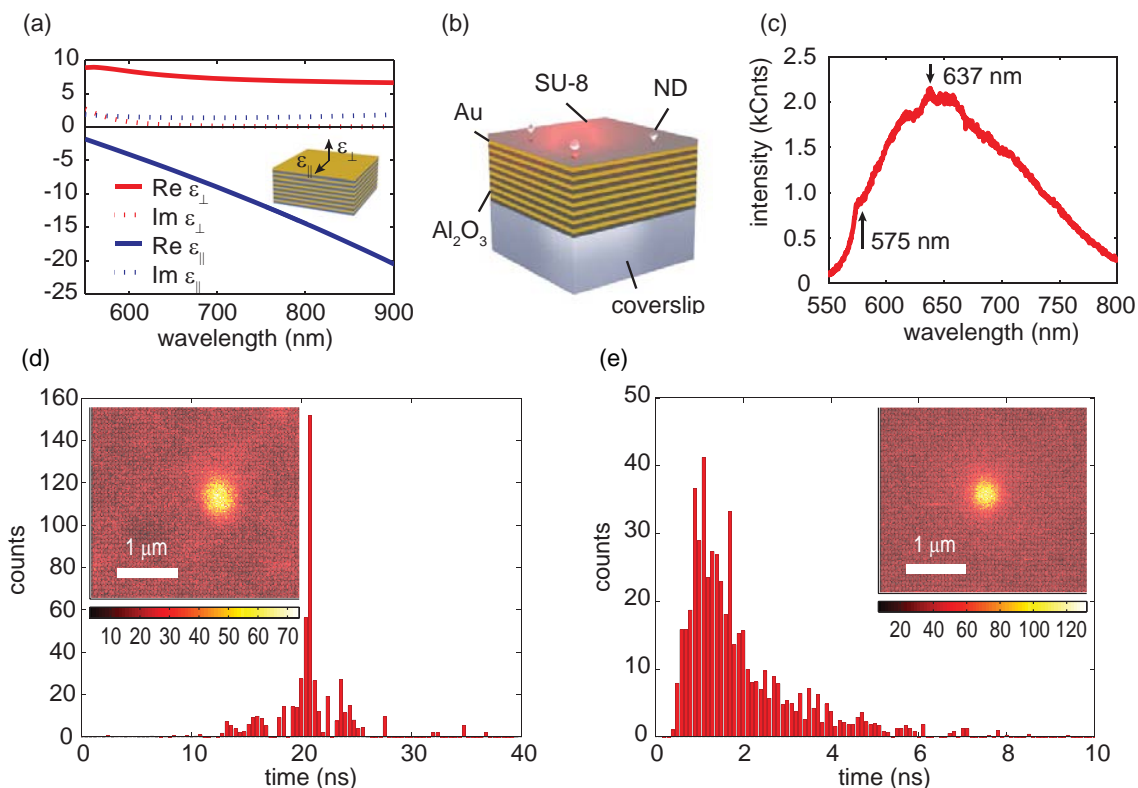
Fig. 1. Coupling nitrogen-vacancy (NV) centers in nanodiamonds (ND) with a hyperbolic metamaterial (HMM). (a) Dielectric functions of fabricated HMM (16 alternating layers of Au and Al 2 O 3 , thickness of each layer – 19 nm) retrieved by spectroscopic ellipsometry measurements, within the range of the plot (550 – 900 nm) \text{Re } \epsilon_{\perp} > 0 , \text{Re } \epsilon_{\parallel} < 0 , hence leading to hyperbolic dispersion. (b) Schematic of the experimental sample consisting of the HMM, 30-nm-thick spacer layer composed of SU-8 photoresist, and NDs with NV centers inside. (c) Emission spectra of NV centers when NDs are placed on HMM. Experimentally measured spontaneous emission lifetimes of the NV centers on (d) coverslip, (e) HMM. Corresponding mean values (standard deviations) of the lifetime distributions are: (d) 20.89 ns (1.15 ns), (e) 1.55 ns (0.95 ns).
