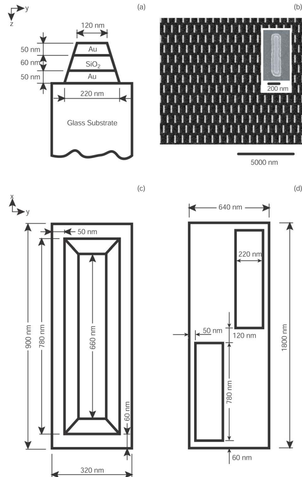
Fig. 12. (c) Single-periodic and (d) skewed-periodic structures of coupled gold rods deposited on a bare glass substrate. Both models used the same rod pairs shown in (a). Geometry in (d) simulates a fabricated sample (sample B). (b) SEM image of sample B.
