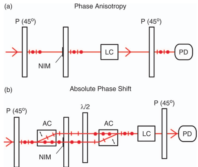
Fig. 6. Schematics of (a) polarization and (b) walk-off interferometers for measuring phase anisotropy and absolute phase induced by a NIM sample. LC is a liquid-crystal phase compensator, P is a 45-deg linear polarizer, AC is an anisotropic calcite crystal with a walk-off effect, \lambda/2 is a half-wave plate, and PD is a photodetector.
