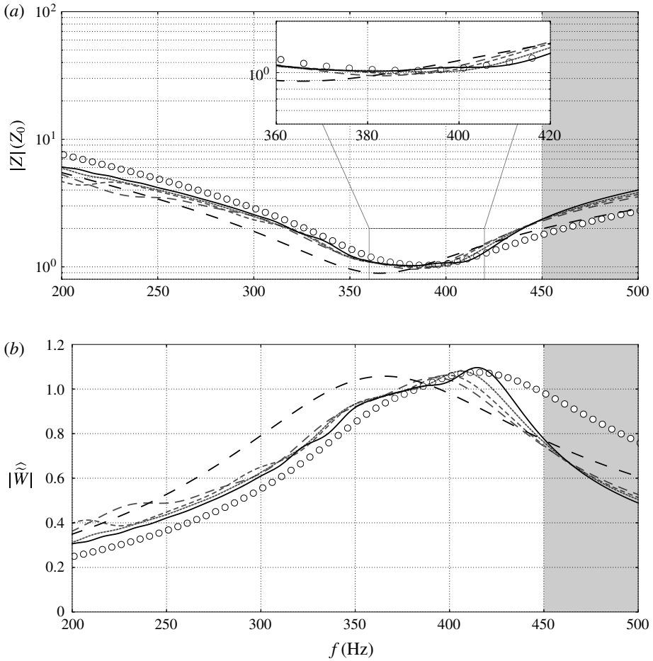
FIGURE 15. Magnitude of experimentally measured impedance (6.5) (a) and (b) wall softness magnitude (O) compared with multi-oscillator model for \bar{\alpha} = 0.2237 ( n_o = 1 ) (—), \bar{\alpha} = 0.12 ( n_o = 4 ) (---), \bar{\alpha} = 0.10 ( n_o = 6 ) (- - -), \bar{\alpha} = 0.08 ( n_o = 13 ) (.....), to 0.06 ( n_o = 18 ) (——). The shaded area highlights the frequency interval f > 450 Hz of negative resistance \text{Re}\{Z_{\text{exp}}(\omega)\} < 0 for the experimentally determined impedance (6.5), deemed unphysical.
