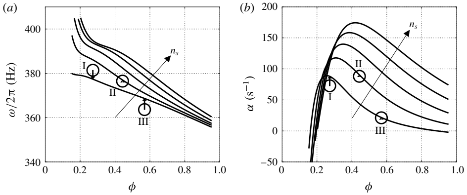
FIGURE 8. Frequency (a) and growth rate (b) versus stack porosity during start-up phase. Results from the nonlinear Navier–Stokes simulations (○) for temperature setting 5 and grid resolution/stack-type C/I, C/II and C/III; predictions from linear theory for n_s = 3, 5, 7, 9 and 11 (—). Vertical arrows denote the difference between the linear theory prediction and Navier–Stokes simulations.
