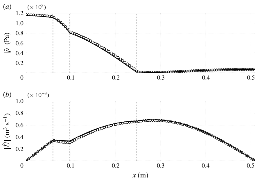
FIGURE 6. Axial distribution of pressure (a) and flow-rate (b) amplitudes of the thermoacoustically unstable mode for temperature setting 5 and grid resolution/stack-type C/I, as predicted by linear theory (—), rescaled to match amplitudes extracted from Navier–Stokes simulations (○) during the start-up phase. The frequency predicted by linear theory is f = 378.9 Hz, while the frequency extracted from the Navier–Stokes calculations yields f = 381.8 Hz (see figure 5). Vertical dashed lines indicate locations of abrupt area change (figure 1).
