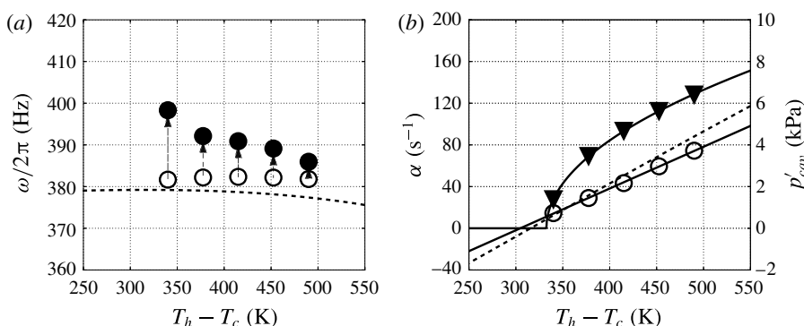
FIGURE 5. Frequency (a) and growth rate (b) versus temperature difference, \Delta T = T_h - T_c , for grid resolution/stack-type C/I. Predictions from linear model (—) and Navier–Stokes simulations at start-up (○); limit cycle frequencies (●); square-root fit (4.1) (—) of limit cycle pressure amplitudes (▼) in the hot cavity versus temperature difference; and linear fit of growth rates from Navier–Stokes calculations (—).
