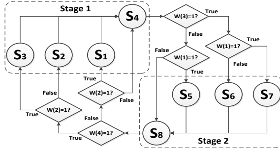
Figure 3: Phase transition of intelligent traffic control.
