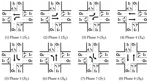
Figure 2: Signal phases of intelligent traffic control.
