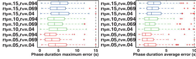
Figure 6: Phase duration error distribution under different r_{fp} ( =r_{fn} ).
