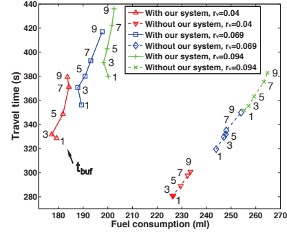
Figure 8: Fuel consumption and travel time for different t_{buf} .
