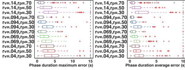
Figure 5: Phase duration error distribution in stage 1 (figure for stage 2 is similar). For each box, central mark is the median, edges are the 25th and 75th percentiles, whiskers covers 99.3% data points, and outliers are red crosses limited by the vertical dashed line.
