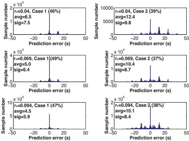
Figure 7: Prediction timing error distribution. avg and sig are average and standard deviation of prediction error.
