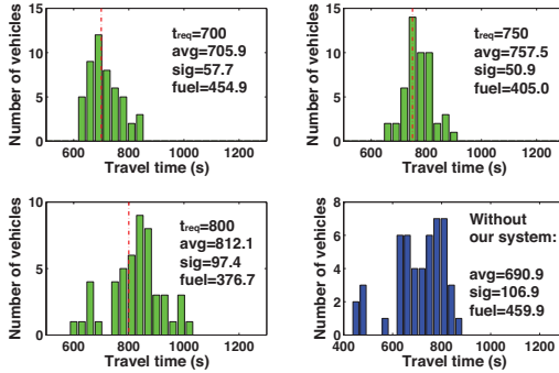
Figure 9: Travel time distribution under different travel time requirements. avg and sig are average and standard deviation of recorded travel time.
