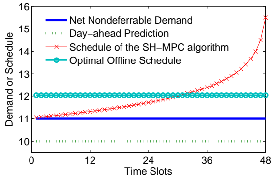
Fig. 2. Poor performance of the SH-MPC algorithm. In this example, the day-ahead prediction consistently underestimates the real demand, and the SH-MPC algorithm leads to a peak that is 1.29 times higher than the optimal offline peak. In comparison, an optimal online algorithm can achieve a peak that is at most 1.06 times higher than the optimal offline peak.
