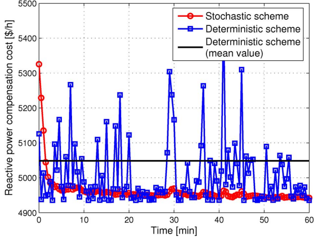
Fig. 3. Reactive management cost for the 47-bus distribution grid ( \eta_t = 2 ).
