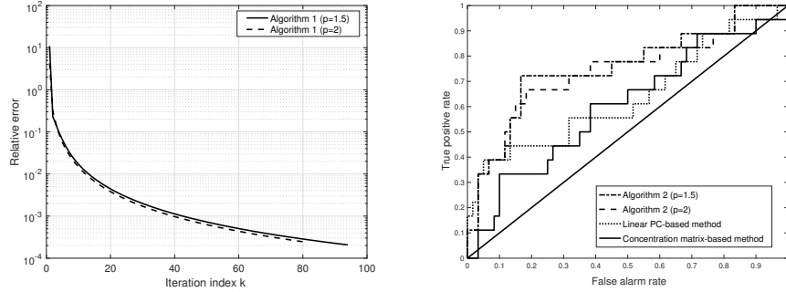
Figure 0.2 Topology recovery for the IEEE 14-bus system. Left : Convergence speed for the devised Frank-Wolfe iterations; Right : ROC curves for line detection.
