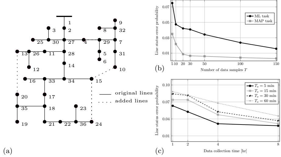
Figure 0.1 a) Line structure for the IEEE 37-bus feeder. b) Line error probability for the ML and the MAP task. c) Line error probability for the ML task (0.10). c) Effect of T_s on the line status error probability for the ML task.
