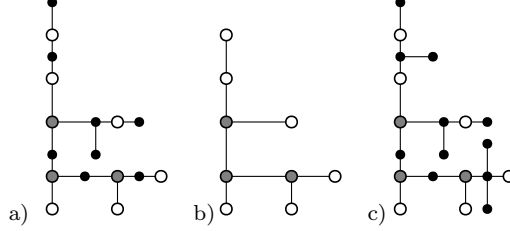
Figure 0.6 a) the original feeder; b) its reduced equivalent; and c) another feeder with the same \mathbf{R}_{\mathcal{PP}} . White nodes are probed; black and gray are not. Gray nodes are internally identifiable nodes comprising \mathcal{I} .
