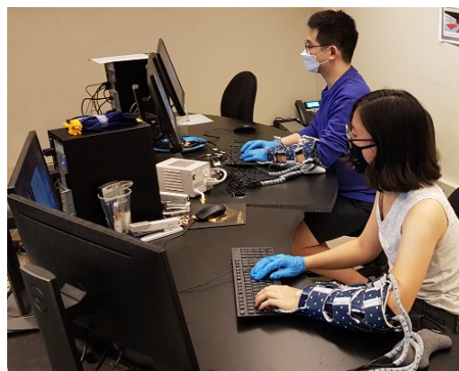
Figure 5. Photo of two-way messaging via TAPS. Each participant wore a TAPS system on the left forearm to receive text messages. They recorded received messages and sent new messages on computer keyboards.
