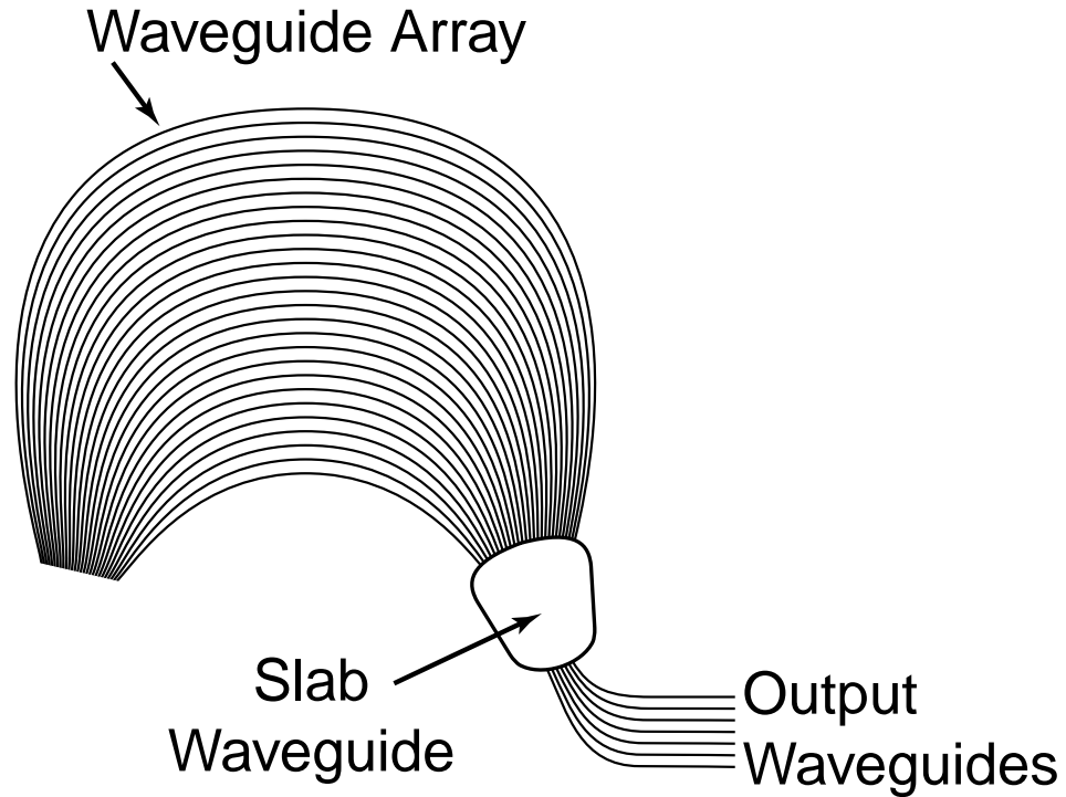
Fig. 4.8. DST-AWG device schematic.
