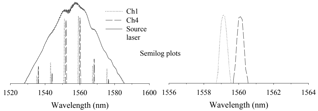
Fig. 4.5. Measured power spectra from the 40 GHz output channel spacing AWG. Both the full wavelength span (left) and the expanded (right) curves are plotted on a semi-log scale to more readily show the multiple filter passbands.
