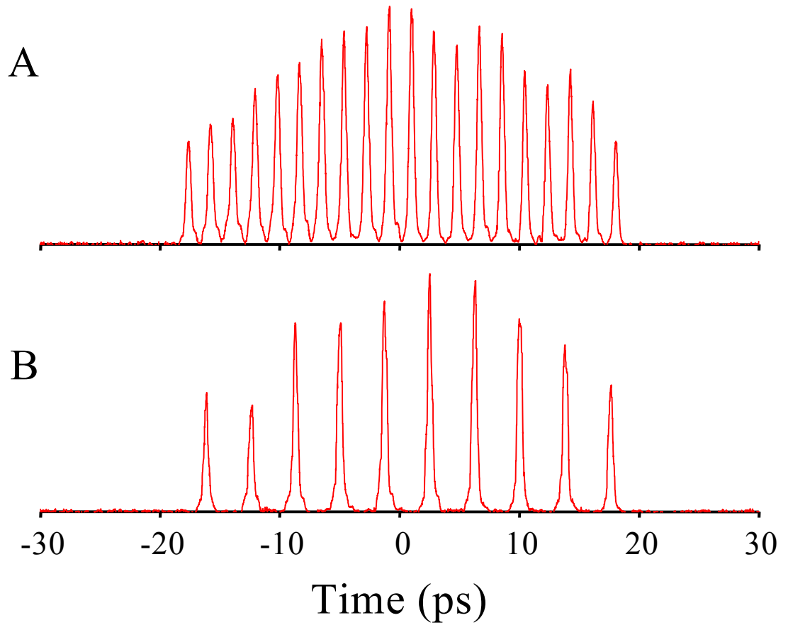
Fig. 3.9. Measured pulse trains utilizing periodic pixelation masks.
