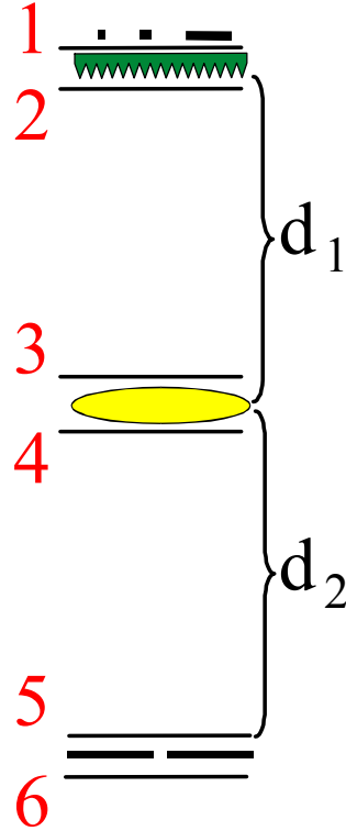
Fig. 3.13. Relevant planes considered in the diffraction analysis
