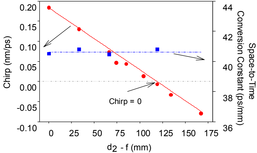
Fig. 3.14. Measured chirp and space-to-time conversion constant as a function of pulse shaping lens-output slit separation.
