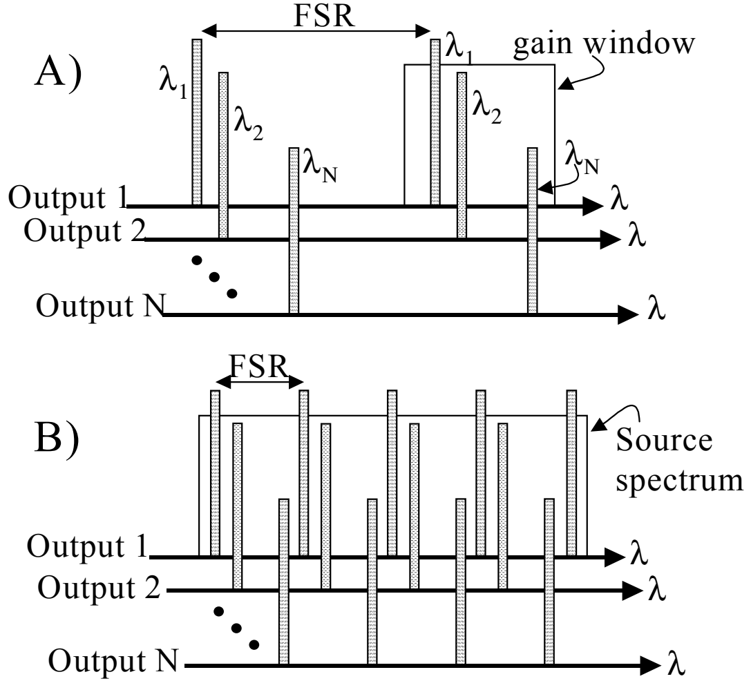
Fig. 4.3. Filter design methodologies for (A) traditional AWG filters, and (B) DST pulse shaping using an AWG.
