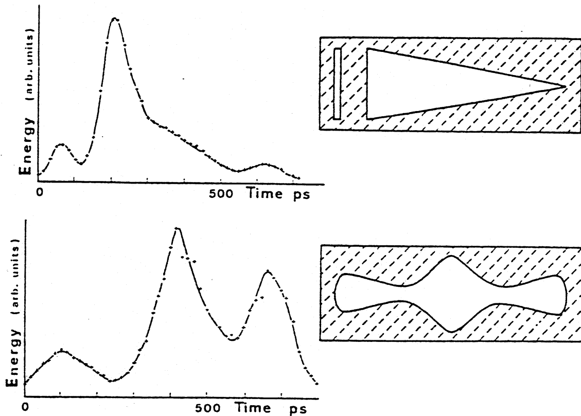
Fig. 3.1. The first 'DST' pulse shaping data (left) and spatial masking functions (right) reported by Froehly et. al. [22].
