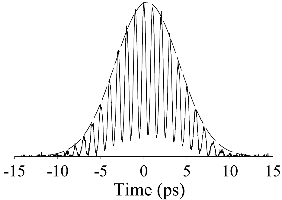
Fig. 4.7. Measured intensity cross correlation (solid) from the 100 GHz output channel spacing device overlaid with the calculated temporal window (dash).
