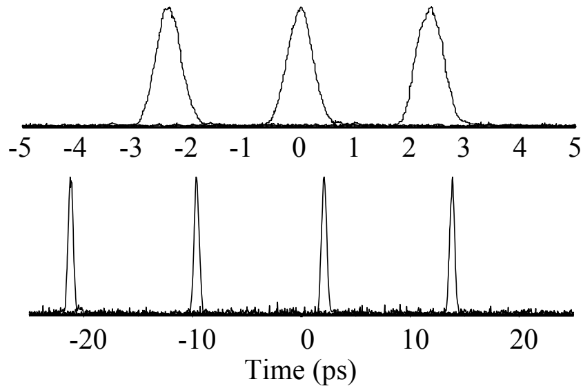
Fig. 3.8. Measurement of the space-to-time conversion constant.
