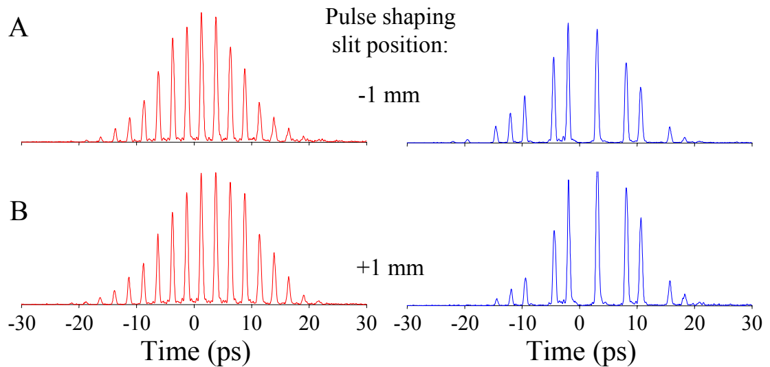
Fig. 3.19. Intensity cross correlation measurements of the DST pulse shaper output for two different transverse positions of the pulse shaping slit separated by 2 mm.
