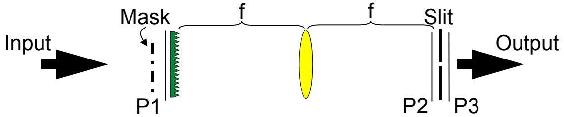
Fig. 3.3. Schematic diagram of the DST pulse shaper.
