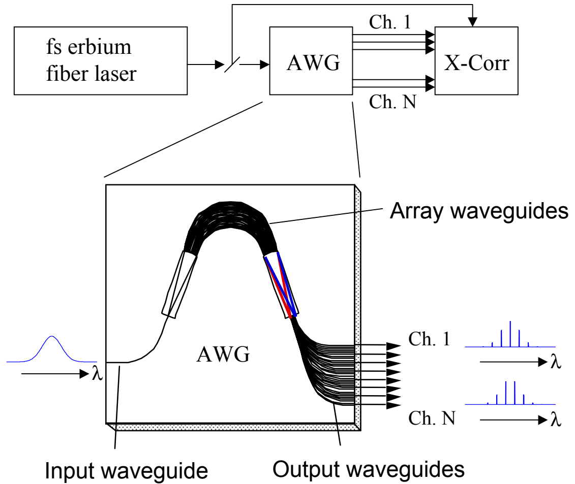
Fig. 4.4. Experimental apparatus for AWG pulse train generation experiments.
