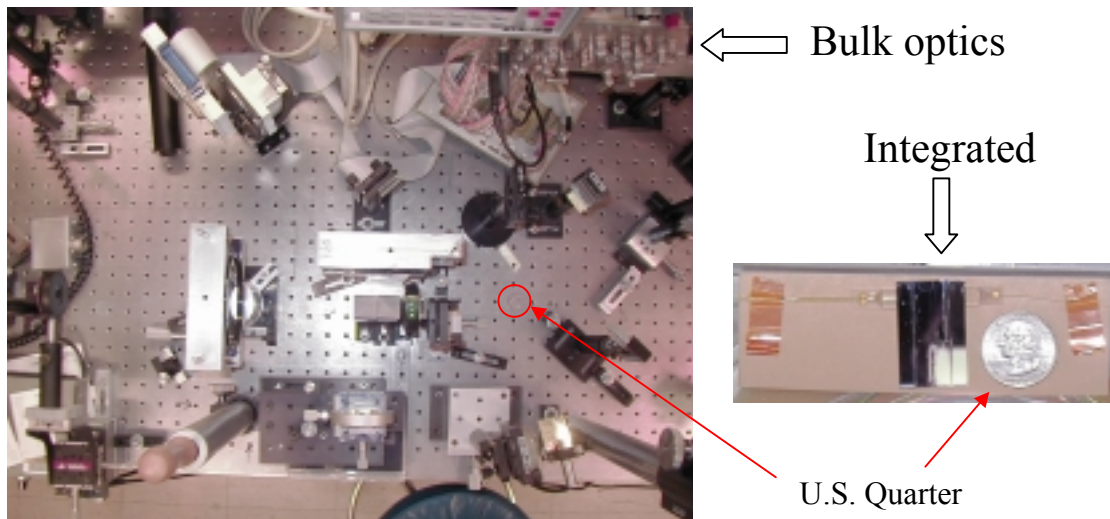
Fig. 4.1. Photos of the bulk optics DST pulse shaper (left) and an AWG (right).
