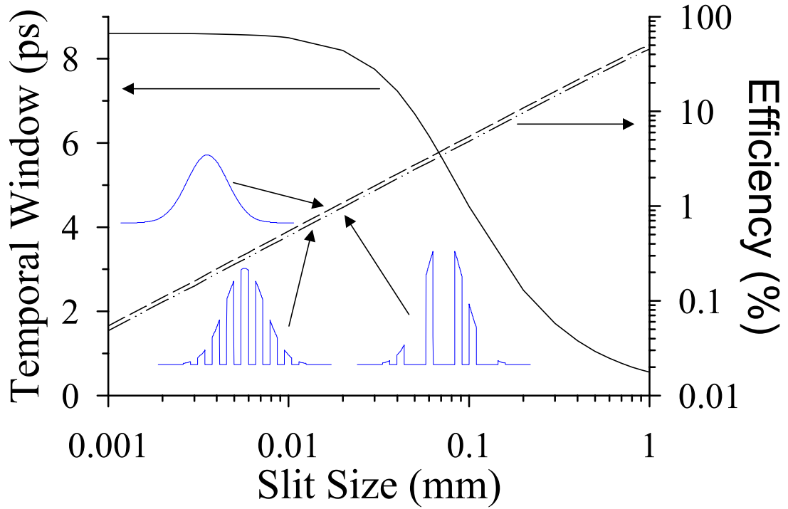
Fig. 3.11. Calculated temporal window and optical efficiency as a function of pulse shaping slit width.
