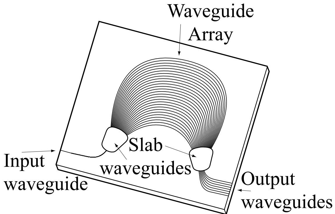
Fig. 4.2. AWG Structure.
