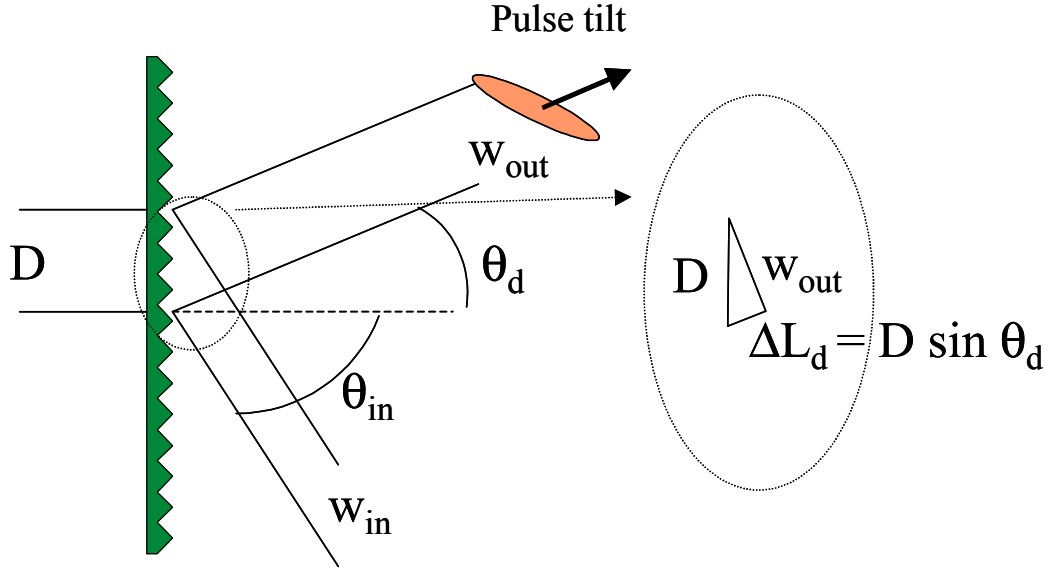
Fig. 3.4. Trigonometric argument for determining the space-to-time conversion constant.
