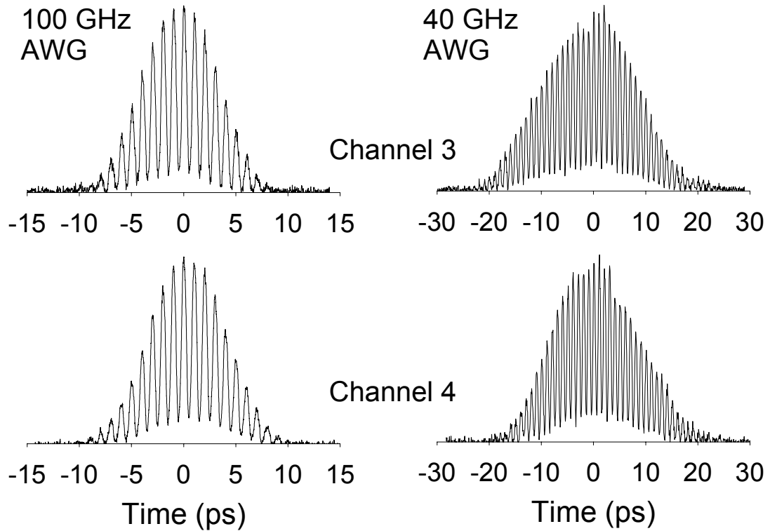
Fig. 4.6. Intensity cross correlation measurements of the 100 GHz output channel spacing (left) and 40 GHz output channel spacing (right) devices for output channels 3 (top) and 4 (bottom).
