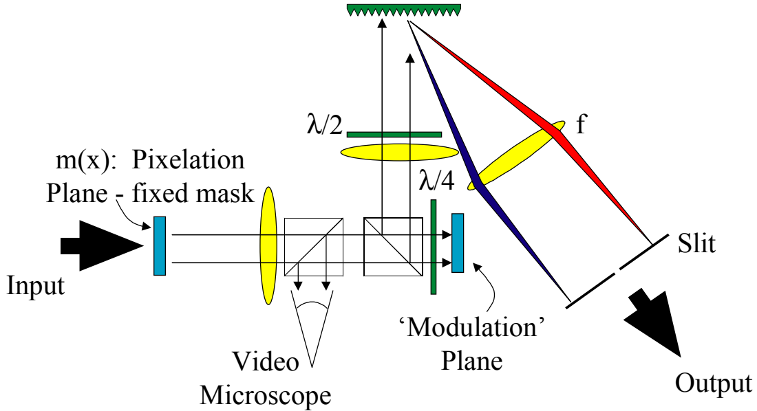
Fig. 3.7. Final DST apparatus with image plane viewing optics.
