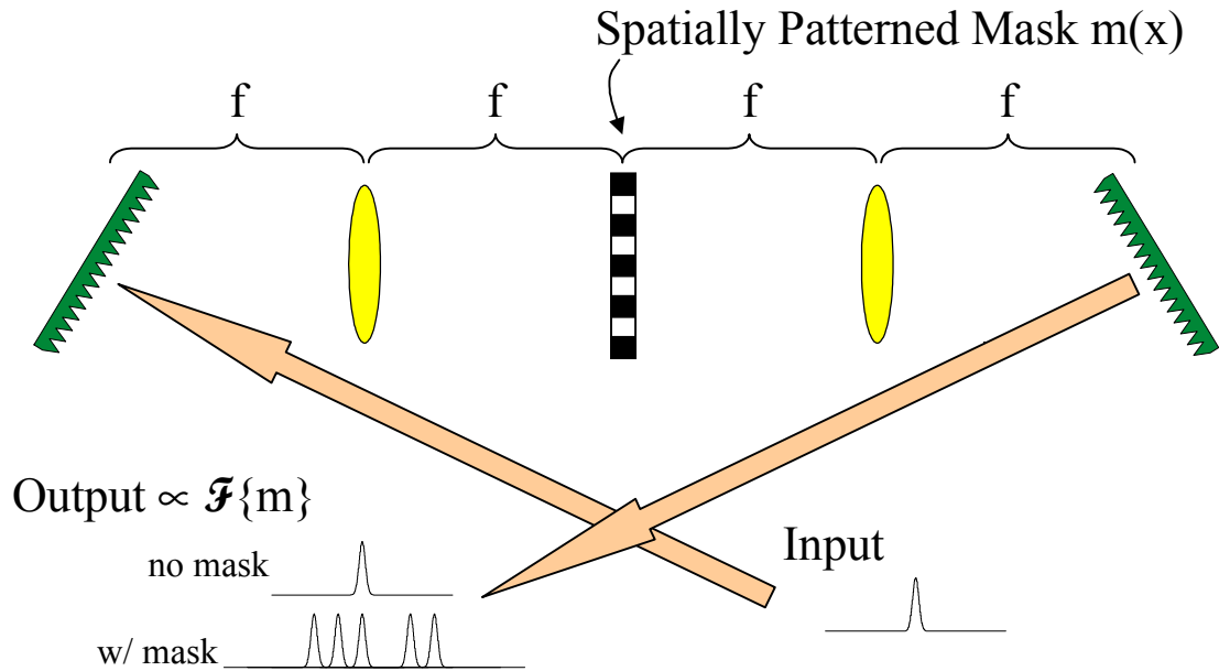
Fig. 2.1. Fourier transform pulse shaping geometry.
