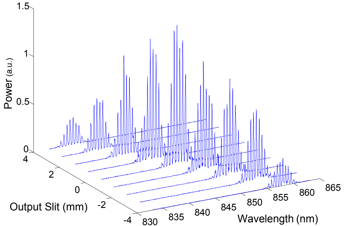
Fig. 3.18. Output power spectra as a function of transverse pulse shaping slit position for a periodic pixelation mask.
