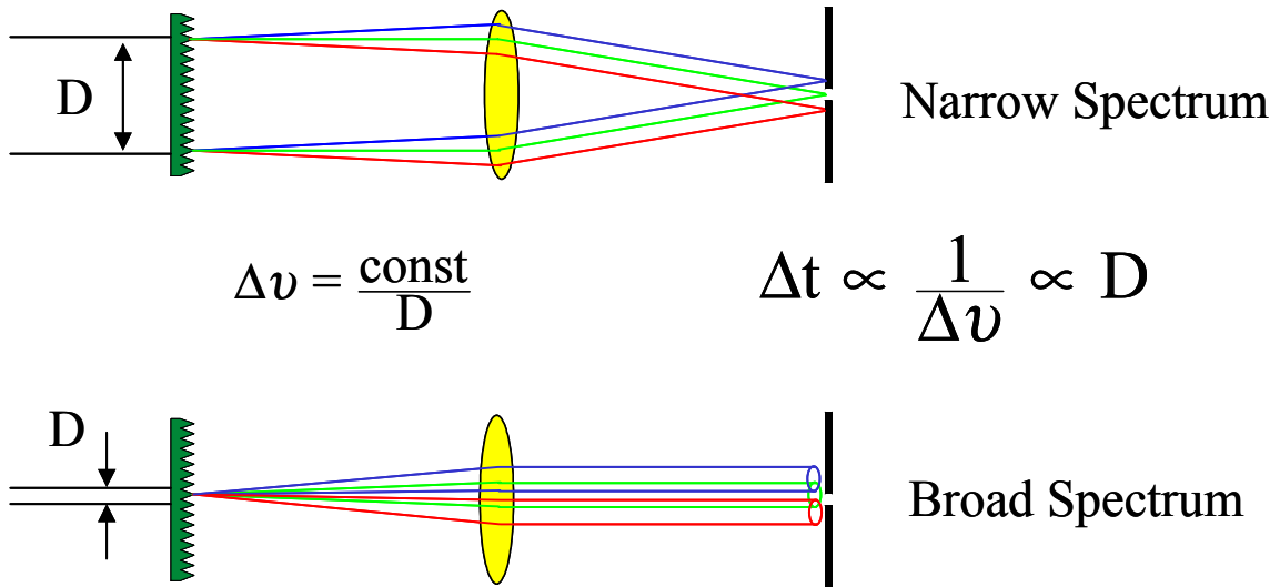
Fig. 3.5. Spectrometer analogy for the DST pulse shaper.
