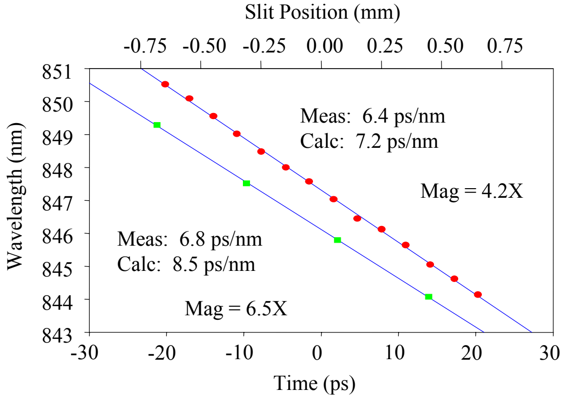
Fig. 3.12. Shift in output center wavelength as a function of input pixelation slit position (in space and time). The slope provides a measure of the chirp on the output of the DST pulse shaper.
