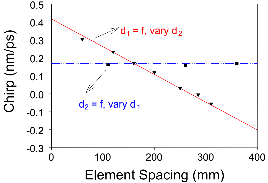
Fig. 3.15. Measured and calculated chirp for two interesting specific cases of the diffraction analysis result. Solid line is calculated and triangles are measured for grating-lens separation, d_1 = f , but lens-slit separation allowed to vary. Dashed line is calculated and squares are measured for lens-slit separation held fixed at the focal length of the pulse shaping lens while grating-lens separation is allowed to vary.
