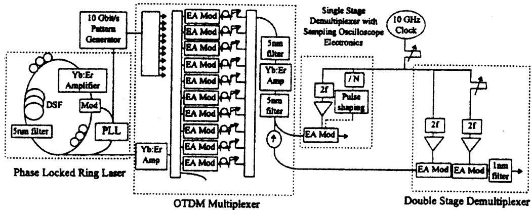
Fig. 2.2. Schematic diagram of the 100Gbit/s testbed used in [48].
