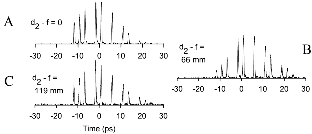
Fig. 3.17. Intensity cross correlation measurements of the DST pulse shaper output for an 'optical packet' pixelation mask, and three values of output chirp. (A) is heavily chirped, (B) moderately, and (C) approximately chirp-free.
