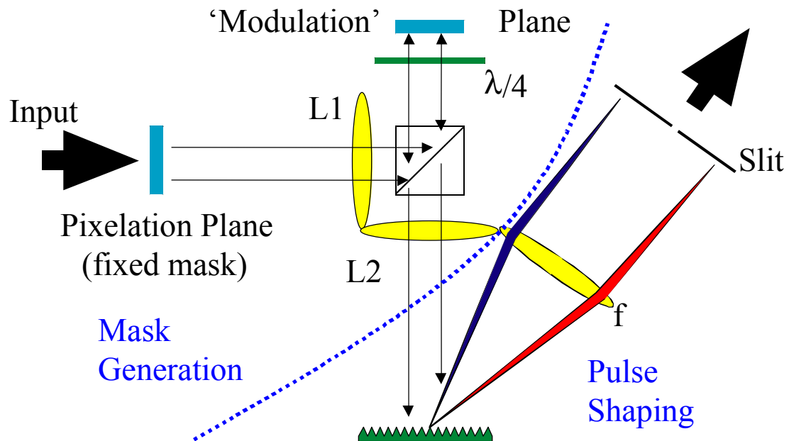
Fig. 3.6. Complete DST pulse shaping apparatus.
