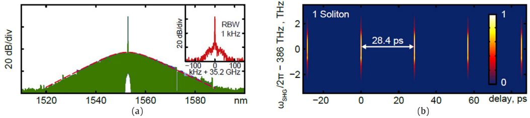
Fig. 28. Soliton generation in a MgF 2 micro-resonator. (a) Shows the optical spectrum of the generated soliton with a characteristic hyperbolic secant shape. The inset is a microwave spectrum of the 35-GHz-repetition-rate, at which the solitons are emitted. (b) Shows a time-domain measurement of the soliton using frequency-resolved optical gating (FROG).
