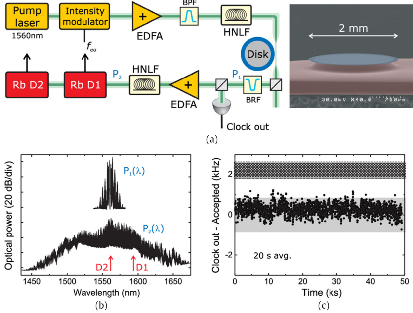
Fig. 46. (a) Schematic, (b) comb spectrum and (c) clock output obtained linking a WGM glass resonator to a rubidium reference. Full stabilisation was achieved with this scheme and the help of additional nonlinear stages. After Ref. [54].
