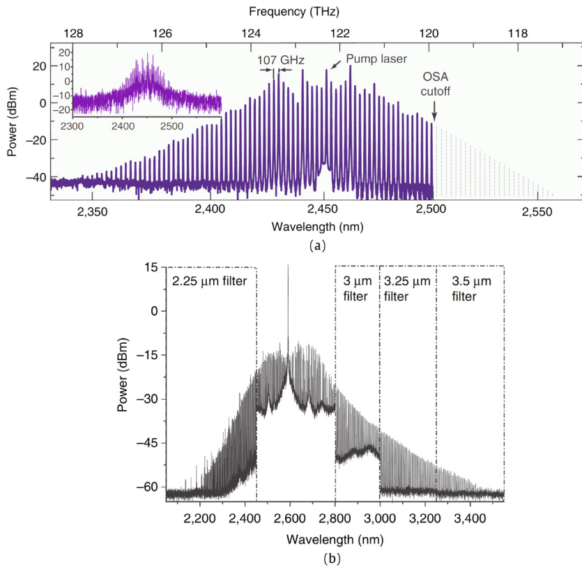
Fig. 47. Mid-infrared micro-comb generation (a) in magnesium fluoride resonators, after Ref. [27] and (b) in an integrated silicon resonator, after Ref. [133].
