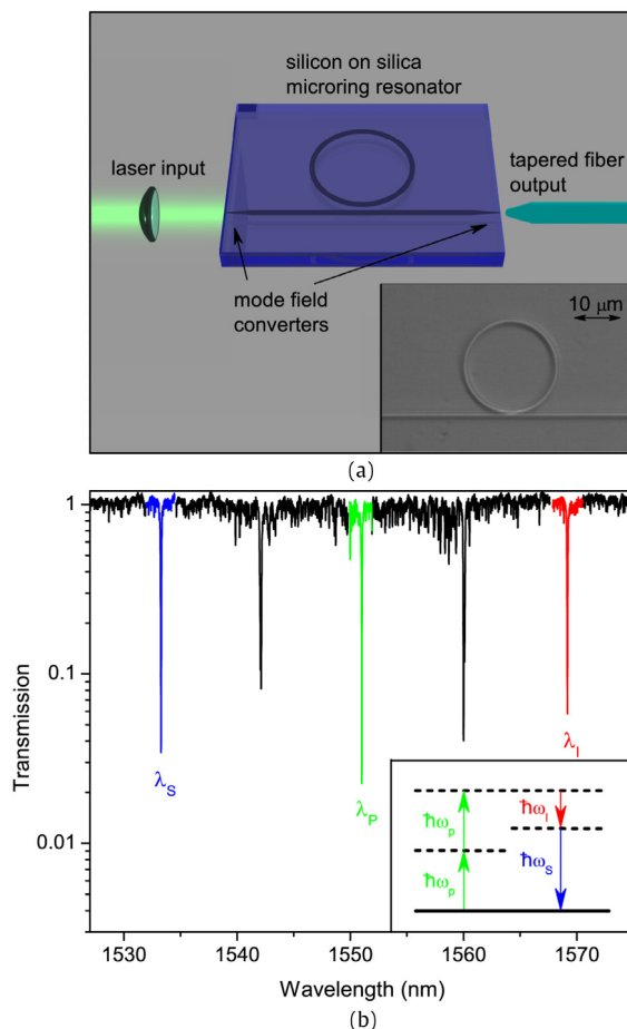
Fig. 55. Ring-resonator device schematic (top) and transmission spectrum (bottom). The 2-port ring-resonator had a radius of 10 \mu\text{m} , a FSR of 9 \text{ nm} and a Q -factor of 15,000 . The nanowire waveguides had transverse dimensions of 500 \text{ nm} (width) and 220 \text{ nm} (height) on SOI. The pump resonance is highlighted in green and the signal and idler resonances employed in the experiment are indicated in blue and red, respectively. After Ref. [326].
