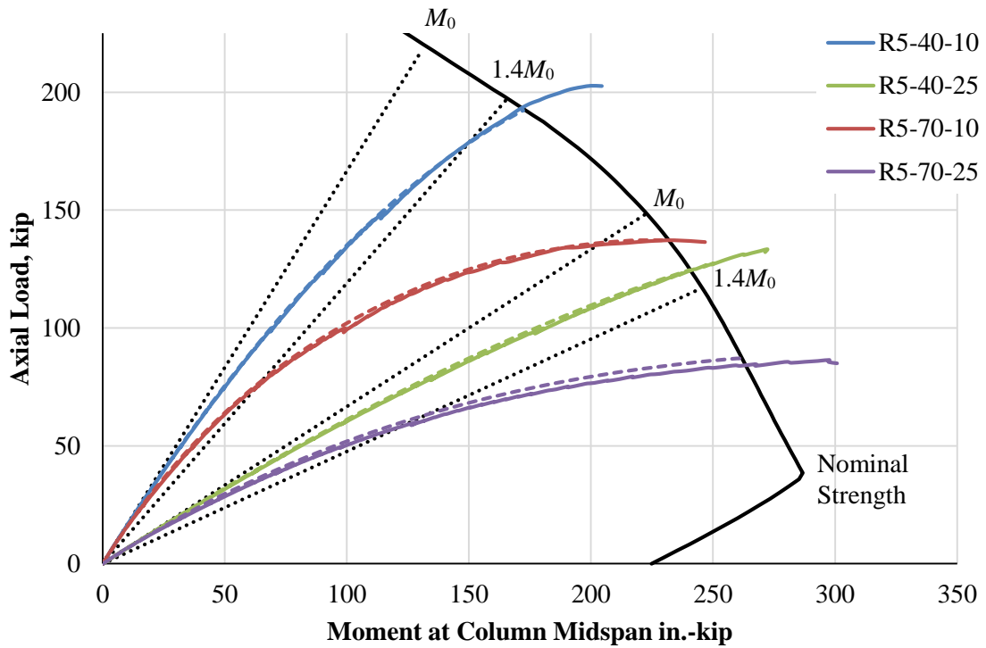
Figure 4.2 – Short-Term Tests Results (#5 bars)
