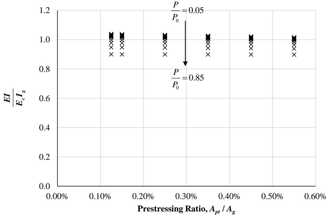
Figure 6.3 – Influence of Prestressing Ratio
