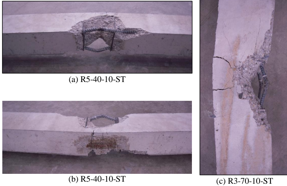
Figure 4.3 – Bar Buckling Failure of Short-Term Tests (Nonprestressed)
