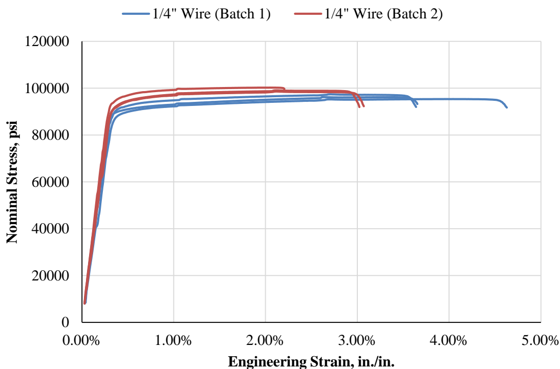
Figure 3.10 – Wire for Column Ties Tests Results
