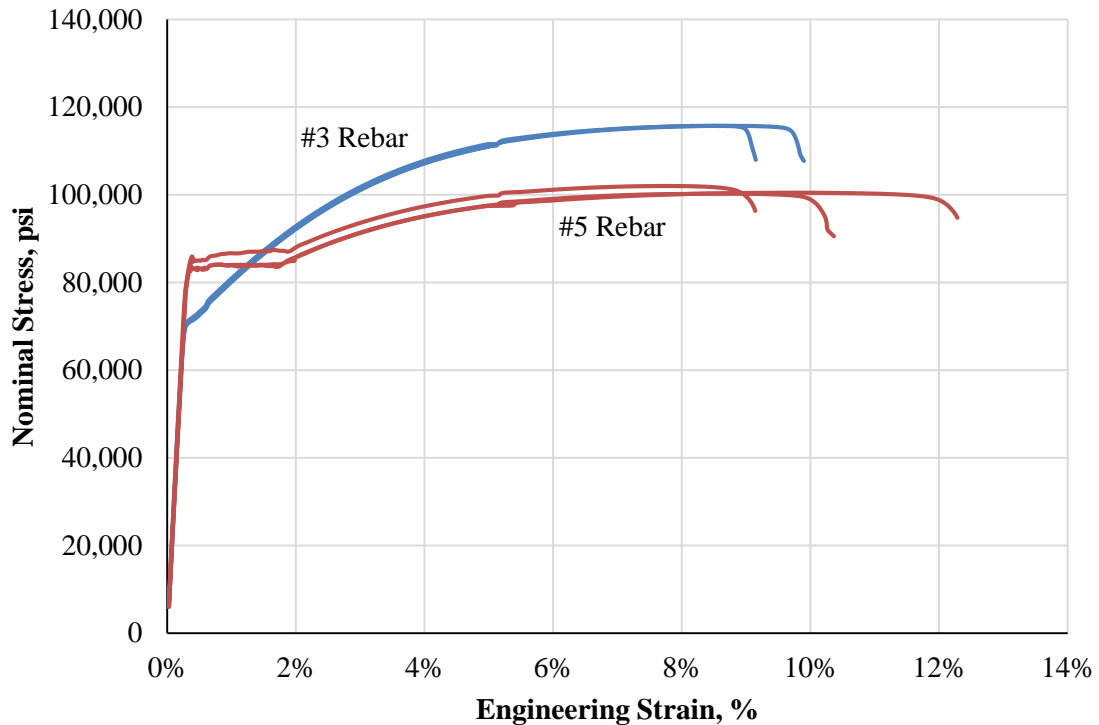
Figure 3.8 – Steel Reinforcing Bar Tests Results
