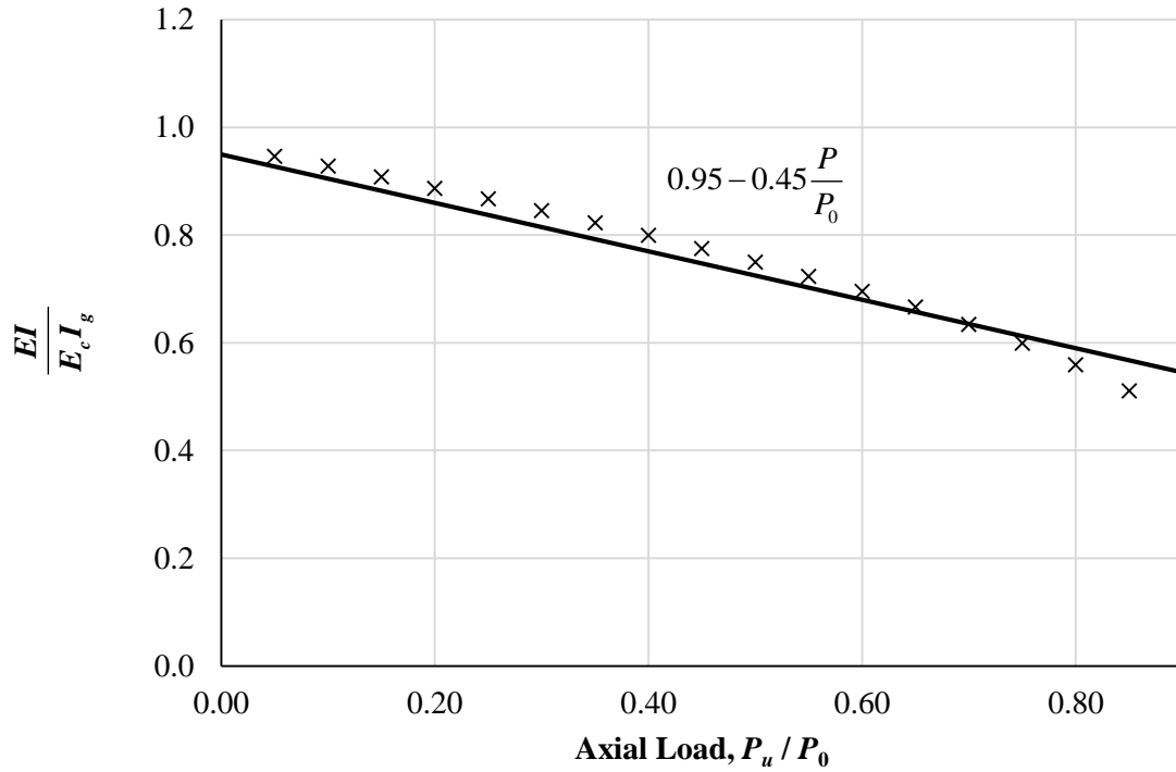
Figure 6.1 – Influence of Varying Axial Load
