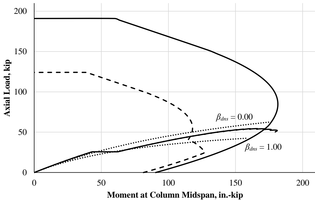
(a) Equation 6.6
