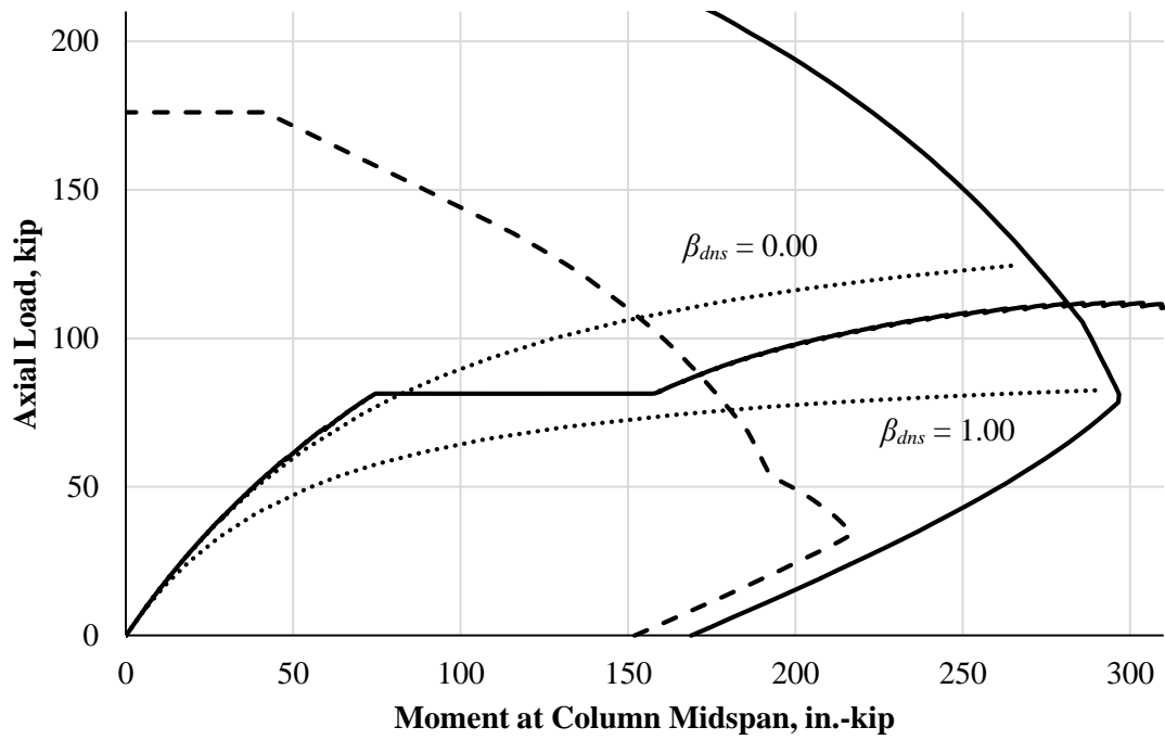
(a) Equation 4.5
