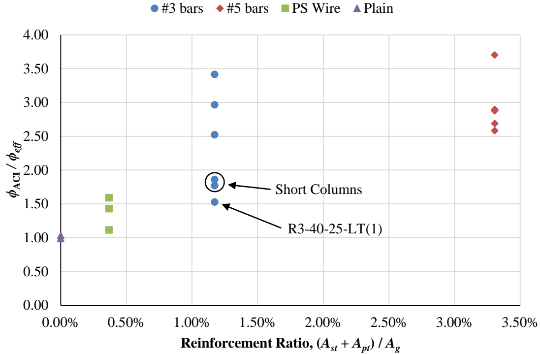
Figure 9.8 – Effective Creep Coefficient versus Reinforcement Ratio
