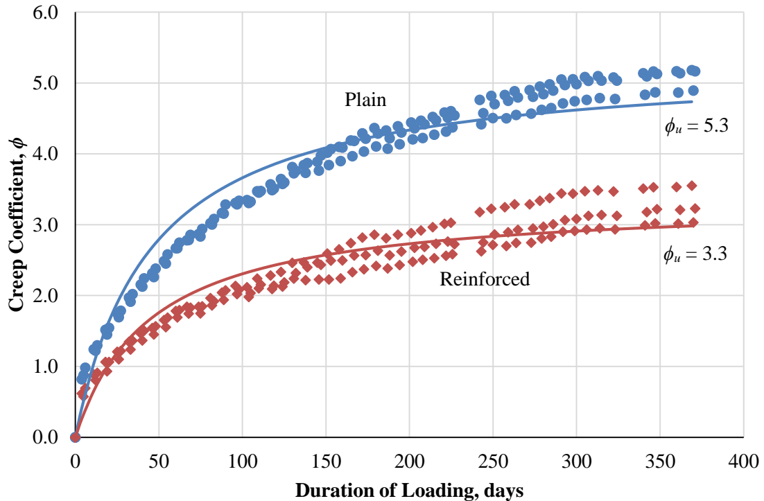
Figure 7.8 – Regression Analysis for Short Column Tests
