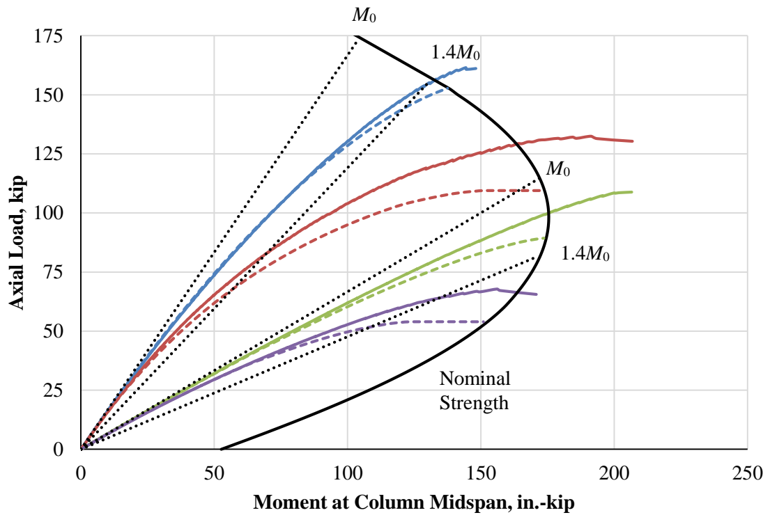
Figure 5.1 – Short-Term Tests Results (2 – PS Wires)
