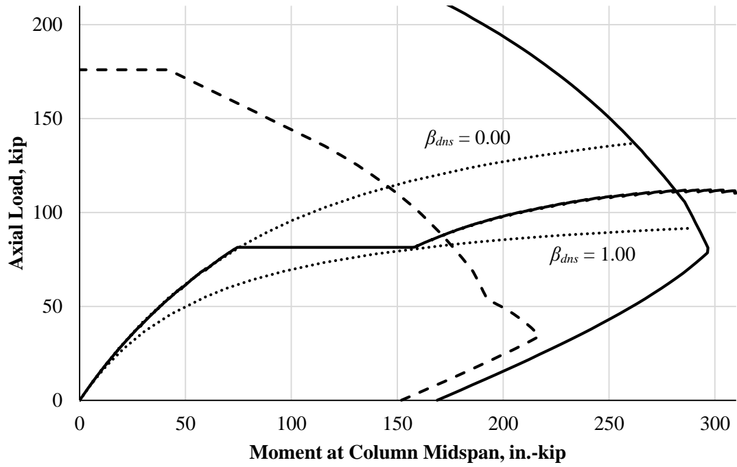
(a) Equation 4.4
