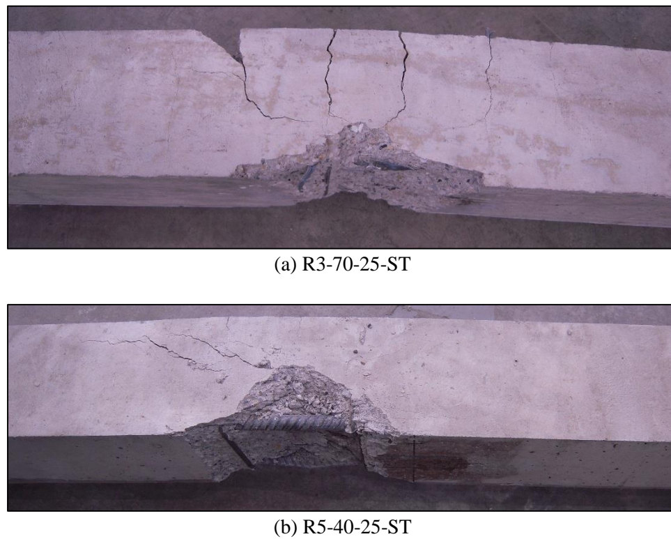
Figure 4.4 – Stiffness Failure of Short-Term Tests (Nonprestressed)
