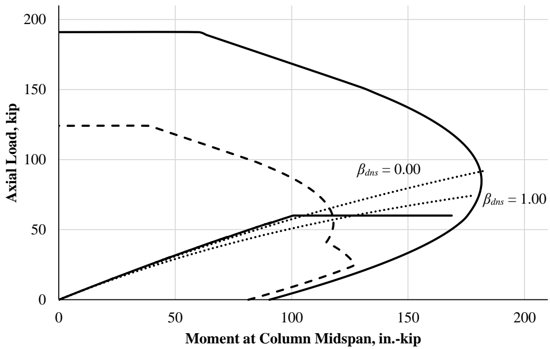
(a) Equation 6.6
