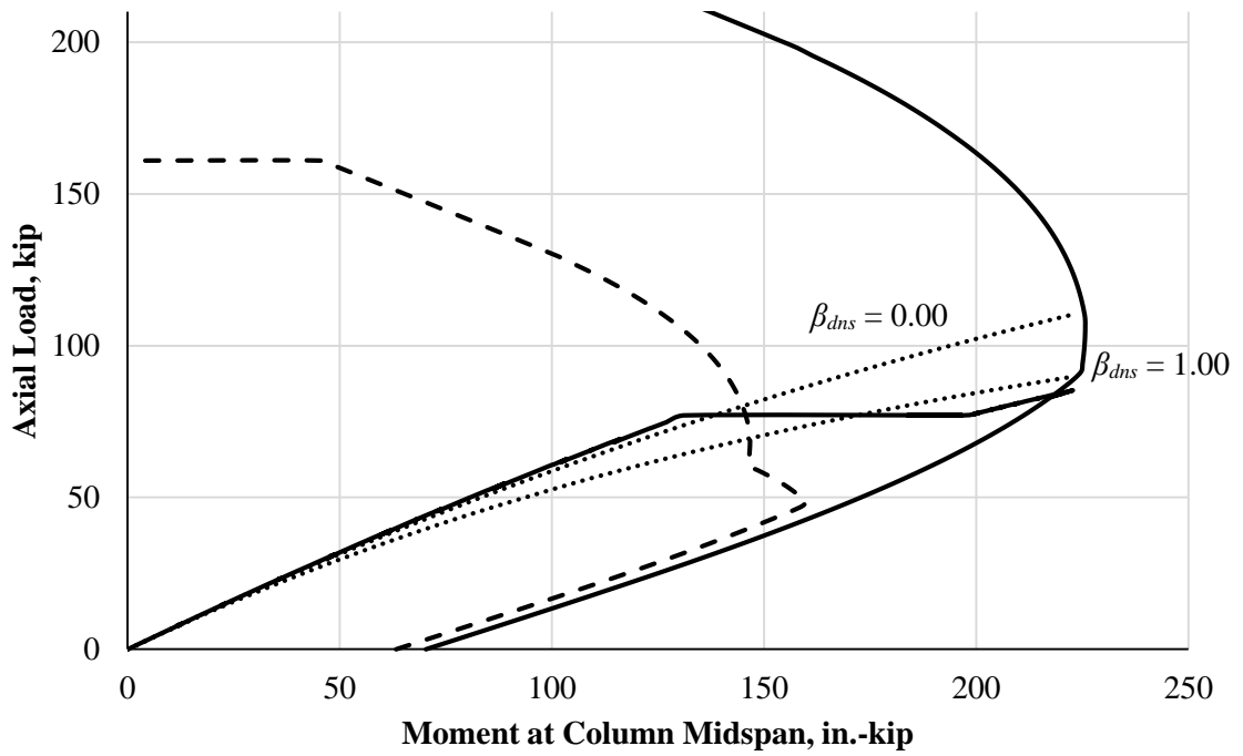
(a) Equation 4.5
