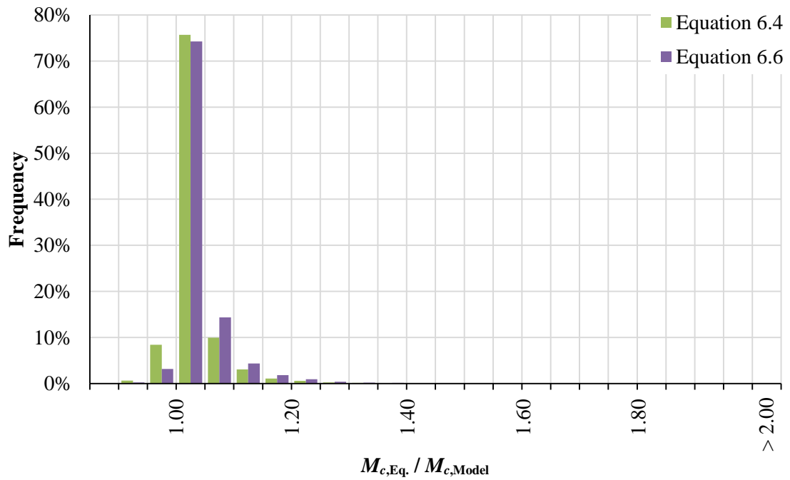
Figure 6.10 – Evaluation of Short-Term Design Equations (Computational Model)
