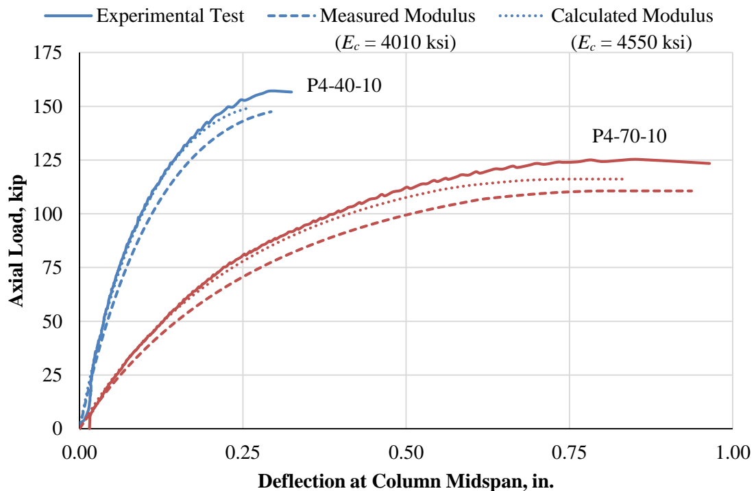
Figure 5.5 – Effect of Modulus of Concrete on Computed Behavior (Prestressed)
