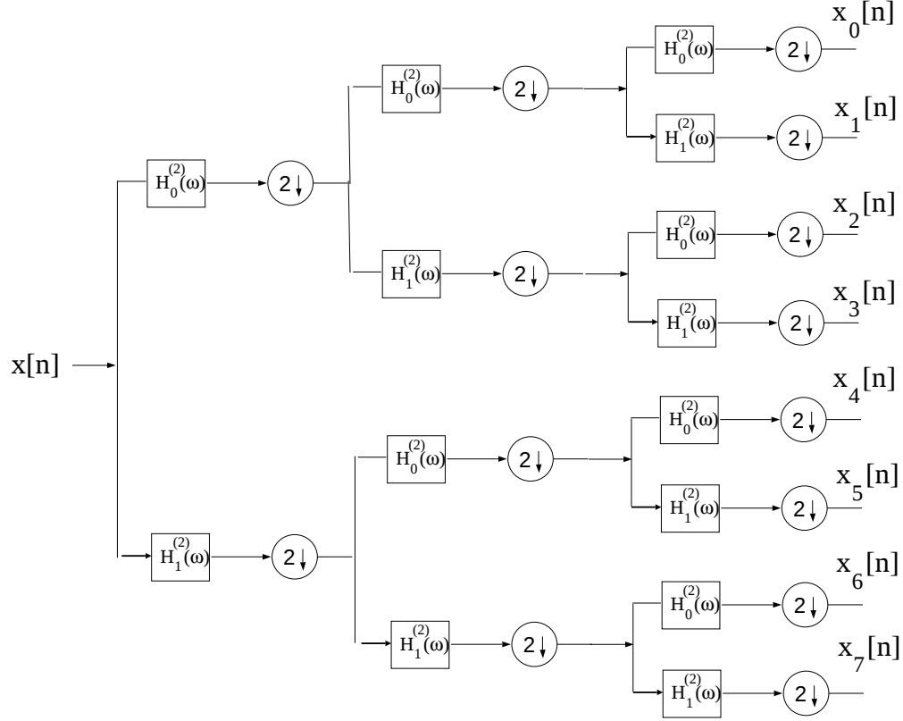
Figure 2(a). Analysis Section of Three-Stage Tree-Structured Filter Bank.
