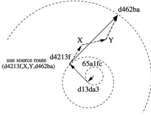
Fig. 3. DPSR routing in MANETs.
