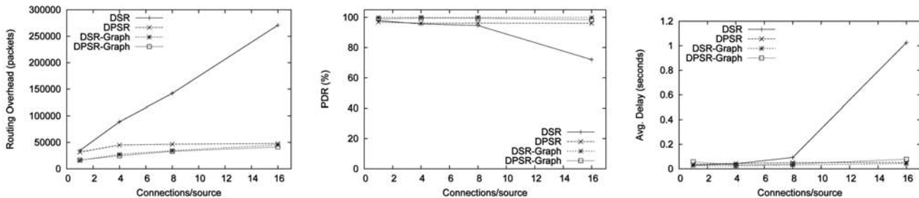
Fig. 8. Routing overhead, PDR, and delay comparison of DPSR and DSR varying the number of data connections for high mobility (pause time 0s).
