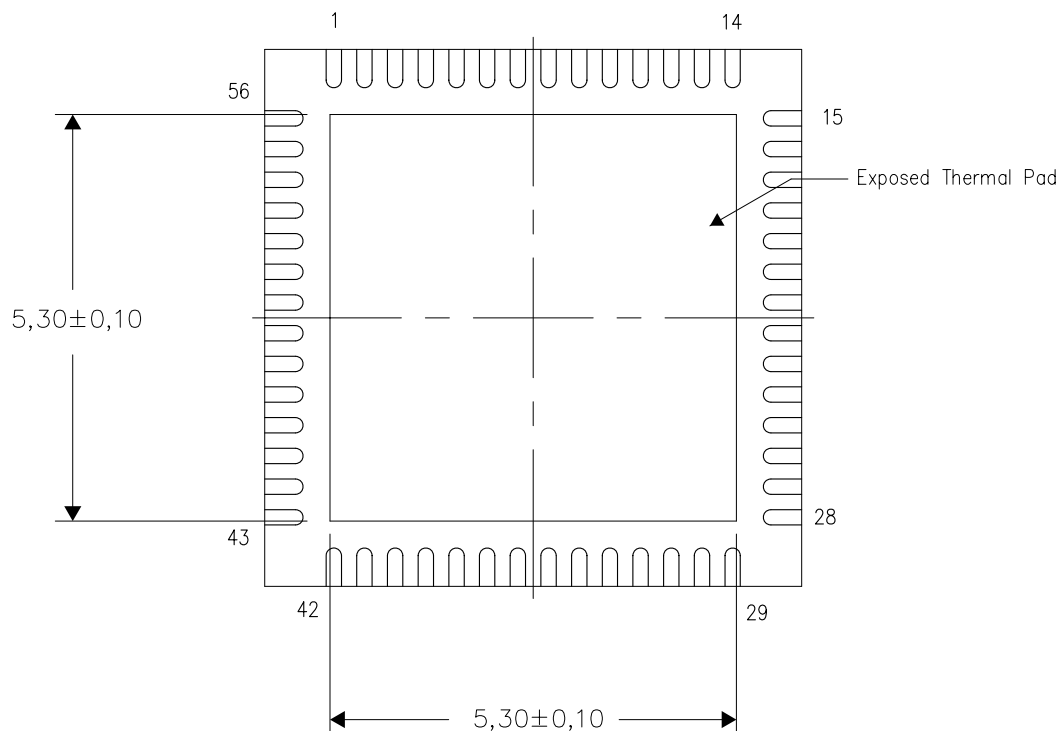
Bottom View
