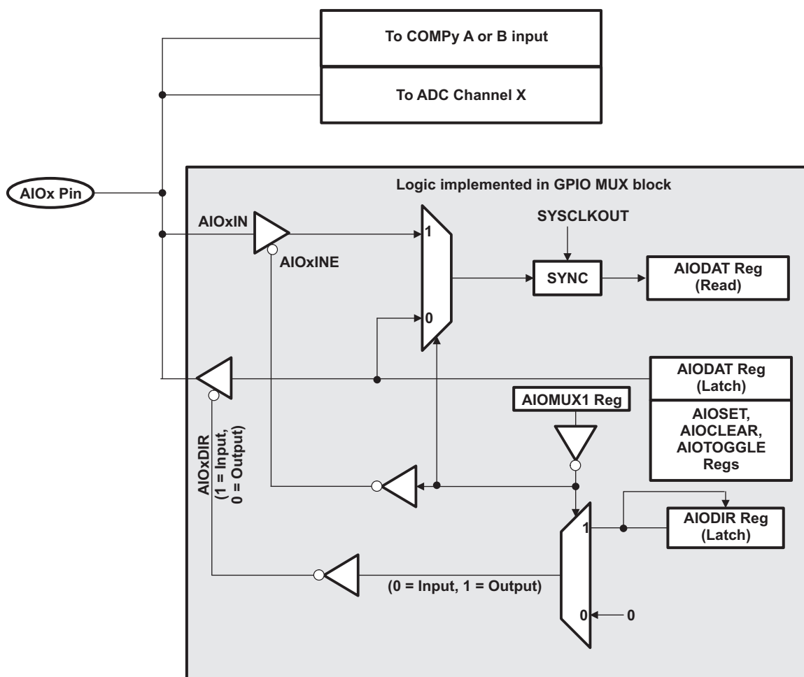
Figure 48. Analog/GPIO Multiplexing
