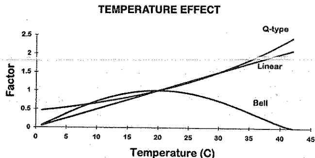
Figure 4—Temperature adjustment factors for maximum specific growth, recycling and senescence. z = 1.33 for bell function, n = 10, Q 10 = 1.5, for Q-type distribution, and minimum, optimum, and maximum temperatures were 0, 20, and 42, respectively.
