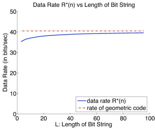
Fig. 5. R^*(n) for \Delta = 50 ms, \delta = 10 ms.
