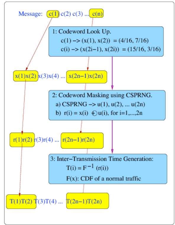
Fig. 9. Non-Detectable Scheme (Sender)
