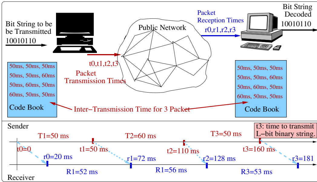
Fig. 1. High Level Design Diagram of Covert Timing Channel
