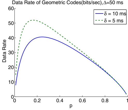
Fig. 3. R(p) for geometric codes.
