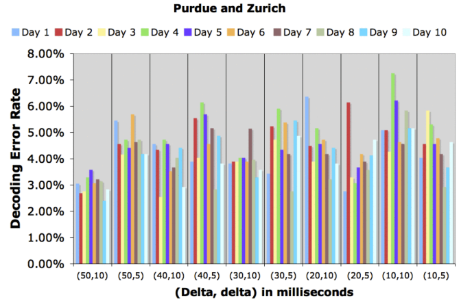
Fig. 7. Daily decoding errors for the covert channel between Purdue and Zurich
