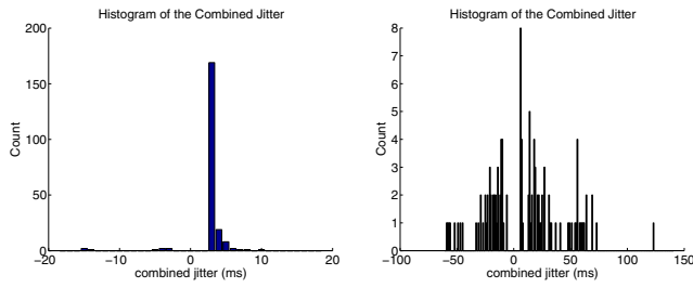
(a) Normal (Excluding |R_i - T_i| < 3 ) (b) Busy (Excluding |R_i - T_i| < 5 )
