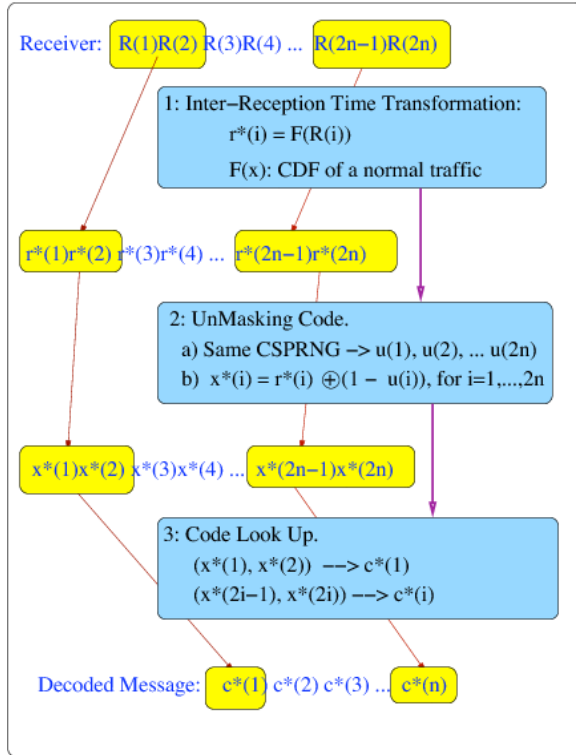
Fig. 10. Message Recovery (Receiver)
