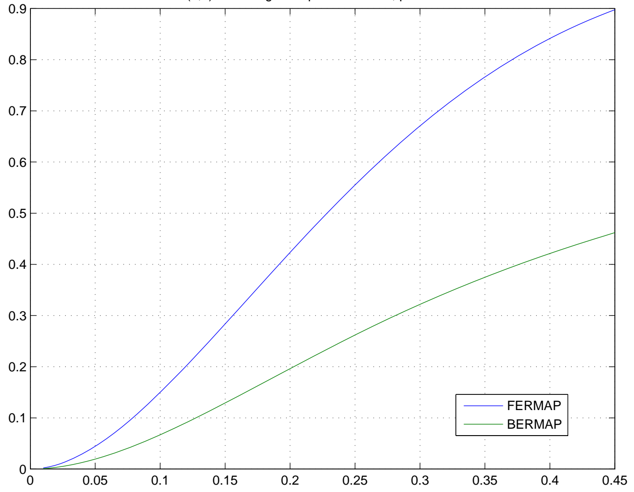
(7,4) Hamming code performance 2, p^*=0.0876
