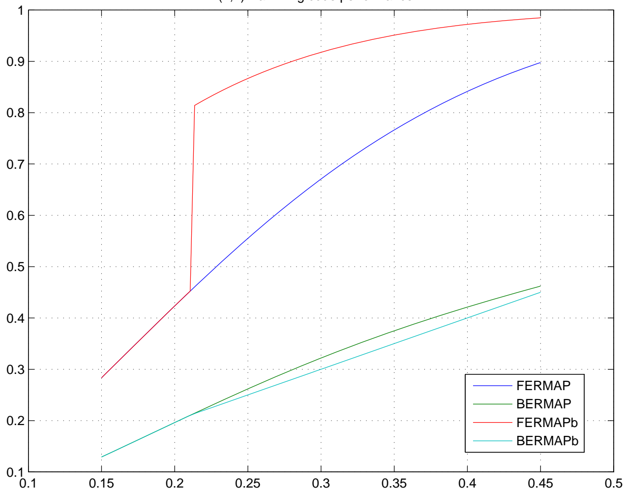
(7,4) Hamming code performance 1
