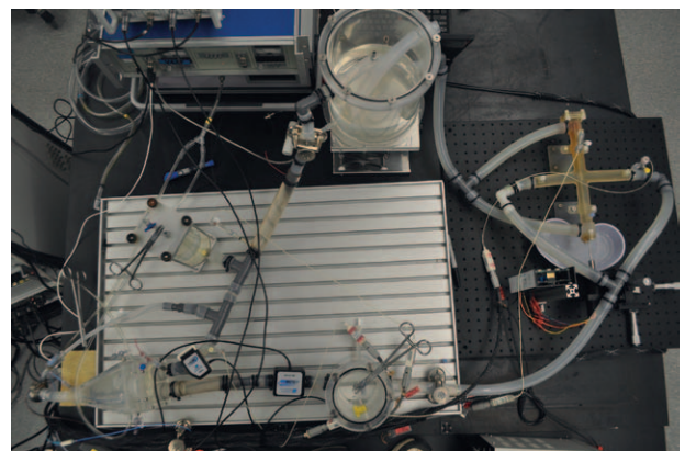
Figure 1. Pediatric Fontan mock circulatory system with: 1) single ventricle, 2) aorta, 3) arterial compliance, 4) systemic vascular resistance, 5) venous compliance, 6) Fontan junction with cavopulmonary assist device (VIP), 7) pulmonary resistance, 8) pulmonary compliance, and 9) ventricular assist device.
