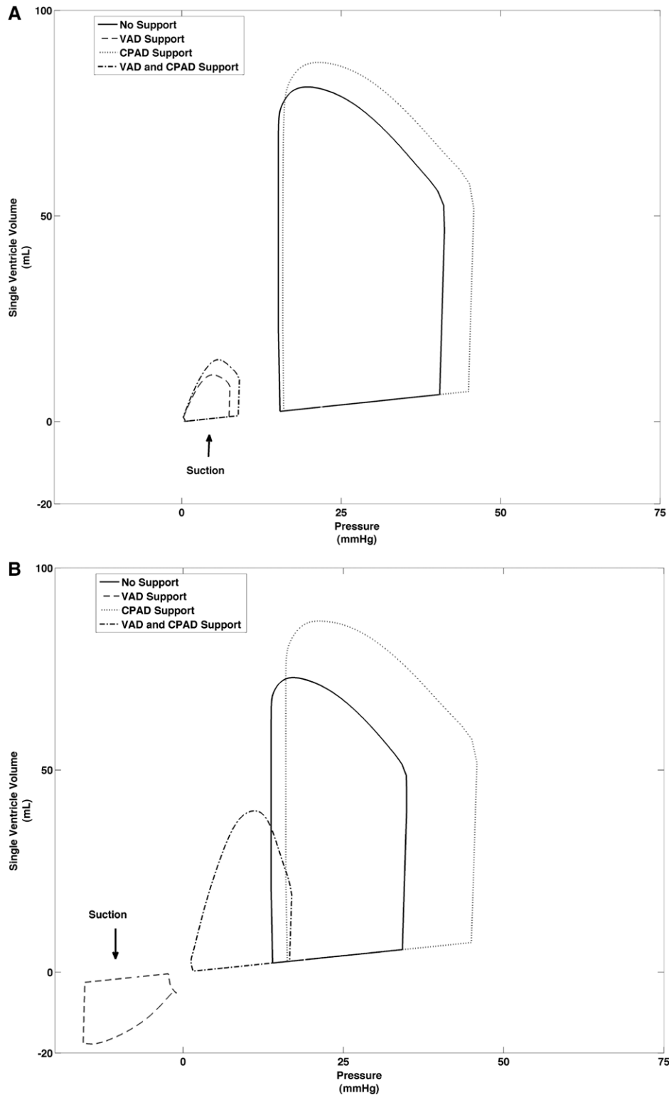
Figure 3. (Continued.) Single ventricular pressure–volumes loops during no support, full ventricular assist device (VAD) support, full cavopulmonary assist device (CPAD) support, and full VAD and CPAD support conditions in Fontan circulations with (A) normal pulmonary resistance (NPR), (B) diastolic dysfunction with elevated pulmonary resistance (right/pulmonic side failure [RSF]), (C) systolic dysfunction (left/systemic side failure [LSF]), and (D) combined systolic and diastolic dysfunction (left and right side failure [LRSF]).
