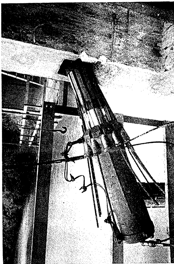
Fig. 21. The hydraulic jack, shown here pulling draped tendons in the web wall, tensioned twelve 1/2-in. (13 mm) diameter 270K strands and had a piston to seat the anchorage cone.
