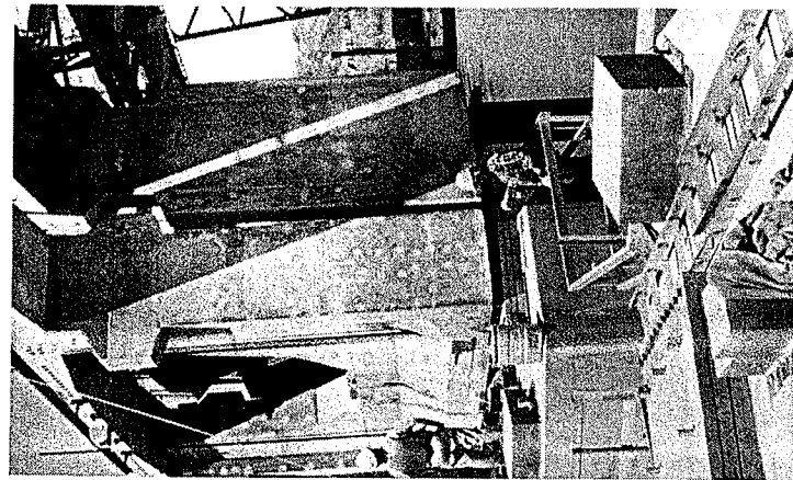
Fig. 19. The first segment was placed May 1, 1979. Note the vertical tie down rod on the side away from the second segment. The concrete risers (with the flat jacks) support the structure until the load is transferred to the pot bearings which are already in place.
