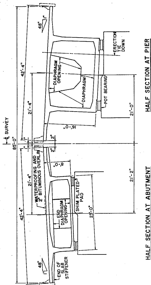
Fig. 2. Cross section of superstructure. (Note: 1 ft = 0.305 m; 1 in. = 25.4 mm.)
