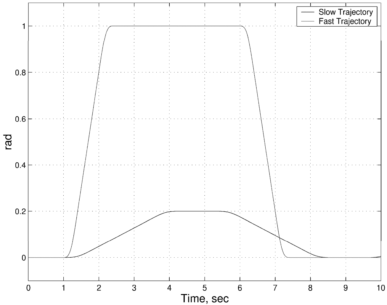
Desired Point-to-Point Trajectory
