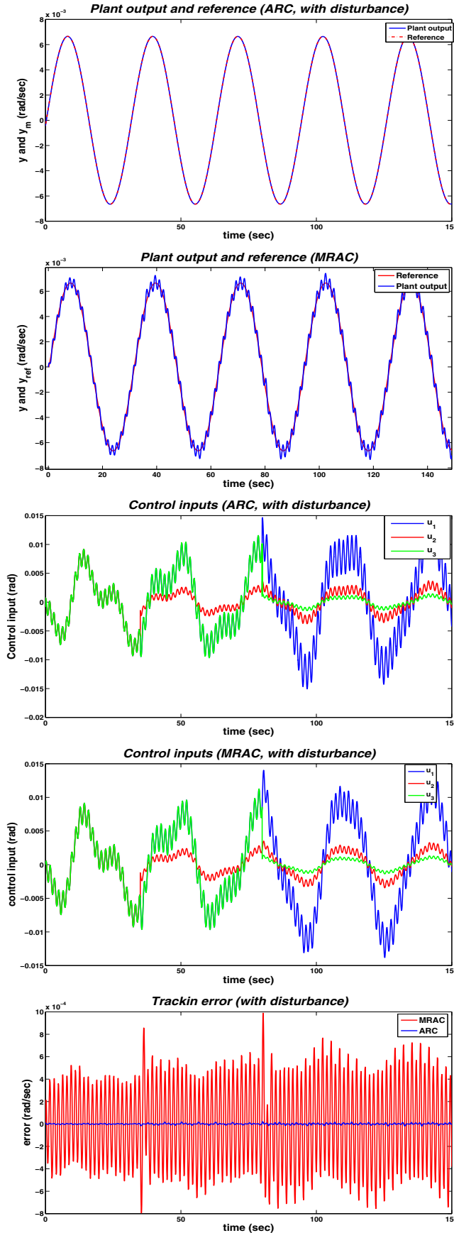
Fig. 2. System response, tracking error and control effort with disturbance.
