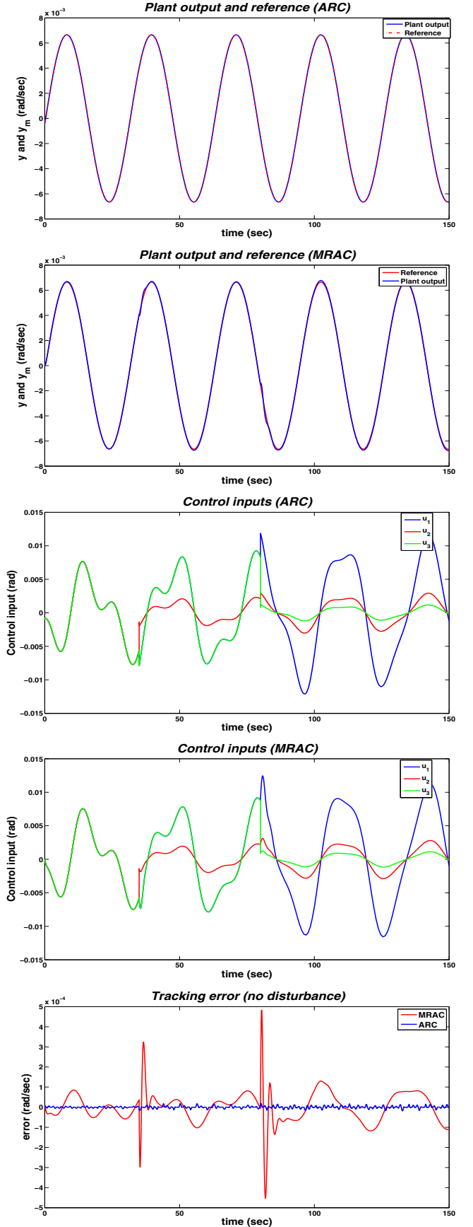
Fig. 1. System response, tracking error and control effort without disturbance.
