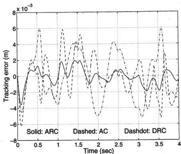
Fig. 4 Motion tracking errors in the presence of parametric uncertainties and large disturbances
