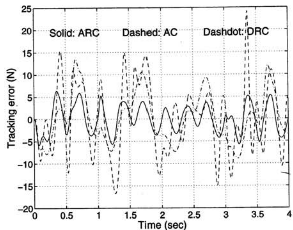
Fig. 5 Force tracking errors in the presence of parametric uncertainties and large disturbances
