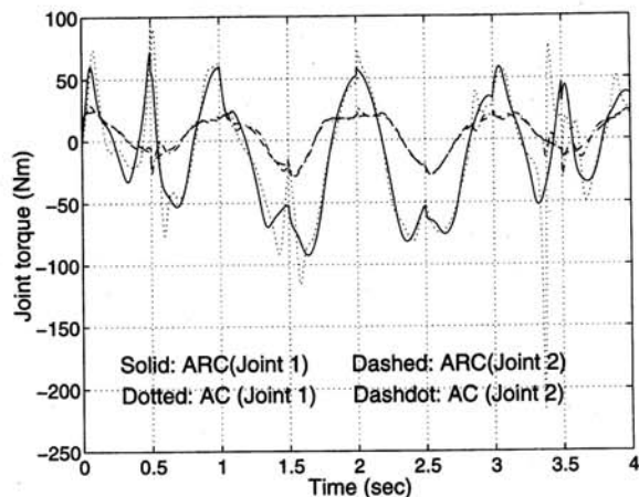
Fig. 6 Control inputs in the presence of parametric uncertainties and large disturbances
