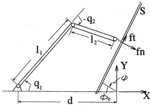
Fig. 1 Configuration of the robot
