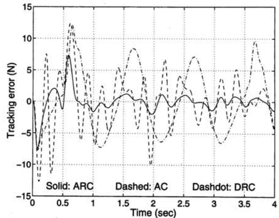
Fig. 3 Force tracking errors in the presence of parametric uncertainties
