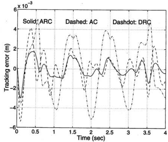
Fig. 2 Motion tracking errors in the presence of parametric uncertainties
