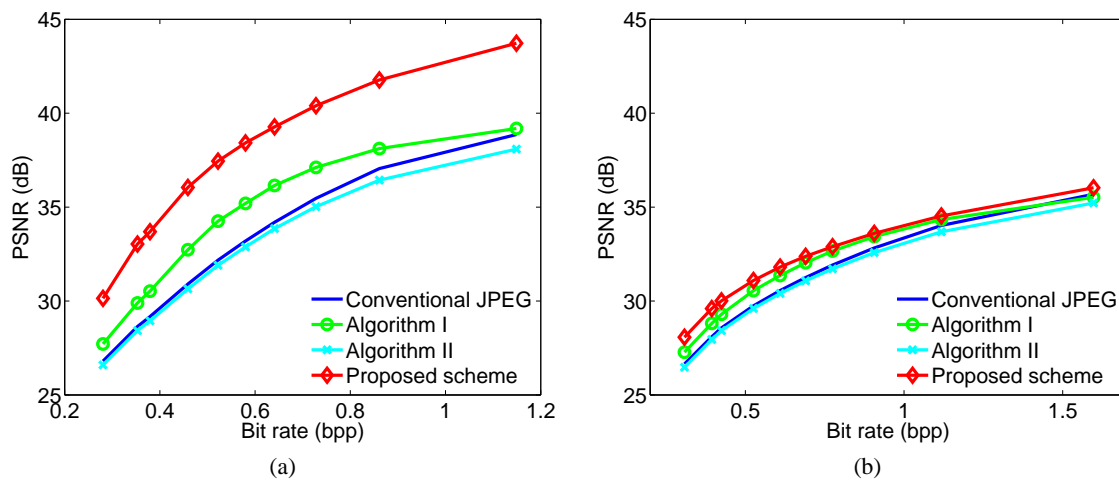
Fig. 19. Average PSNR versus average bit rate computed for 30 digital images in (a), and another 30 scanned images in (b).
