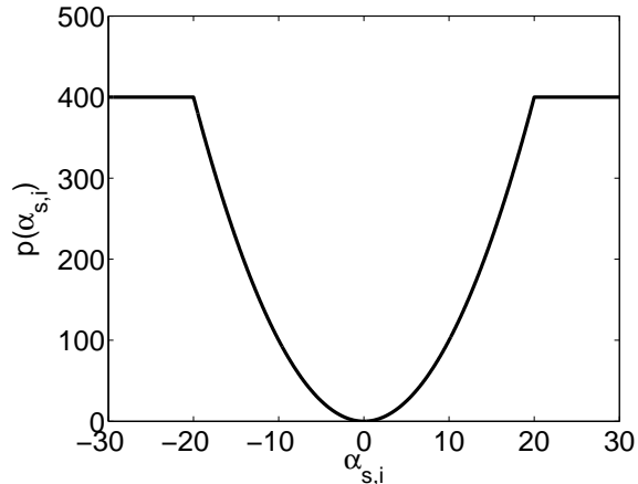
Fig. 3. The potential function \rho(x) = \min(x^2, \tau^2) , \tau = 20 , of the Markov random fields used to characterize the spatial variation of the predominant colors C_{1,s} and C_{2,s} . The threshold parameter \tau ensures that we avoid excessively penalizing large intensity difference between the two corresponding predominant colors of two neighboring blocks.
