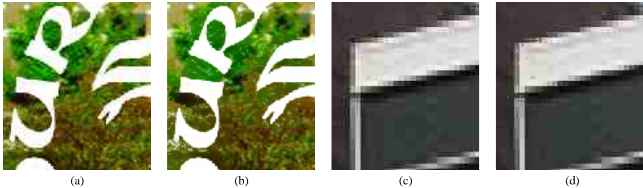
Fig. 18. Robustness of the proposed algorithm. (a), (b) Image patch where text blocks contain non-uniform background: (a) conventional JPEG decoder, (b) the proposed algorithm. (c), (d) Image patch where our segmentation algorithm misclassifies some of the picture blocks as text blocks: (c) conventional JPEG decoder, (d) the proposed algorithm.
