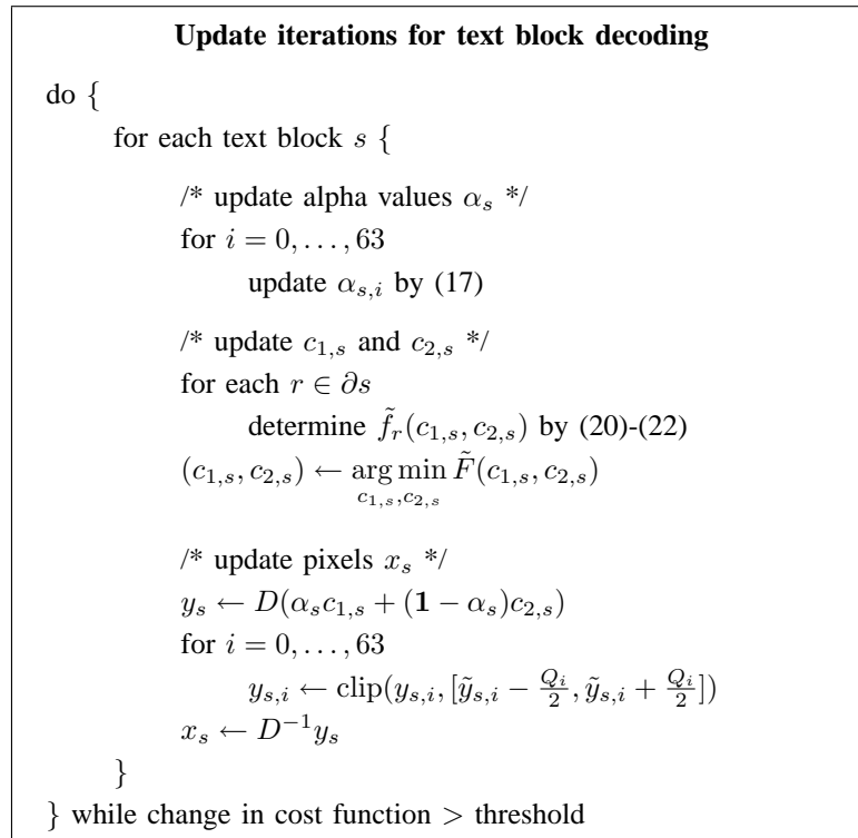
Fig. 4. Pseudo-code of the update iterations for text block decoding. One full iteration consists of updating every text block once. Each text block s is updated in three steps which minimize the cost with respect to: 1) the alpha values in \alpha_s ; 2) the predominant intensities ( c_{1,s}, c_{2,s} ); and 3) the pixel intensities in x_s .
