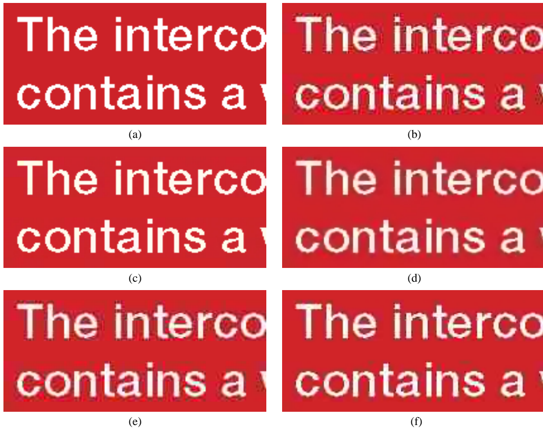
Fig. 12. A text region from Image 1. (a) Original. (b) Conventional JPEG decoding. (c) The proposed algorithm. (d) Algorithm I [11]. (e) Algorithm II [34]. (f) Algorithm III [3].
