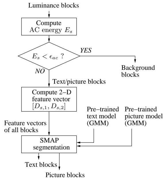
Fig. 5. Block-based segmentation. The background blocks are first identified by AC energy thresholding. A 2-D feature vector is then computed for each block. Two Gaussian mixture models are obtained from supervised training: one for the text class and one for the picture class. With these two models, the feature vector image is segmented using the SMAP segmentation algorithm. The result is combined with the detected background blocks to form the final segmentation map.
