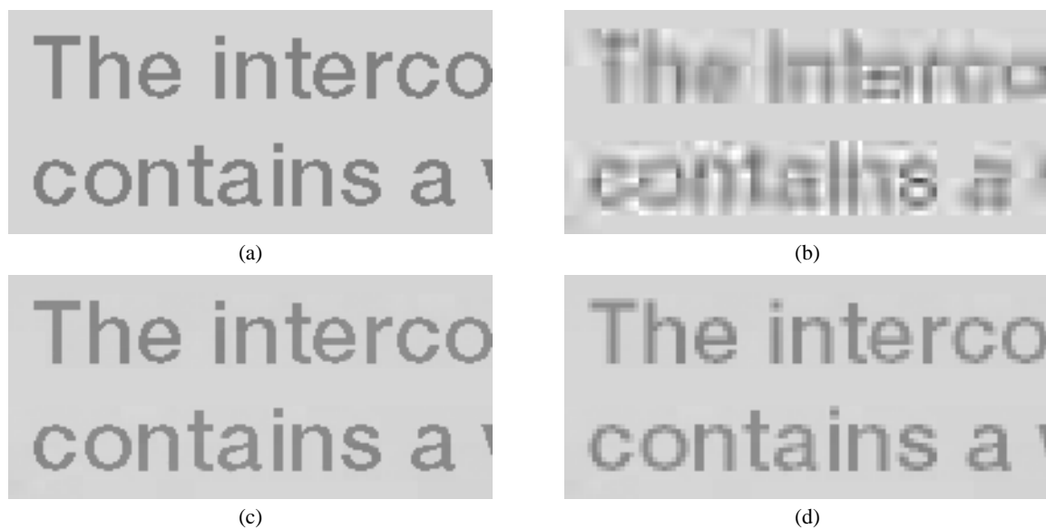
Fig. 11. Chrominance component ( C_r ) of the region shown in Fig. 10. (a) Original. (b) Decoded by conventional JPEG decoding and interpolated by pixel replication. (c) Decoded by our scheme. (d) Decoded by our scheme but interpolated by pixel replication.
