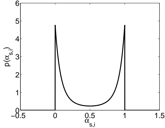
Fig. 2. The marginal probability density function of an alpha value \alpha_{s,i} , for \nu = 12 . As the alpha value controls the proportion of the two intensities C_{1,s} and C_{2,s} present in a text pixel value, the density function's support is [0, 1] . The bimodal nature of the density function with peaks at 0 and 1 models the clustering of the text pixel values around C_{1,s} and C_{2,s} .
