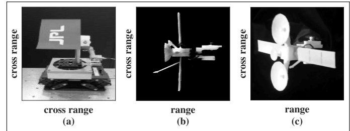
Fig. 3. Targets used for laboratory experiments. (a) JPL logo with range axis into the page. The stencil was placed on a Lambertian reflector angled at 45 degrees. (b) Mock satellite (Orientation 1). (c) Mock satellite (Orientation 2).
