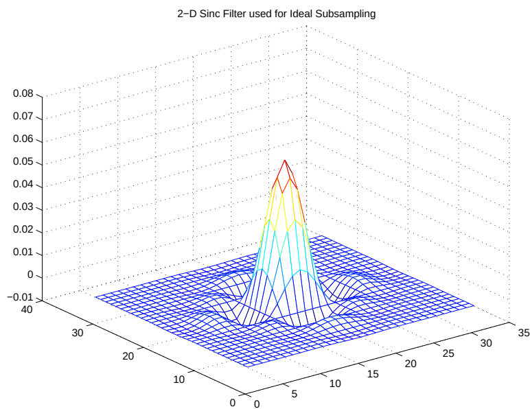
Sinc filter
