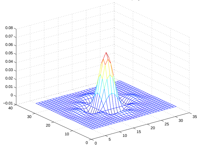
Sinc filter
