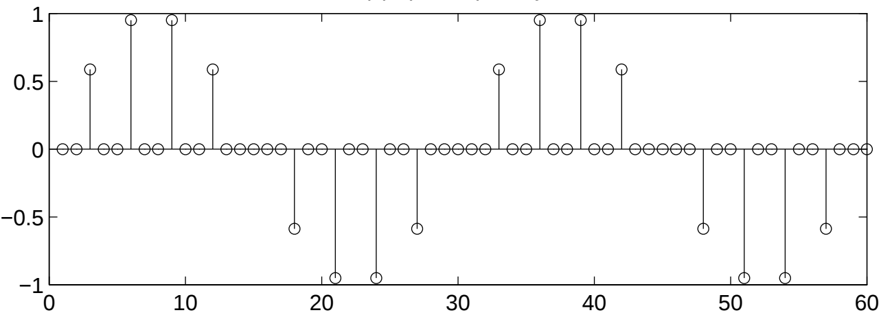
x[n] up-sampled by 3
