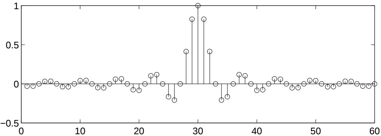
Ideal interpolating filter h(n)
