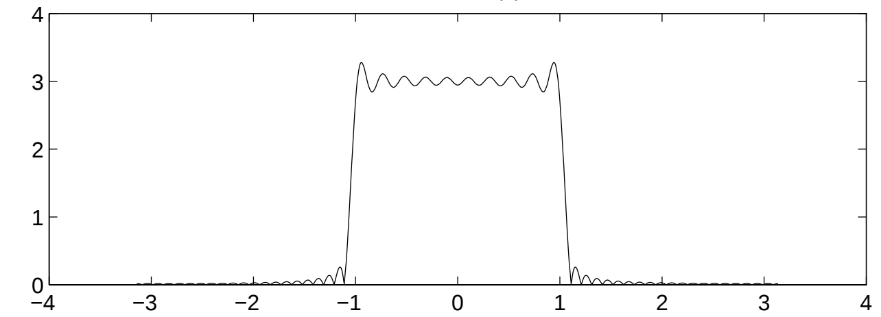
DTFT of H(n)
